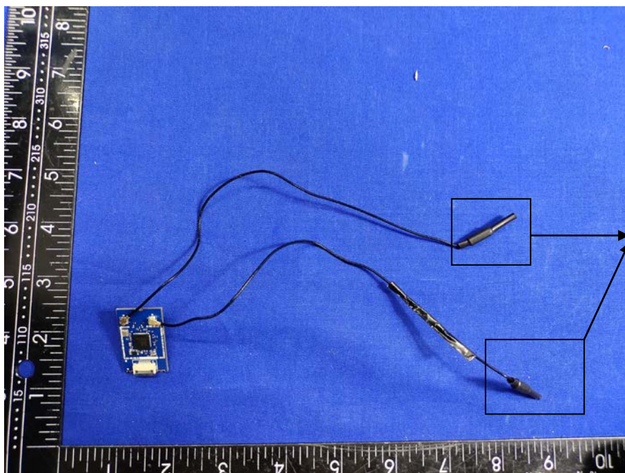
Copper Tube Antenna
