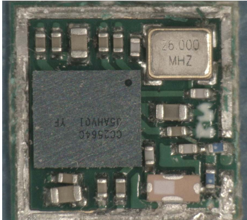
Figure 2 - Front of Module - Inside
