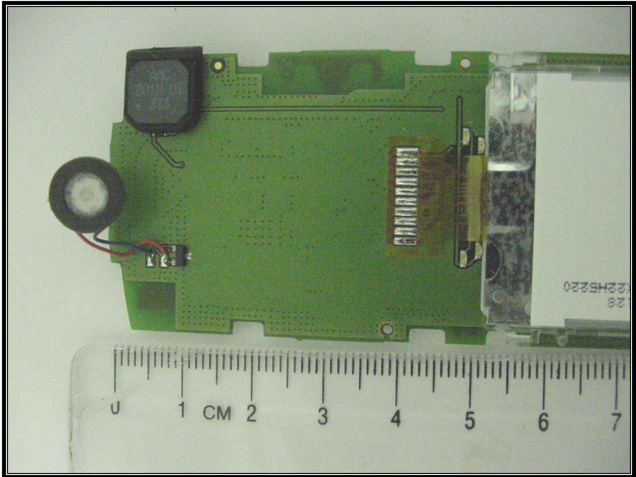
PHOTOGRAPH 16: UNDER LCD ON FRONT OF PCB
