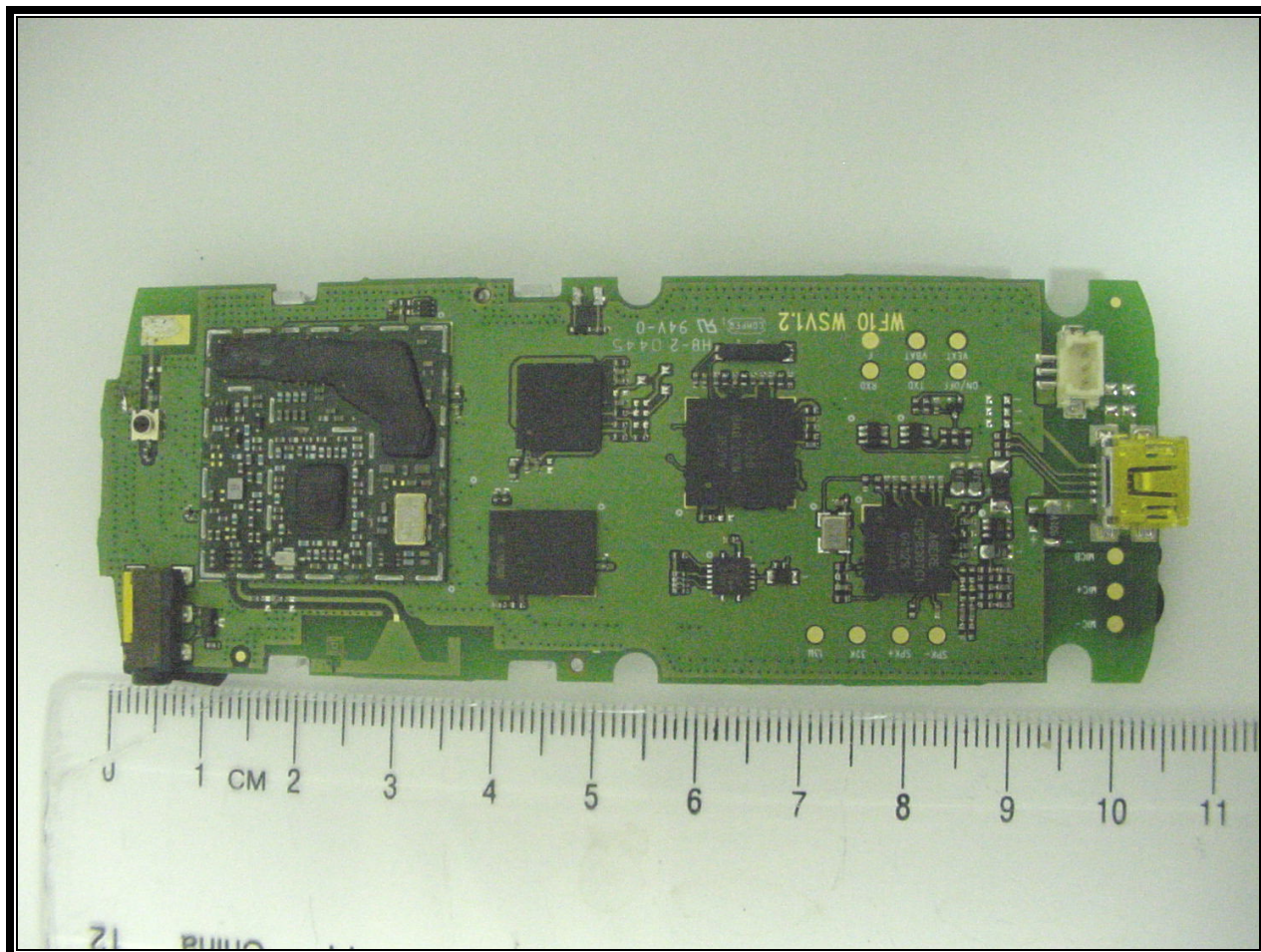
PHOTOGRAPH 15: PCB BACK WITH SHIELD REMOVED
