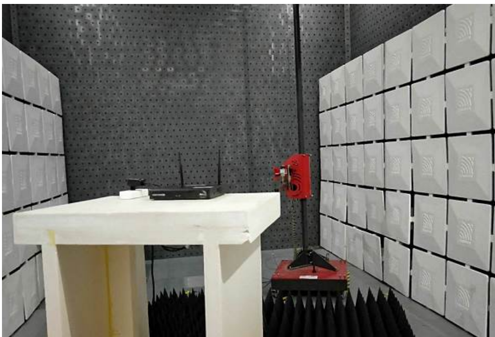
Radiated Emissions, Above 1GHz Test Setup
