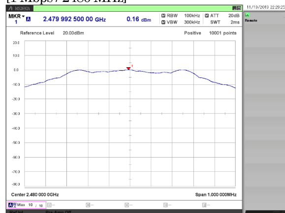
[1 Mbps / 2480 MHz]
