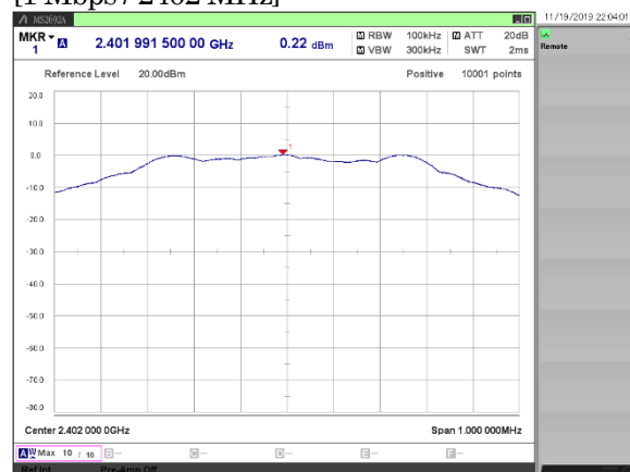
[1 Mbps / 2402 MHz]
