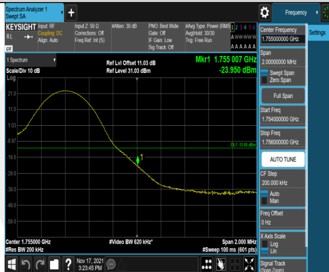
Band4-10MHz-QPSK-20350-1RB#49
