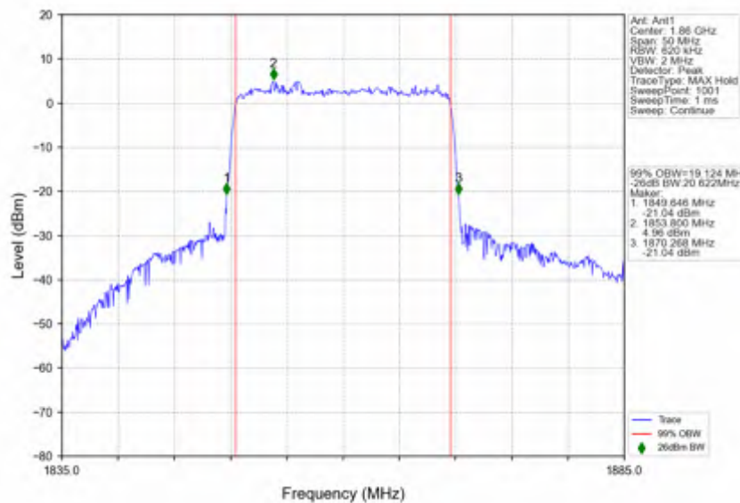
n2_15kHz_SISO_NTNV_20MHz_CP-OFDM_QPSK_1860MHz_Outer_Full
