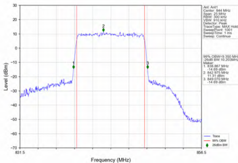
n5_15kHz_SISO_NTNV_10MHz_CP-OFDM 64 QAM_844MHz_Outer_Full
