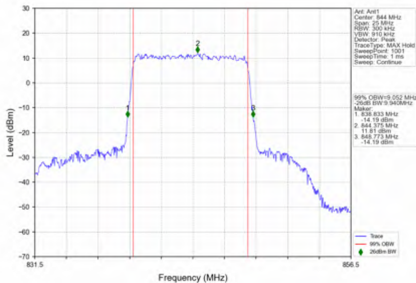
n5_15kHz_SISO_NTNV_10MHz_DFT-s-OFDM 64 QAM_844MHz_Outer_Full
