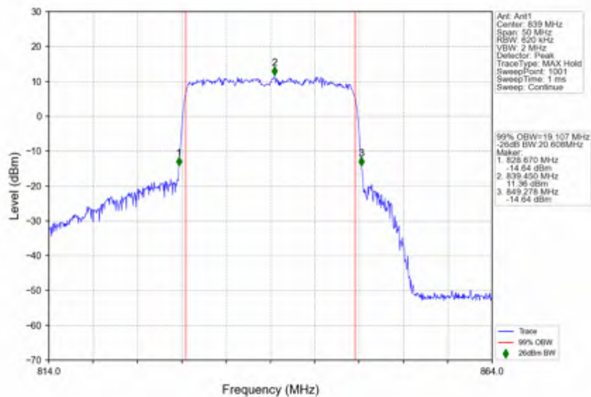
n5_15kHz_SISO_NTNV_20MHz_CP-OFDM_64_QAM_839MHz_Outer_Full
