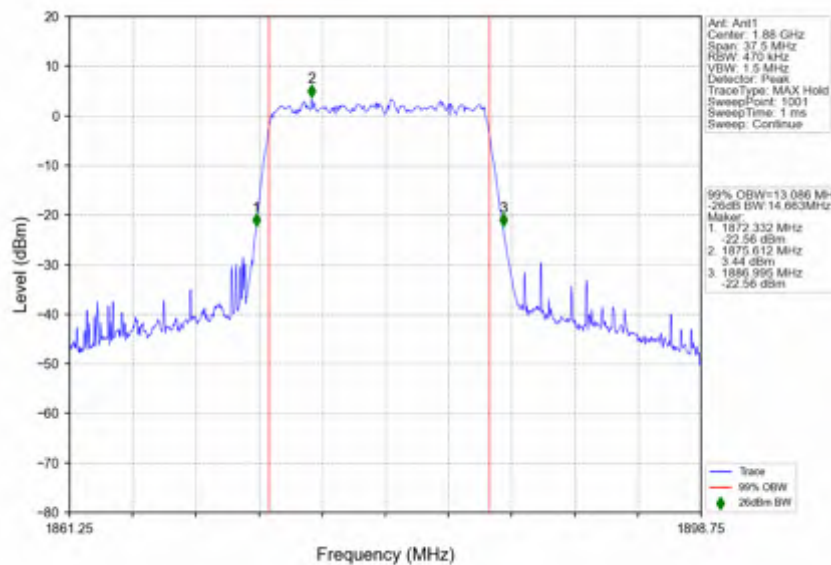
n2_30kHz_SISO_NTNV_15MHz_DFT-s-OFDM 256 QAM_1880MHz_Outer_Full
