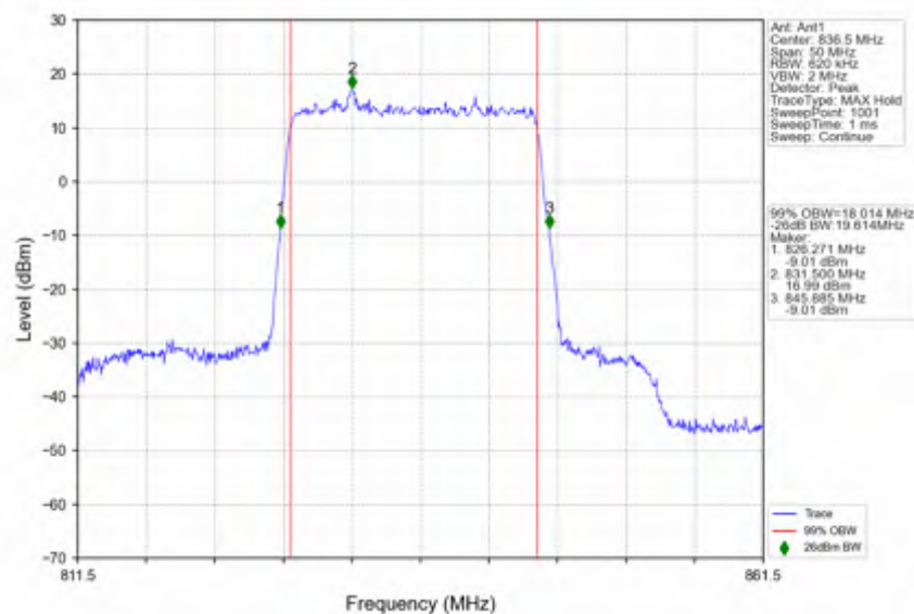
n5_15kHz_SISO_NTNV_20MHz_DFT-s-OFDM_PI/2_BPSK_836.5MHz_Outer_Full
