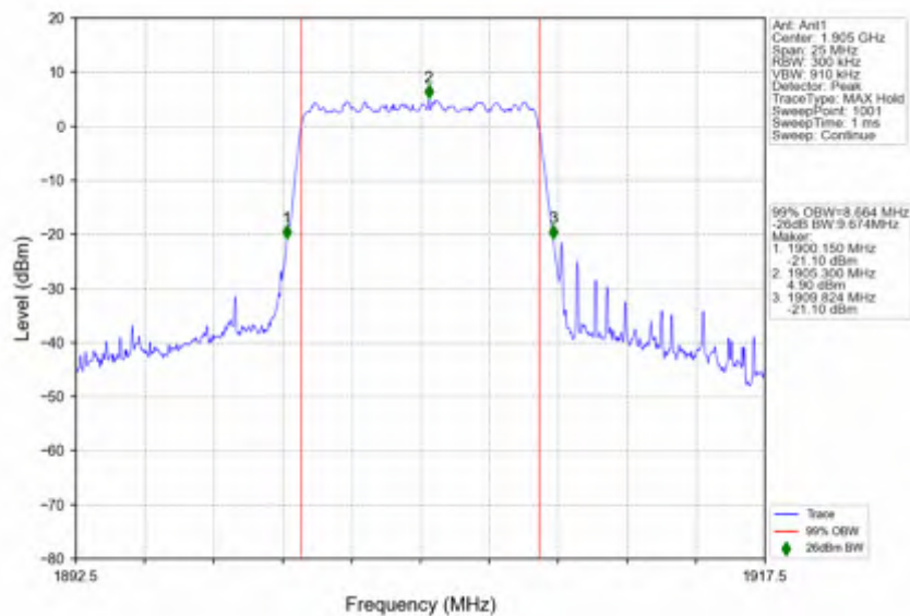
n2_30kHz_SISO_NTNV_10MHz_DFT-s-OFDM 64 QAM_1905MHz_Outer_Full
