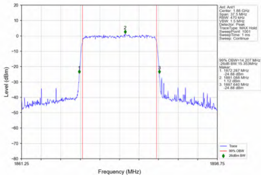
n2_15kHz_SISO_NTNV_15MHz_CP-OFDM_256_QAM_1880MHz_Outer_Full
