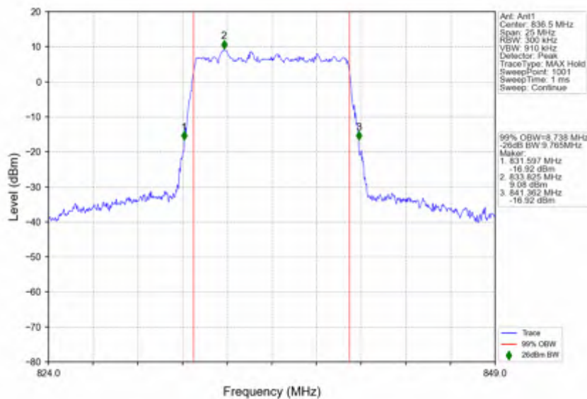
n5_30kHz_SISO_NTNV_10MHz_CP-OFDM 256 QAM_836.5MHz_Outer_Full
