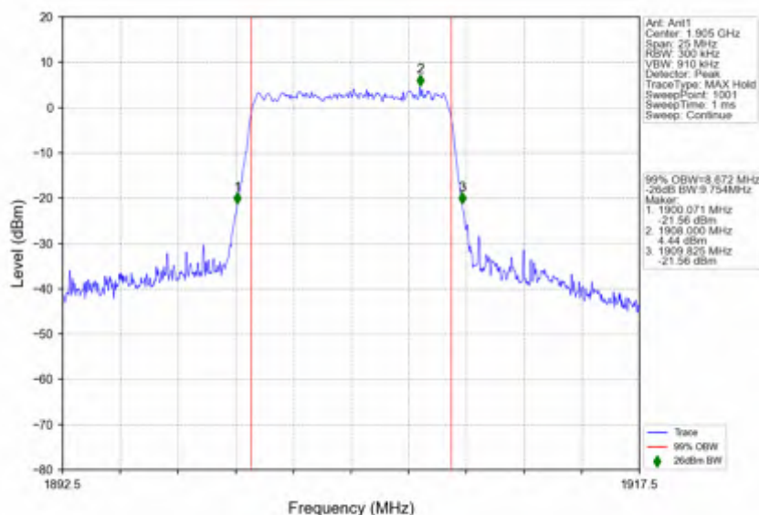
n2_30kHz_SISO_NTNV_10MHz_CP-OFDM 64 QAM_1905MHz_Outer_Full
