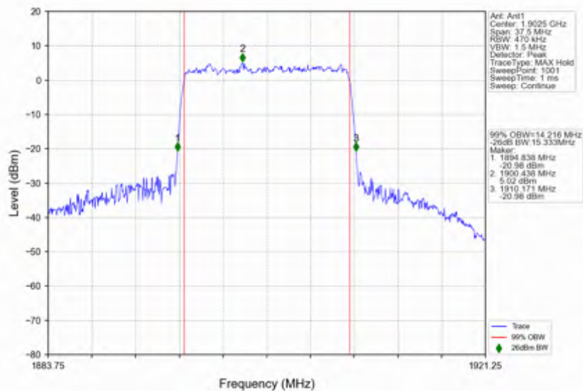
n2_15kHz_SISO_NTNV_15MHz_CP-OFDM QPSK_1902.5MHz_Outer_Full
