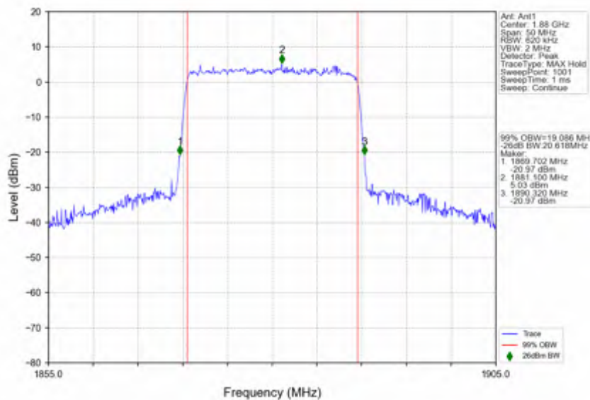
n2_15kHz_SISO_NTNV_20MHz_CP-OFDM_16_QAM_1880MHz_Outer_Full
