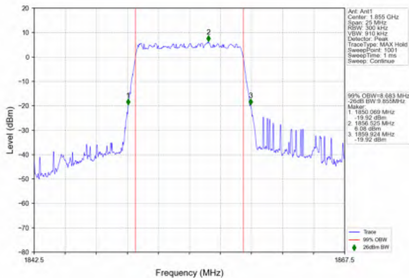
n2_30kHz_SISO_NTNV_10MHz_DFT-s-OFDM QPSK_1855MHz_Outer_Full
