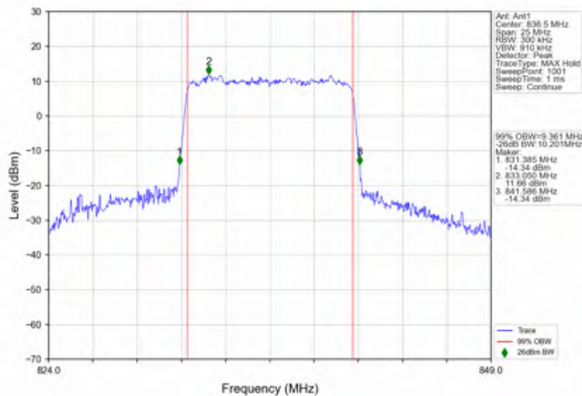
n5_15kHz_SISO_NTNV_10MHz_CP-OFDM_16_QAM_836.5MHz_Outer_Full
