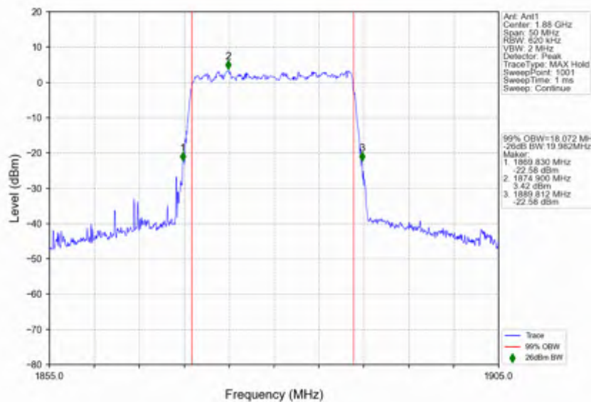
n2_30kHz_SISO_NTNV_20MHz_DFT-s-OFDM_256_QAM_1880MHz_Outer_Full
