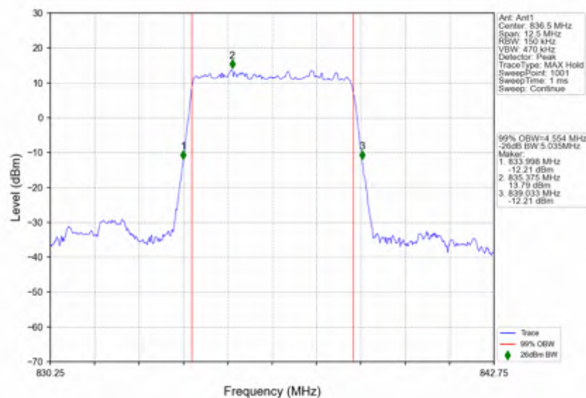
n5_15kHz_SISO_NTNV_5MHz_DFT-s-OFDM_PI/2_BPSK_836.5MHz_Outer_Full
