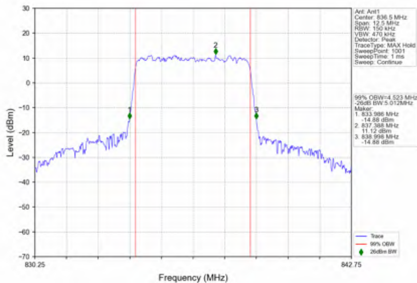
n5_15kHz_SISO_NTNV_5MHz_CP-OFDM_16_QAM_836.5MHz_Outer_Full
