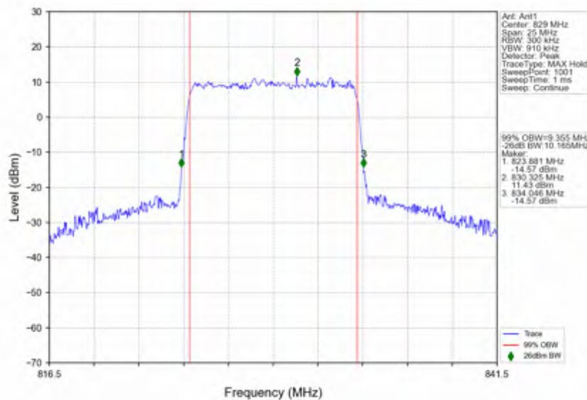
n5_15kHz_SISO_NTNV_10MHz_CP-OFDM 64 QAM_829MHz_Outer_Full
