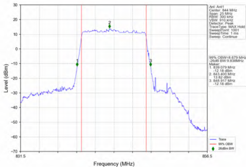
n5_30kHz_SISO_NTNV_10MHz_DFT-s-OFDM QPSK_844MHz_Outer_Full
