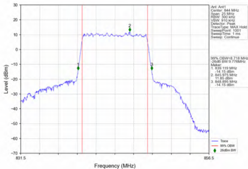
n5_30kHz_SISO_NTNV_10MHz_CP-OFDM 64 QAM_844MHz_Outer_Full
