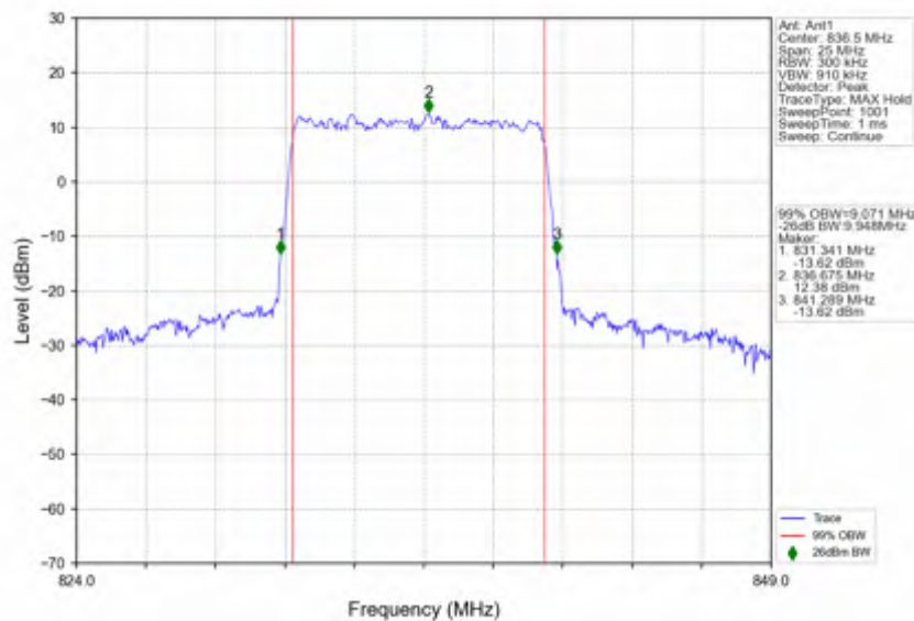
n5_15kHz_SISO_NTNV_10MHz_DFT-s-OFDM_16_QAM_836.5MHz_Outer_Full
