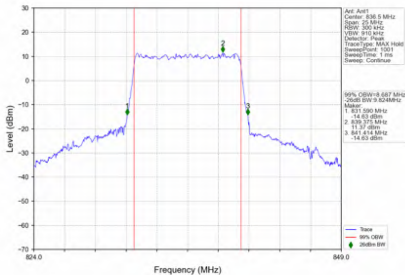
n5_30kHz_SISO_NTNV_10MHz_CP-OFDM 16 QAM_836.5MHz_Outer_Full
