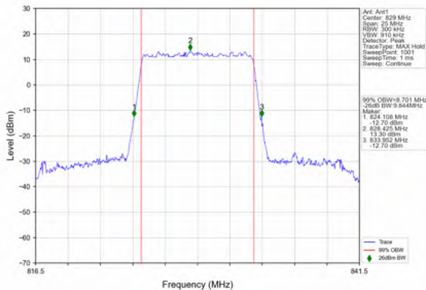
n5_30kHz_SISO_NTNV_10MHz_DFT-s-OFDM QPSK_829MHz_Outer_Full
