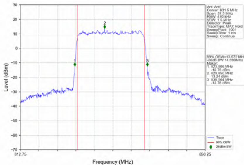
n5_15kHz_SISO_NTV_15MHz_DFT-s-OFDM 64 QAM 831.5MHz_Outer_Full
