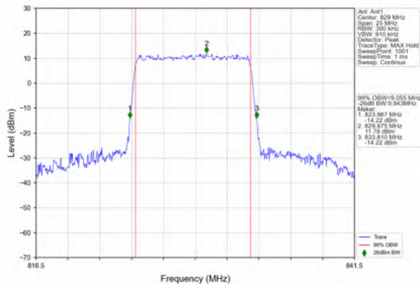
n5_15kHz_SISO_NTNV_10MHz_DFT-s-OFDM_64 QAM_829MHz_Outer_Full
