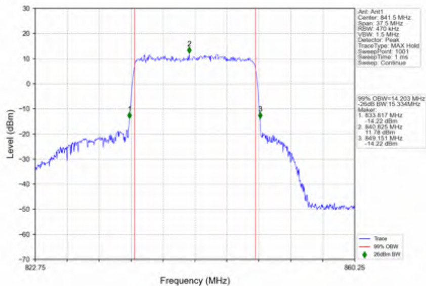
n5_15kHz_SISO_NTV_15MHz_CP-OFDM 64 QAM_841.5MHz_Outer_Full
