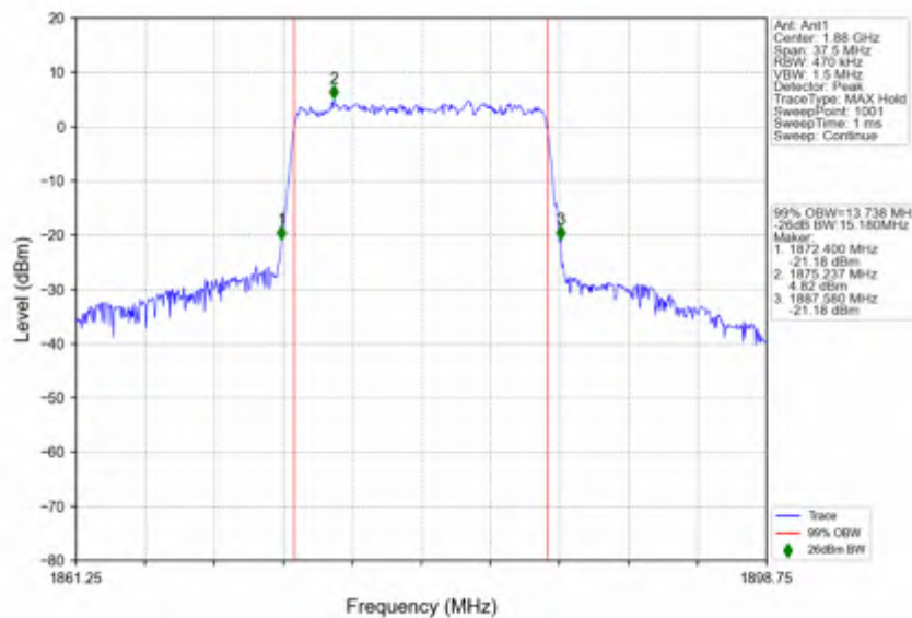
n2_30kHz_SISO_NTNV_15MHz_CP-OFDM_16_QAM_1880MHz_Outer_Full
