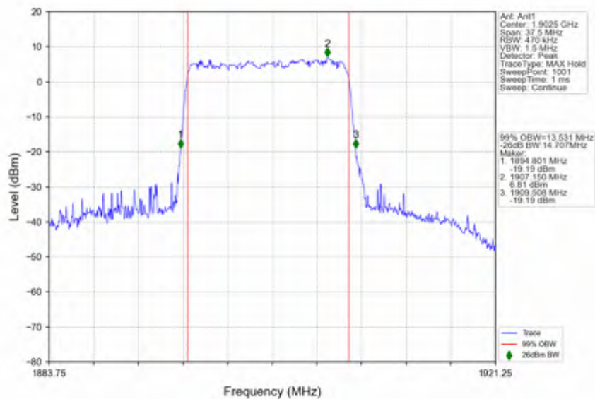
n2_15kHz_SISO_NTNV_15MHz_DFT-s-OFDM QPSK_1902.5MHz_Outer_Full
