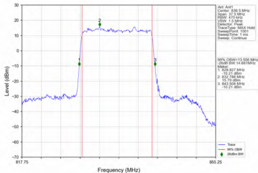
n5_15kHz_SISO_NTNV_15MHz_DFT-s-OFDM_PI/2_BPSK_836.5MHz_Outer_Full
