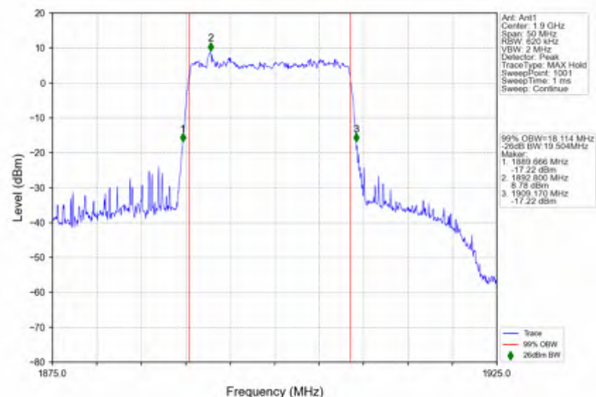
n2_15kHz_SISO_NTNV_20MHz_DFT-s-OFDM_QPSK_1900MHz_Outer_Full
