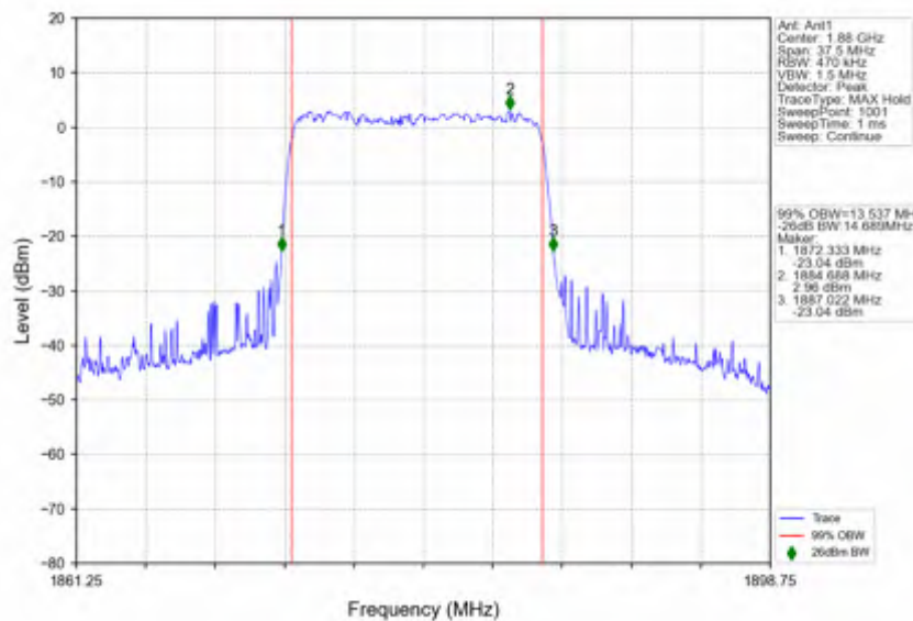
n2_15kHz_SISO_NTNV_15MHz_DFT-s-OFDM 256 QAM_1880MHz_Outer_Full
