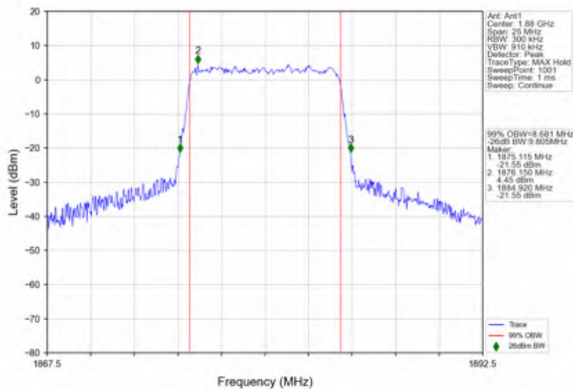
n2 30kHz SISO NTN 10MHz CP-OFDM 16 QAM 1880MHz Outer Full
