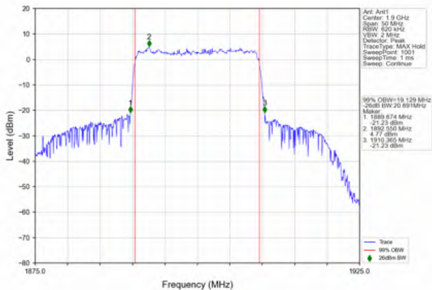
n2 15kHz SISO NTN 20MHz CP-OFDM 64 QAM 1900MHz Outer Full
