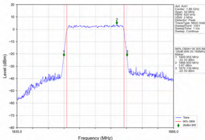
n2_30kHz_SISO_NTNV_20MHz_CP-OFDM 64 QAM_1860MHz_Outer_Full
