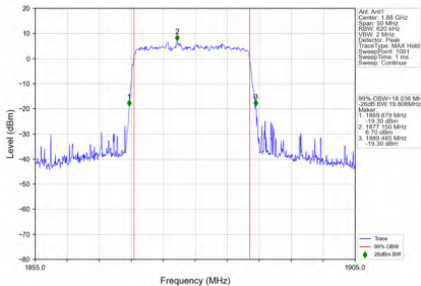
n2_15kHz_SISO_NTNV_20MHz_DFT-s-OFDM_16 QAM_1880MHz_Outer_Full
