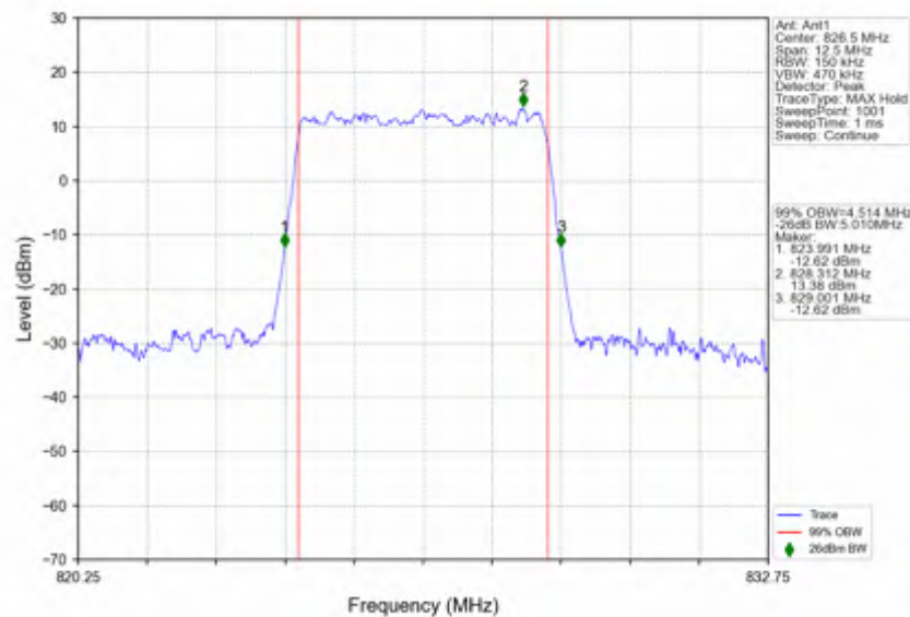
n5_15kHz_SISO_NTNV_5MHz_DFT-s-OFDM QPSK_826.5MHz_Outer_Full
