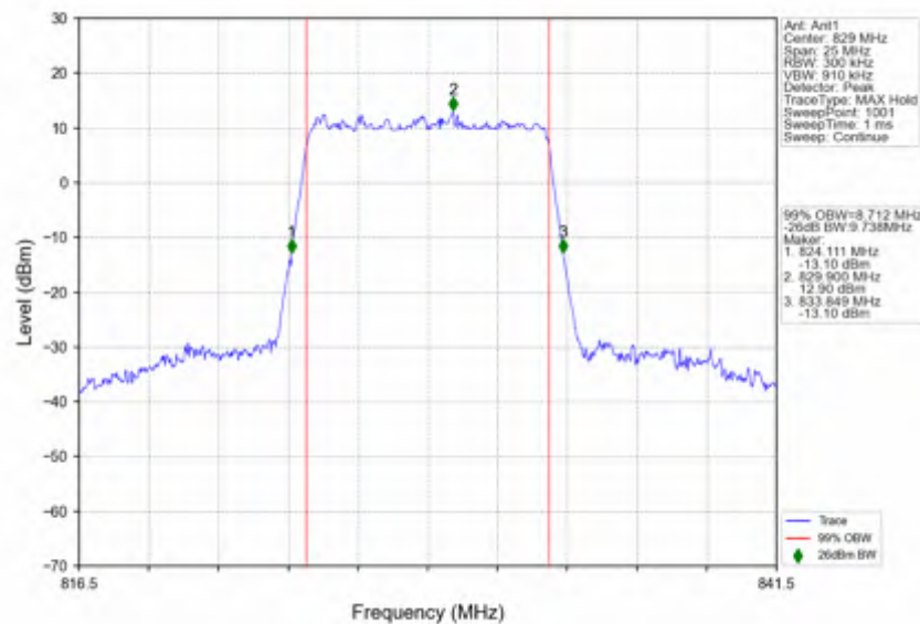
n5_30kHz_SISO_NTNV_10MHz_DFT-s-OFDM 64 QAM_829MHz_Outer_Full
