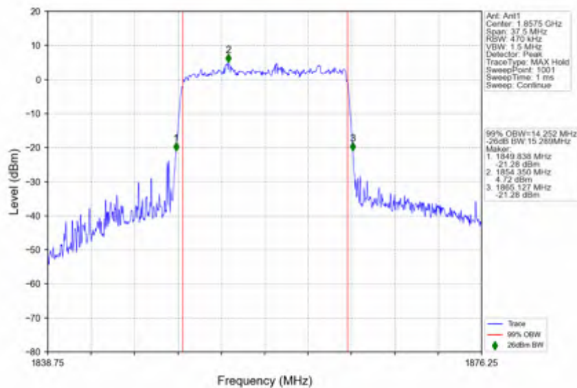
n2_15kHz_SISO_NTNV_15MHz_CP-OFDM_64_QAM_1857.5MHz_Outer_Full
