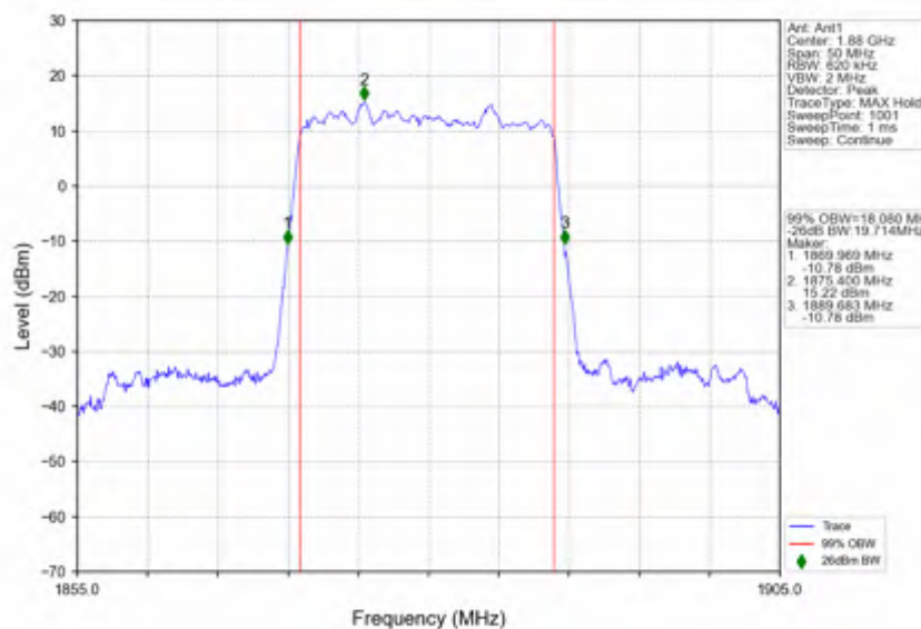
n2_30kHz_SISO_NTNV_20MHz_DFT-s-OFDM PI/2 BPSK_1880MHz_Outer_Full
