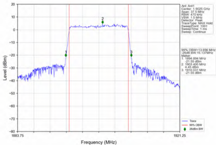
n2_30kHz_SISO_NTNV_15MHz_CP-OFDM 64 QAM_1902.5MHz_Outer_Full
