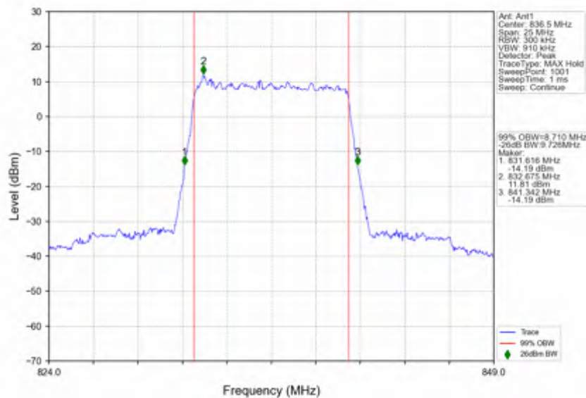
n5_30kHz_SISO_NTNV_10MHz_DFT-s-OFDM_256_QAM_836.5MHz_Outer_Full
