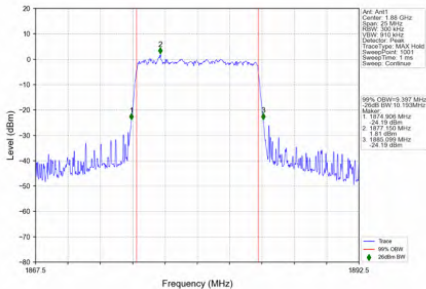
n2 15kHz SISO NTV 10MHz CP-OFDM 256 QAM 1880MHz Outer Full
