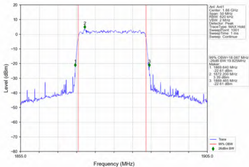
n2_15kHz_SISO_NTNV_20MHz_DFT-s-OFDM_256_QAM_1880MHz_Outer_Full
