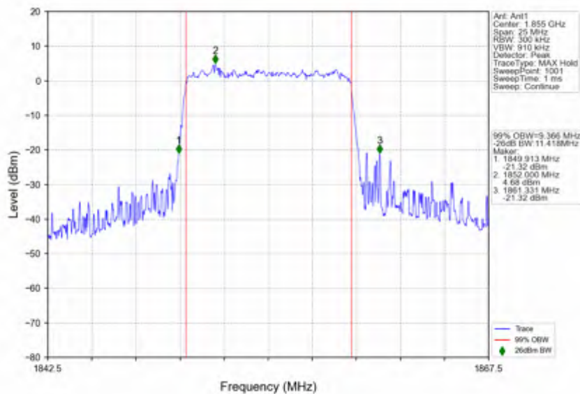
n2 15kHz SISO NTN 10MHz CP-OFDM 64 QAM 1855MHz Outer Full
