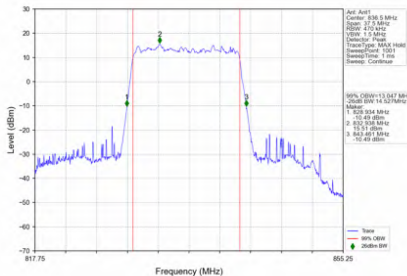
n5_30kHz_SISO_NTNV_15MHz_DFT-s-OFDM PI/2 BPSK_836.5MHz_Outer_Full
