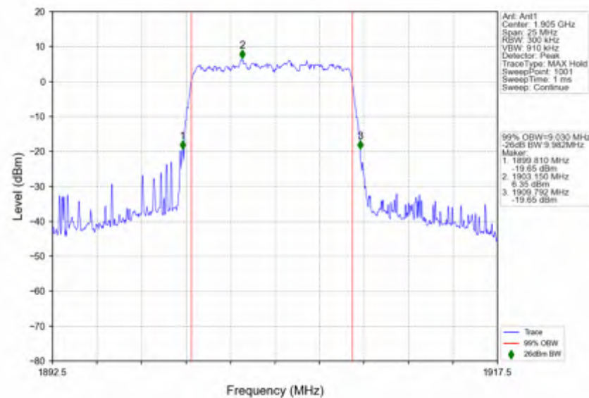
n2_15kHz_SISO_NTNV_10MHz_DFT-s-OFDM_QPSK_1905MHz_Outer_Full
