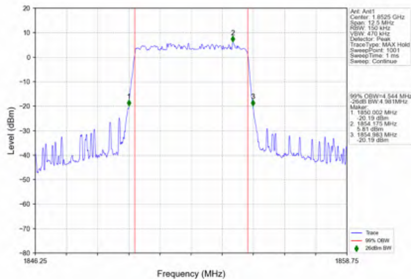
n2_15kHz_SISO_NTNV_5MHz_DFT-s-OFDM QPSK_1852.5MHz_Outer_Full
