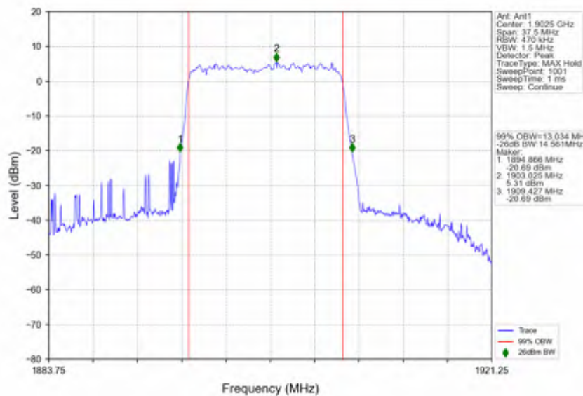
n2_30kHz_SISO_NTNV_15MHz_DFT-s-OFDM 64 QAM_1902.5MHz_Outer_Full
