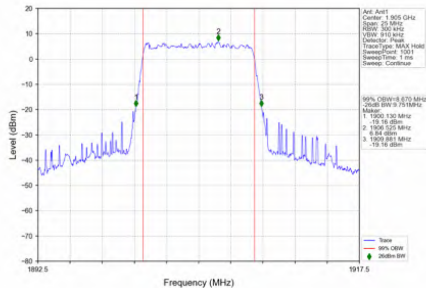
n2_30kHz_SISO_NTNV_10MHz_DFT-s-OFDM_QPSK_1905MHz_Outer_Full
