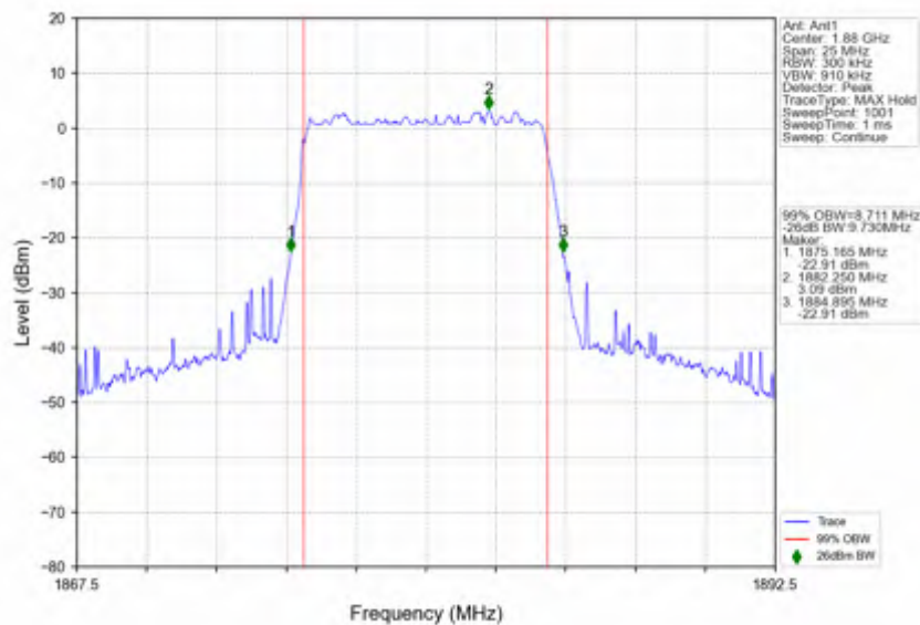
n2_30kHz_SISO_NTNV_10MHz_DFT-s-OFDM_256_QAM_1880MHz_Outer_Full
