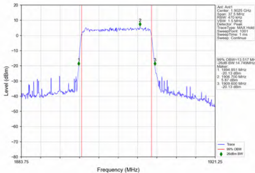
n2_15kHz_SISO_NTNV_15MHz_DFT-s-OFDM 64 QAM_1902.5MHz_Outer_Full
