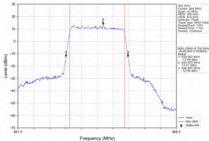
n5_30kHz_SISO_NTNV_10MHz_DFT-s-OFDM 64 QAM_844MHz_Outer_Full
