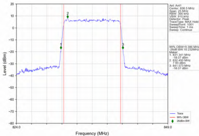
n5 15kHz SISO NTNV 10MHz CP-OFDM 256 QAM 836.5MHz Outer Full
