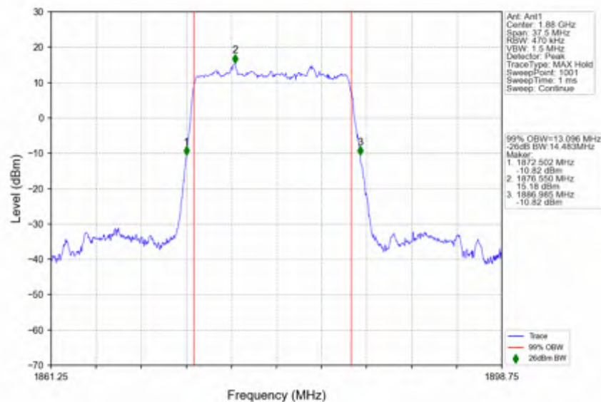
n2_30kHz_SISO_NTNV_15MHz_DFT-s-OFDM_PI/2_BPSK_1880MHz_Outer_Full
