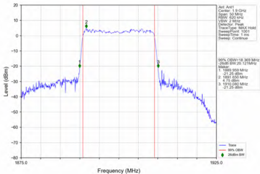
n2_30kHz_SISO_NTNV_20MHz_CP-OFDM 64 QAM_1900MHz_Outer_Full
