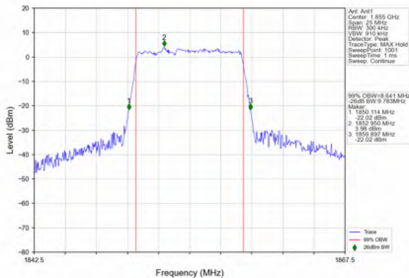
n2_30kHz_SISO_NTNV_10MHz_CP-OFDM_QPSK_1855MHz_Outer_Full
