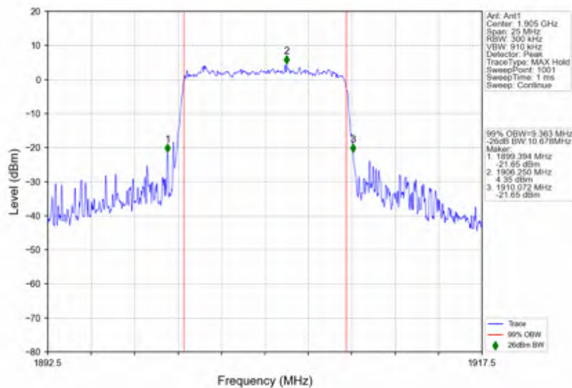
n2 15kHz SISO NTNV 10MHz CP-OFDM QPSK 1905MHz Outer Full
