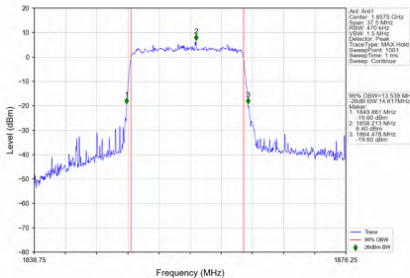
n2_15kHz_SISO_NTNV_15MHz_DFT-s-OFDM 64 QAM_1857.5MHz_Outer_Full
