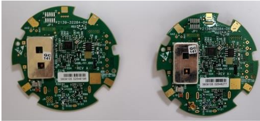
RF card- bottom, identical but extra mmcX connector for external antenna configuration (right card)
