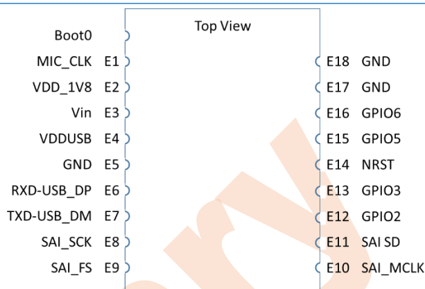
Figure 2 - OSM-1-1313 Pinout
