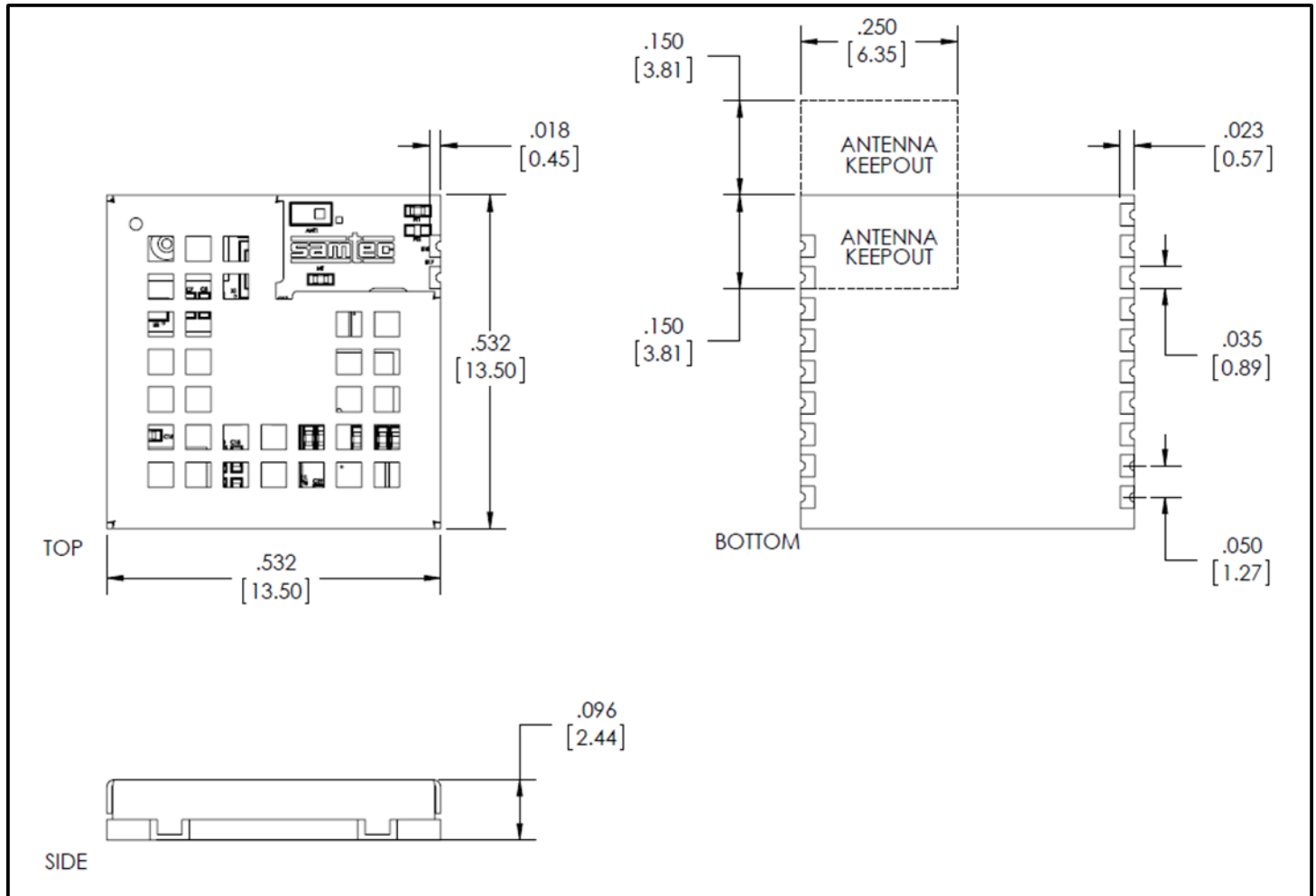
Figure 8 - OSM-1-1313 Mechanical Dimensions
