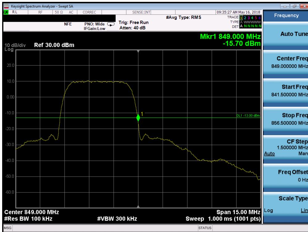
Plot 7-86. Band Edge Plot (Cellular WCDMA Mode - High Channel)
