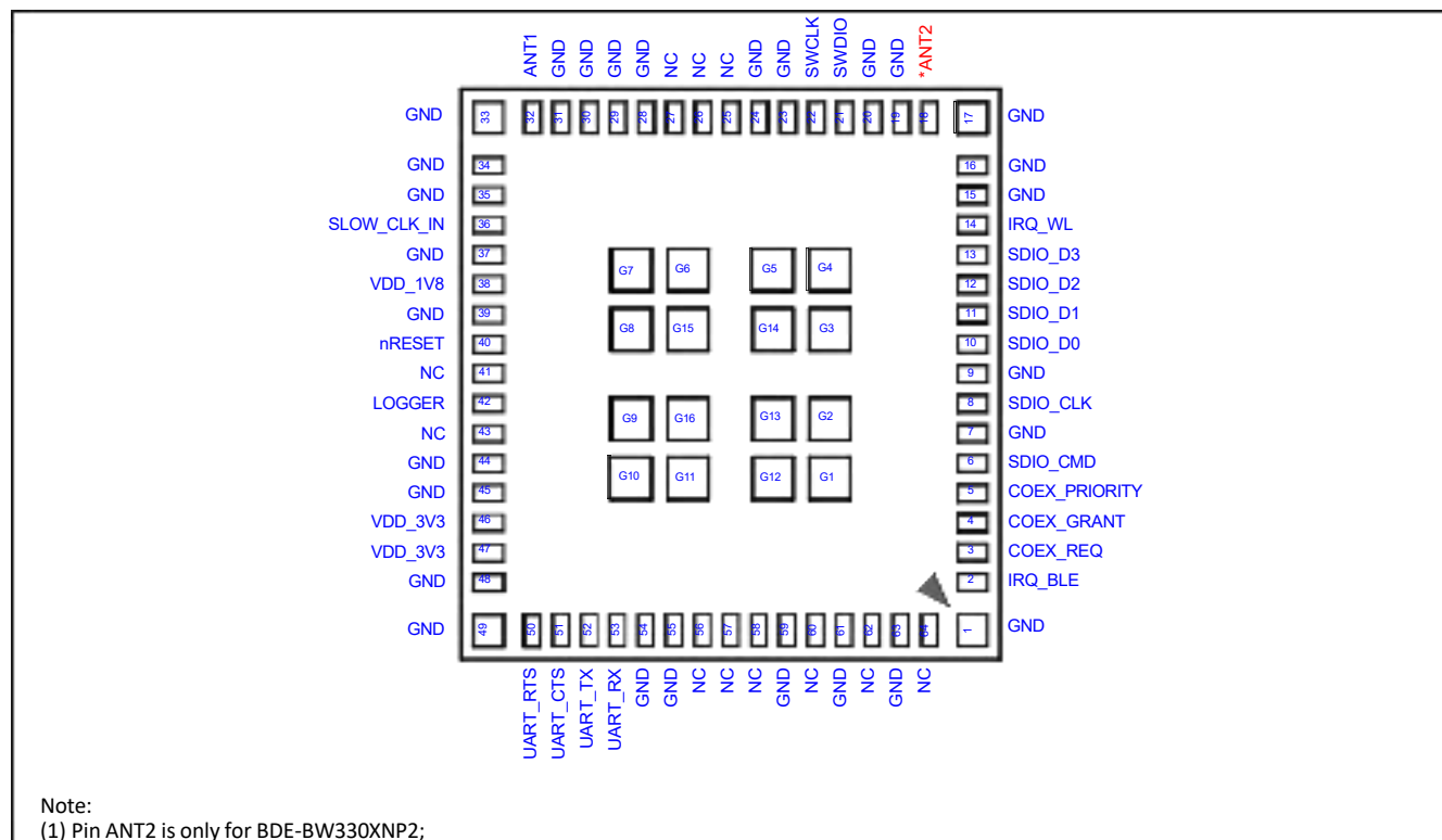
Figure 4. Pin Diagram of BDE-BW330XNP1 and BDE-BW330XNP2 (Top View)
