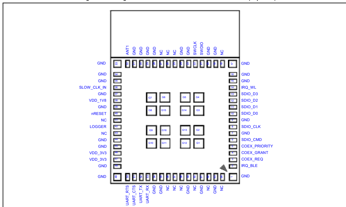
Figure 5. Pin Diagram of BDE-BW330XUP1 and BDE-BW330XUP2 (Top View)
