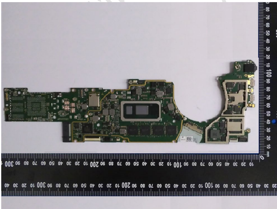
PCB view-03
