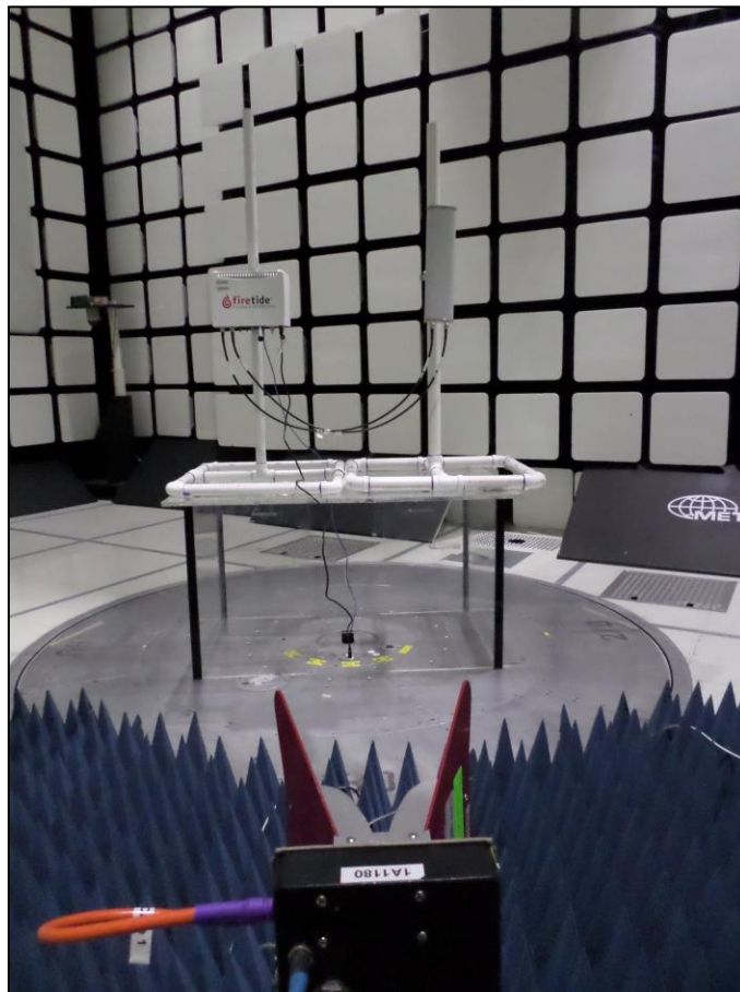
Photograph 6. Radiated Spurious Emissions, Above 1 GHz, 13dBi Panel Antenna, Test Setup
