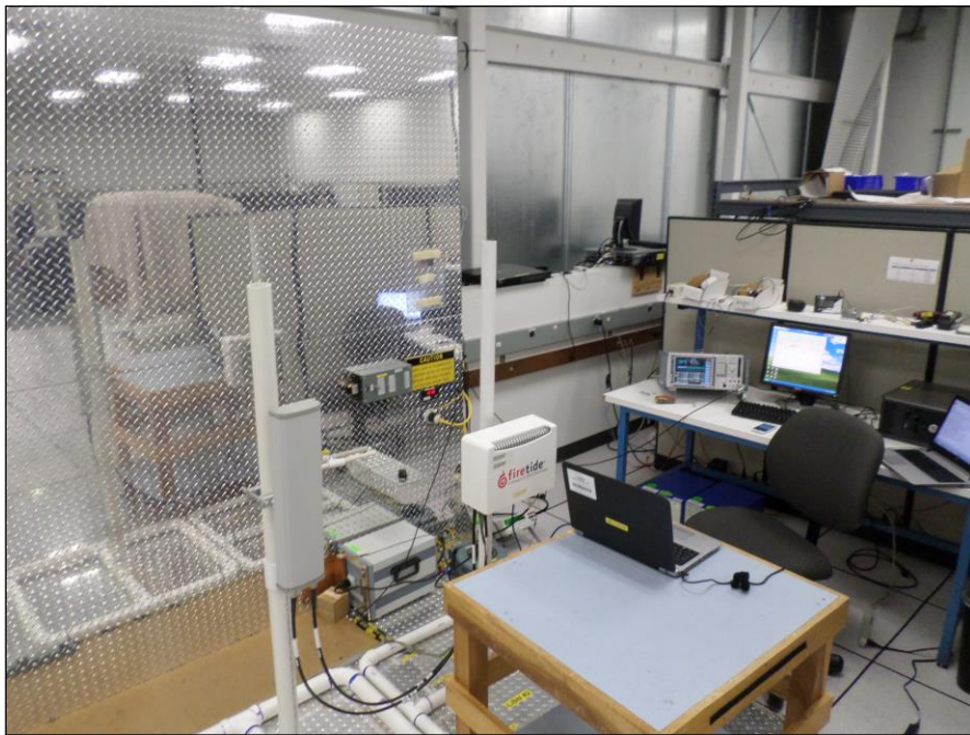
Photograph 2. Conducted Emissions, 15.207(a), Test Setup, 13 dBi Antenna
