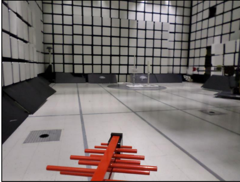
Photograph 3. Radiated Spurious Emissions, Below 1 GHz, 9dBi Omni Antenna, Test Setup
