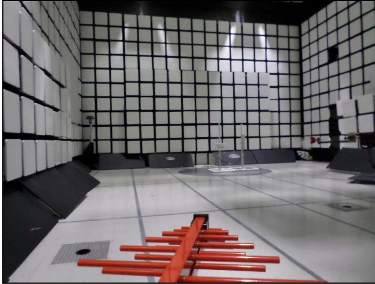
Photograph 5. Radiated Spurious Emissions, Below 1 GHz, 13dBi Panel Antenna, Test Setup
