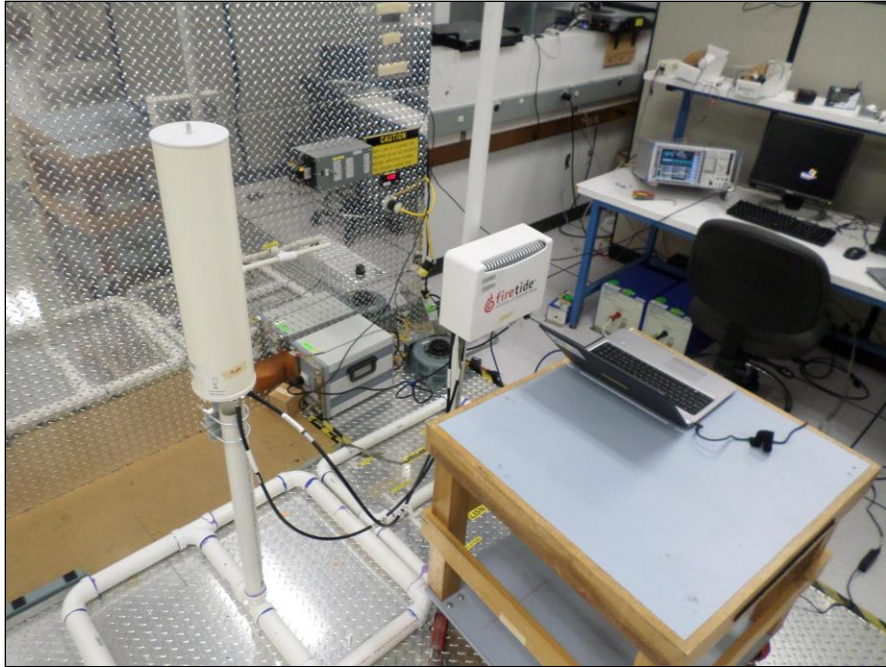
Photograph 1. Conducted Emissions, 15.207(a), Test Setup, 9 dBi Antenna
