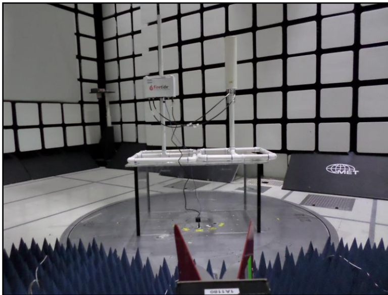
Photograph 4. Radiated Spurious Emissions, Above 1 GHz, 9dBi Omni Antenna, Test Setup
