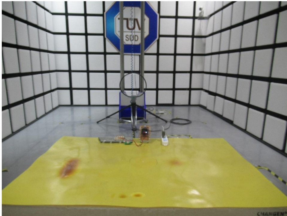
Radiated Emission 9KHz to 30MHz
