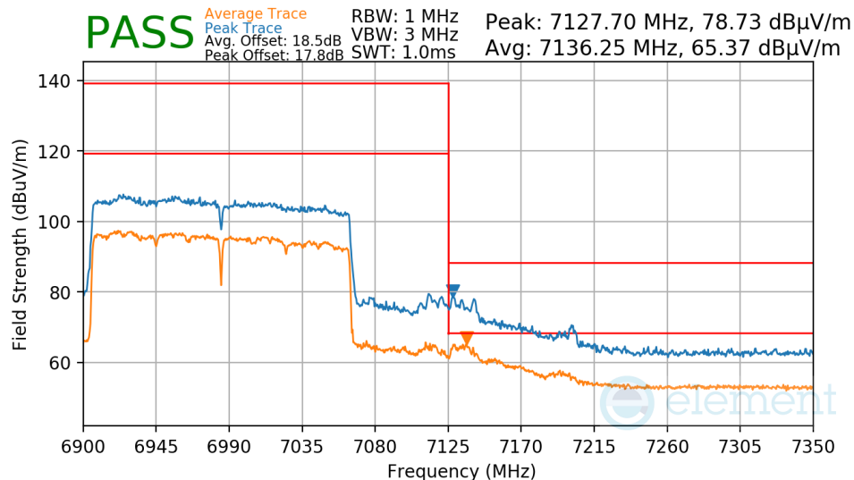
Plot 7-926. Antenna WF7a Radiated Upper Band Edge (Peak & Average – UNII Band 8)
