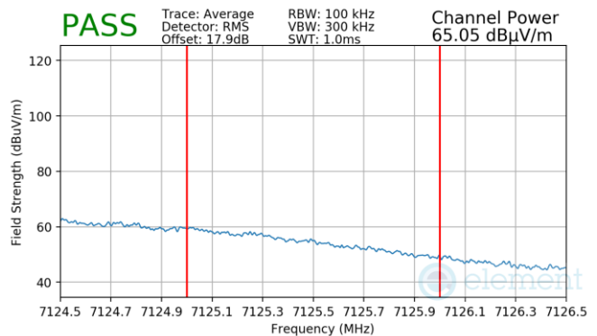
Plot 7-892. Antenna WF7a Radiated Upper Band Edge (Average – UNII Band 8)
