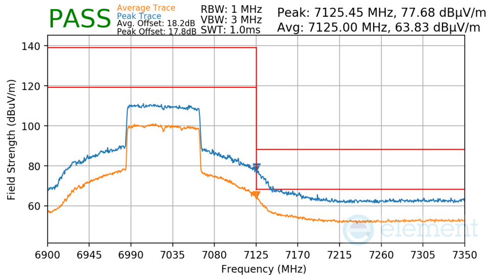
Plot 7-919. Antenna WF7a Radiated Upper Band Edge (Peak & Average – UNII Band 8)
