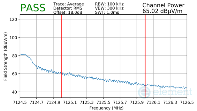
Plot 7-904. Antenna WF7a Radiated Upper Band Edge (Average – UNII Band 8)
