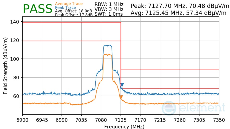
Plot 7-900. Antenna WF7a Radiated Upper Band Edge (Peak/Average – UNII Band 8)
