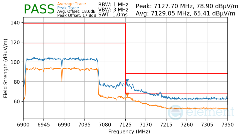
Plot 7-884. Antenna WF8 Radiated Upper Band Edge (Peak & Average – UNII Band 8)
