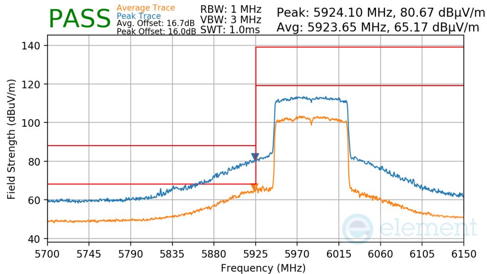
Plot 7-875. Antenna WF8 Radiated Lower Band Edge (Peak & Average – UNII Band 5)
