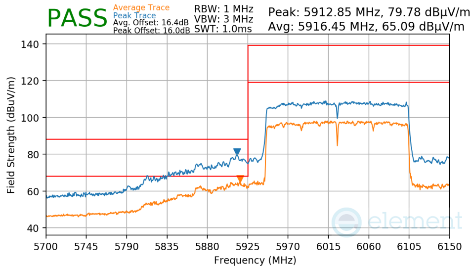
Plot 7-923. Antenna WF7a Radiated Lower Band Edge (Peak & Average – UNII Band 5)
