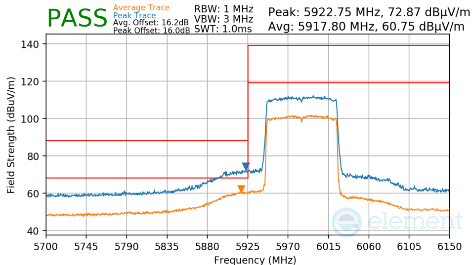
Plot 7-915. Antenna WF7a Radiated Lower Band Edge (Peak & Average – UNII Band 5)
