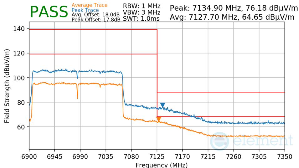
Plot 7-882. Antenna WF8 Radiated Upper Band Edge (Peak & Average – UNII Band 8)
