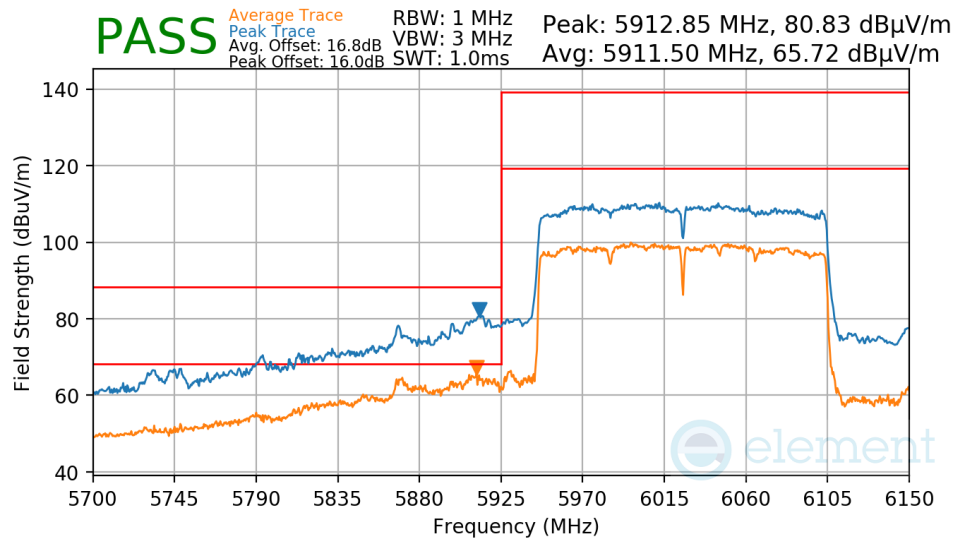
Plot 7-881. Antenna WF8 Radiated Lower Band Edge (Peak & Average – UNII Band 5)
