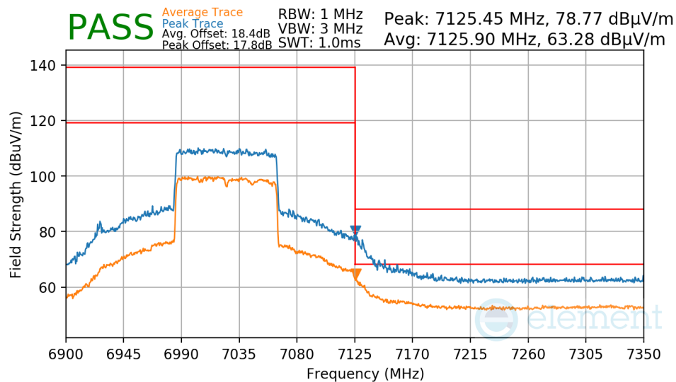
Plot 7-920. Antenna WF7a Radiated Upper Band Edge (Peak & Average – UNII Band 8)
