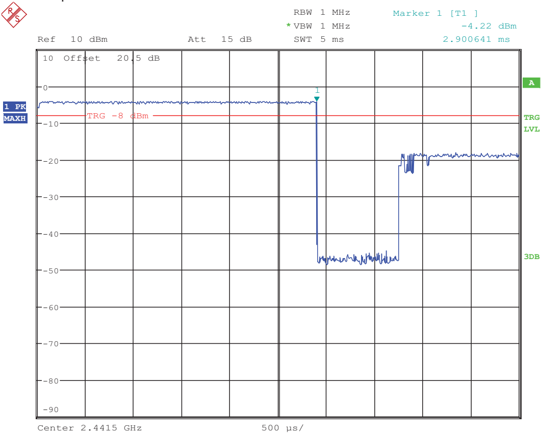
DH5 pulse's on time: 2.901ms
