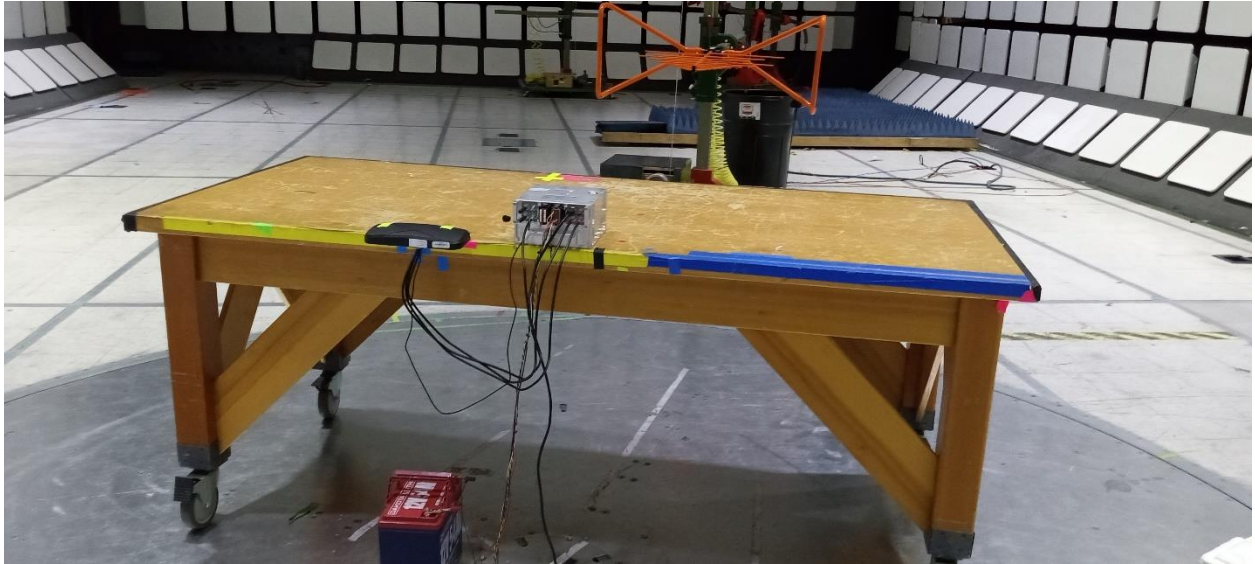
30MHz – 1 GHz, X Axis
