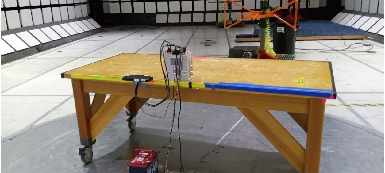
30MHz – 1 GHz, Z Axis
