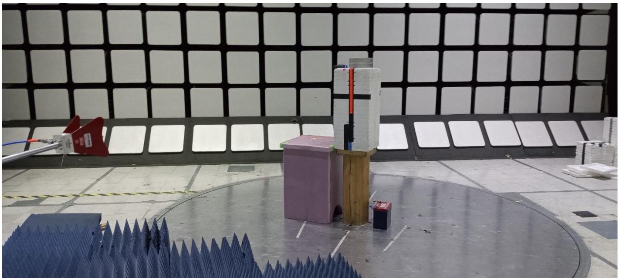
>1GHz Radiated Emissions
