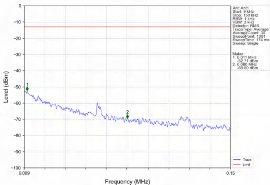
Band2_5MHz_QPSK_LCH_1852.5MHz_RB_1_0_NTNV
