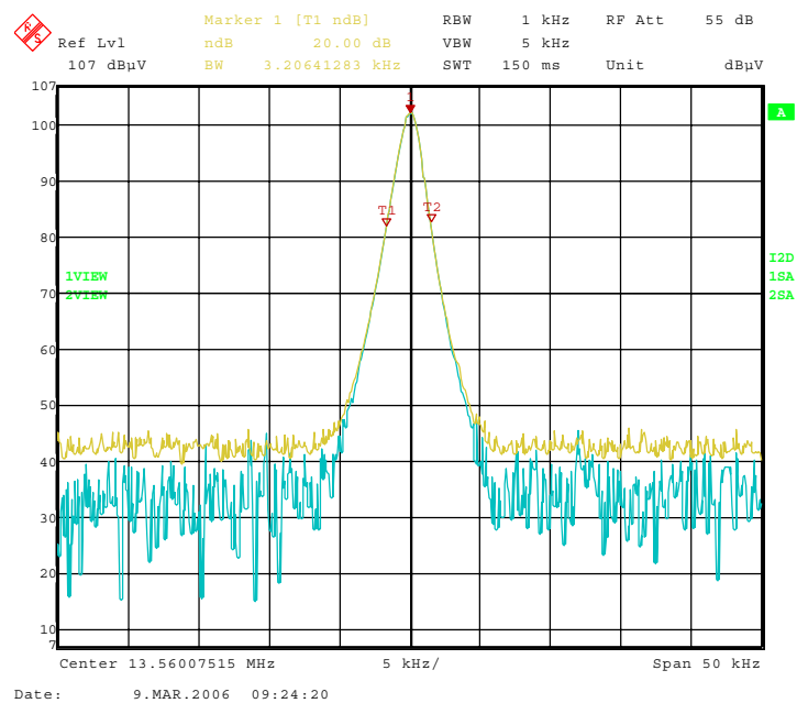
20 dB Bandwidth
