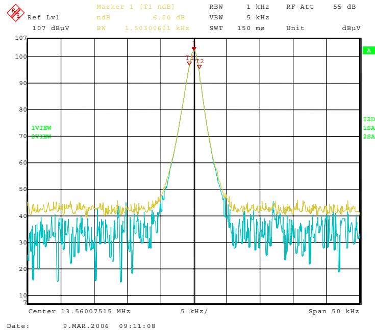
6 dB Bandwidth
