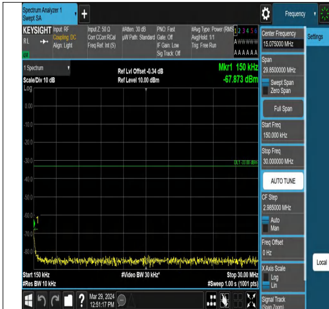
Band2_5MHz_QPSK_18900_1RB#0_0.15~30_0.15~30
