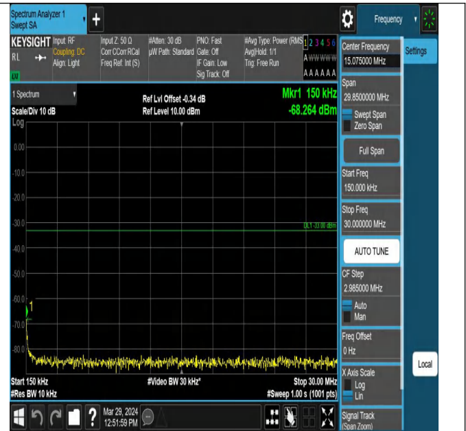
Band2_5MHz_QPSK_19175_1RB#0_0.15~30_0.15~30
