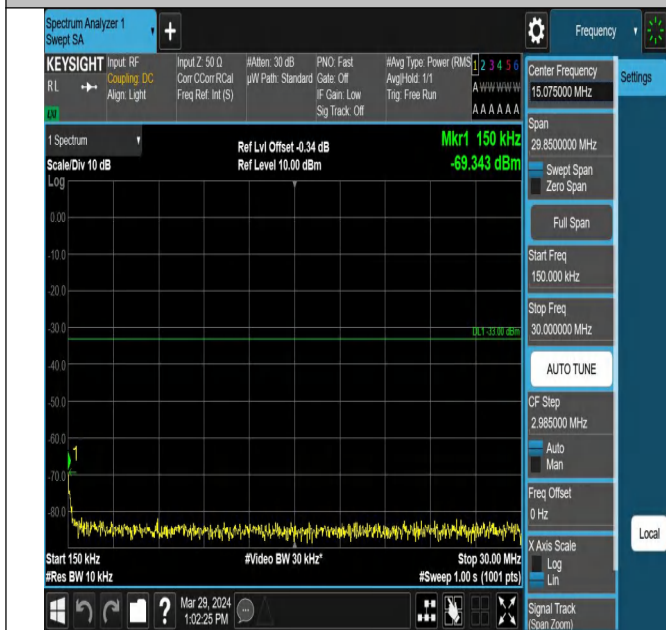
Band2_20MHz_QPSK_19100_1RB#0_0.15~30_0.15~30
