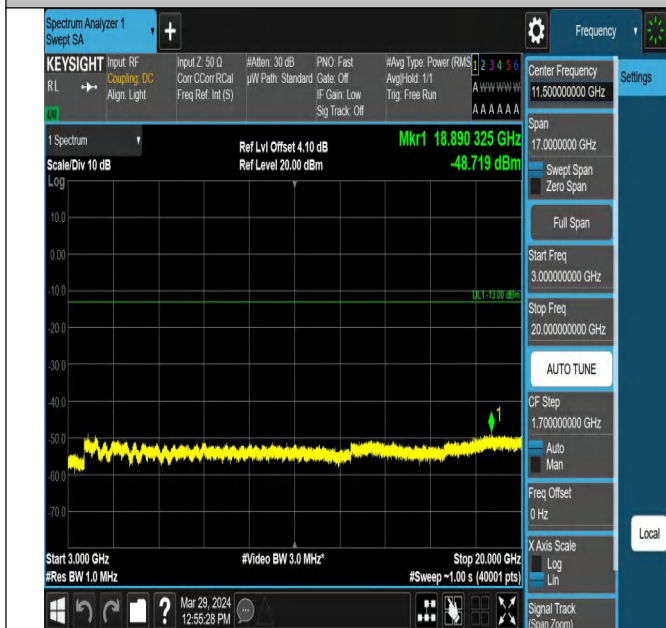
Band2_10MHz_QPSK_18900_1RB#0_3000~20000_3000~20
