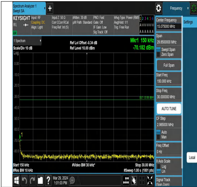
Band2_20MHz_QPSK_18700_1RB#0_0.15~30_0.15~30
