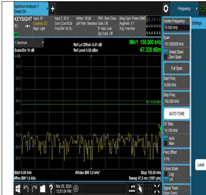
Band2_5MHz_QPSK_19175_1RB#0_0.009~0.15_0.009~0.15
