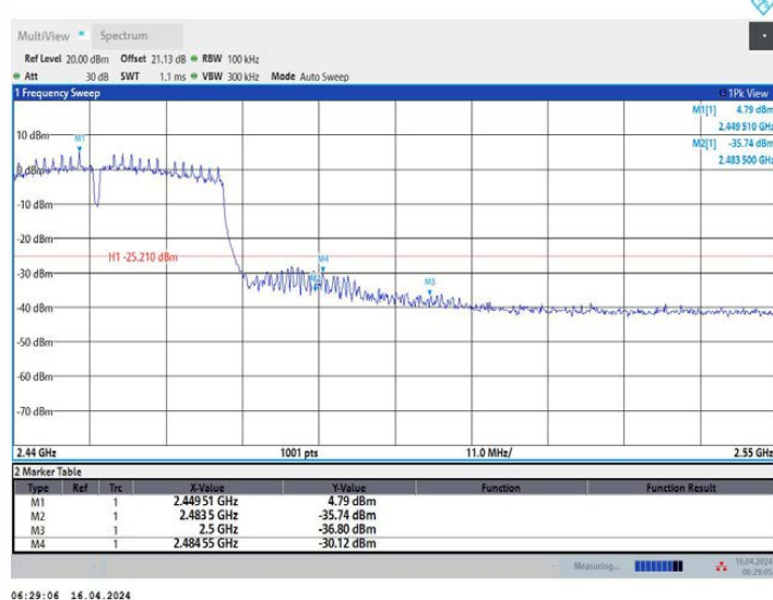
11N40MIMO_Ant1_High_2452
