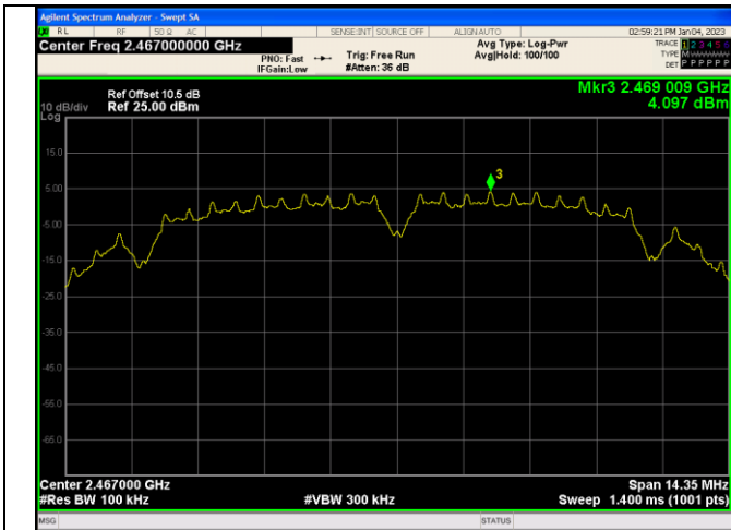
In-Band Reference Level IEEE 802.11b Channel 12 20MHz Antenna 0
