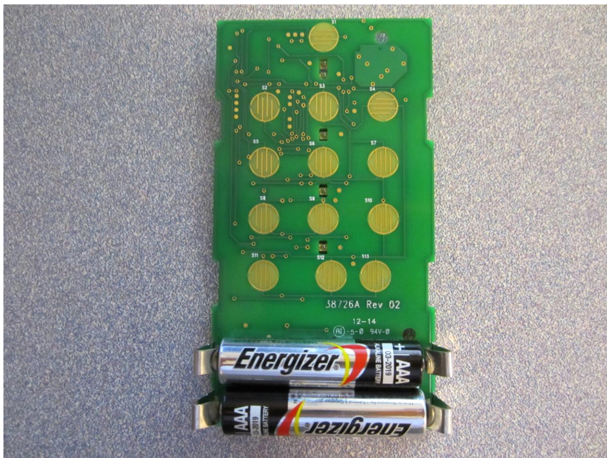
Figure 3: PCB Bottom
