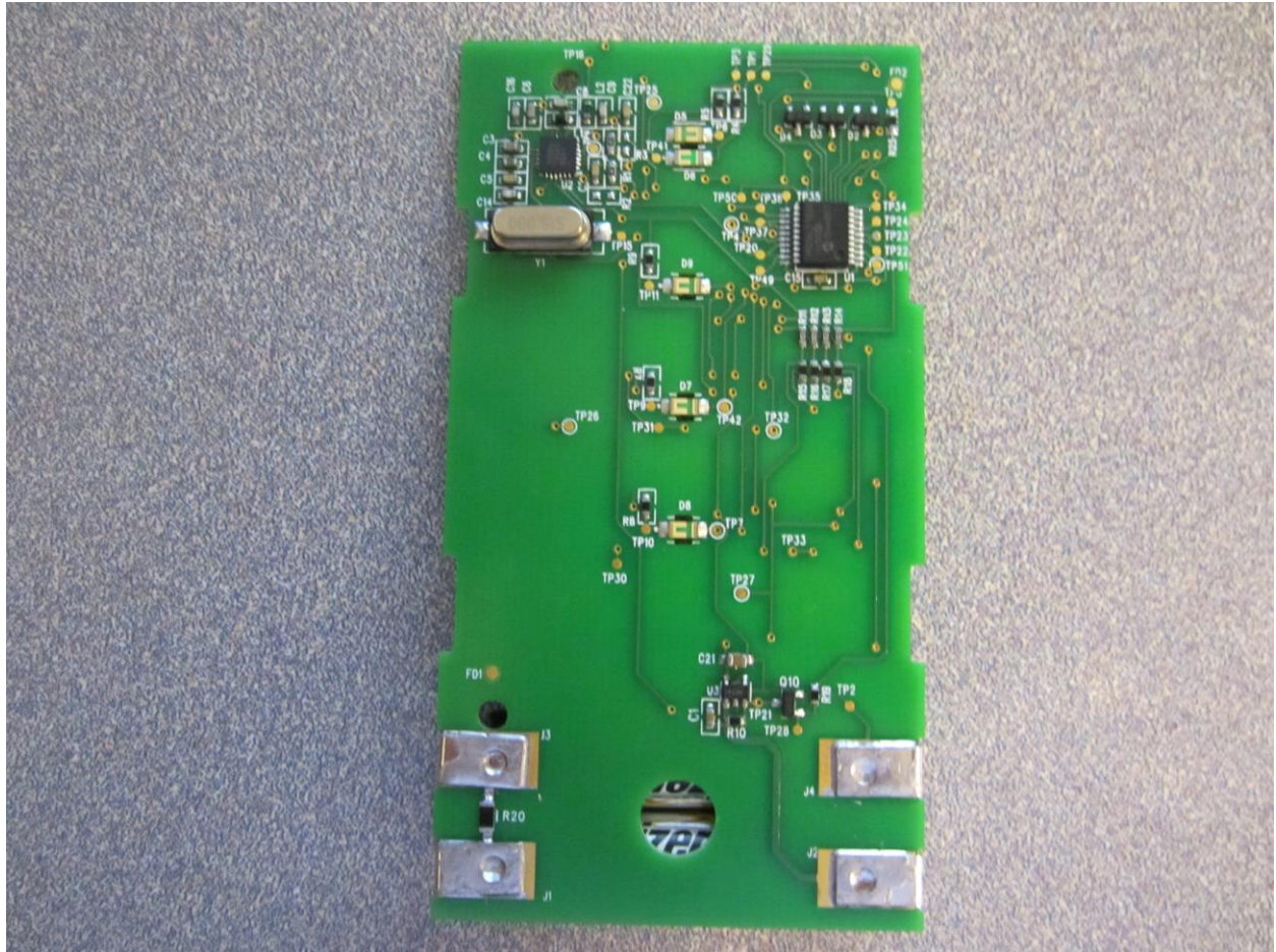
Figure 2: PCB Top
