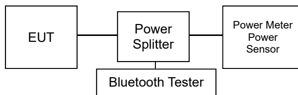
Figure 8.2.1 Average Power Measurement Setup
