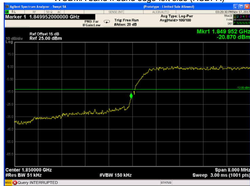
WCDMA band II band edge-left side (HSDPA)
