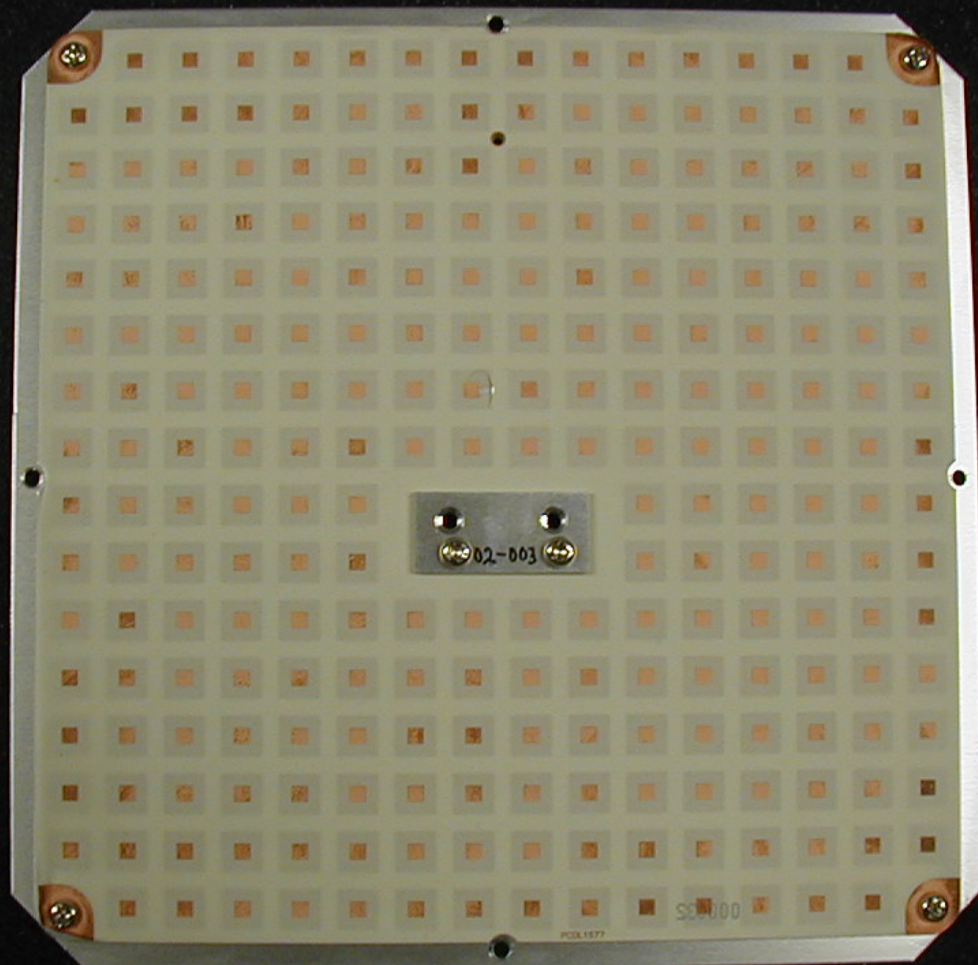
Type W WT Antenna
