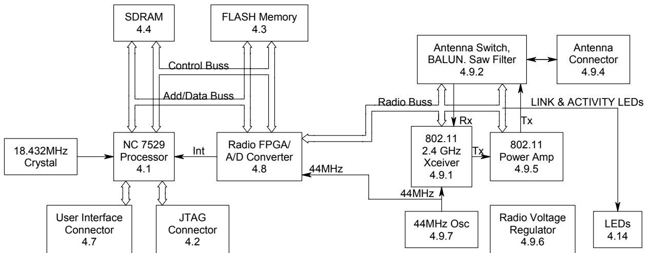
Digi Wi-EM Block Diagram
