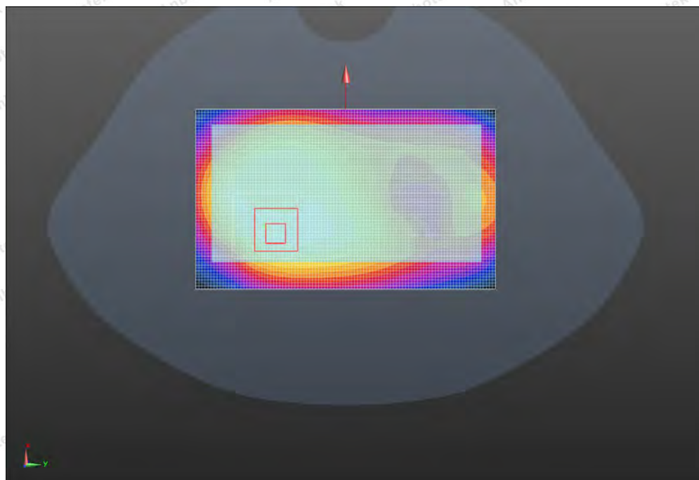
Rear Side (PCS1900 GPRS 4TS Middle Channel)
