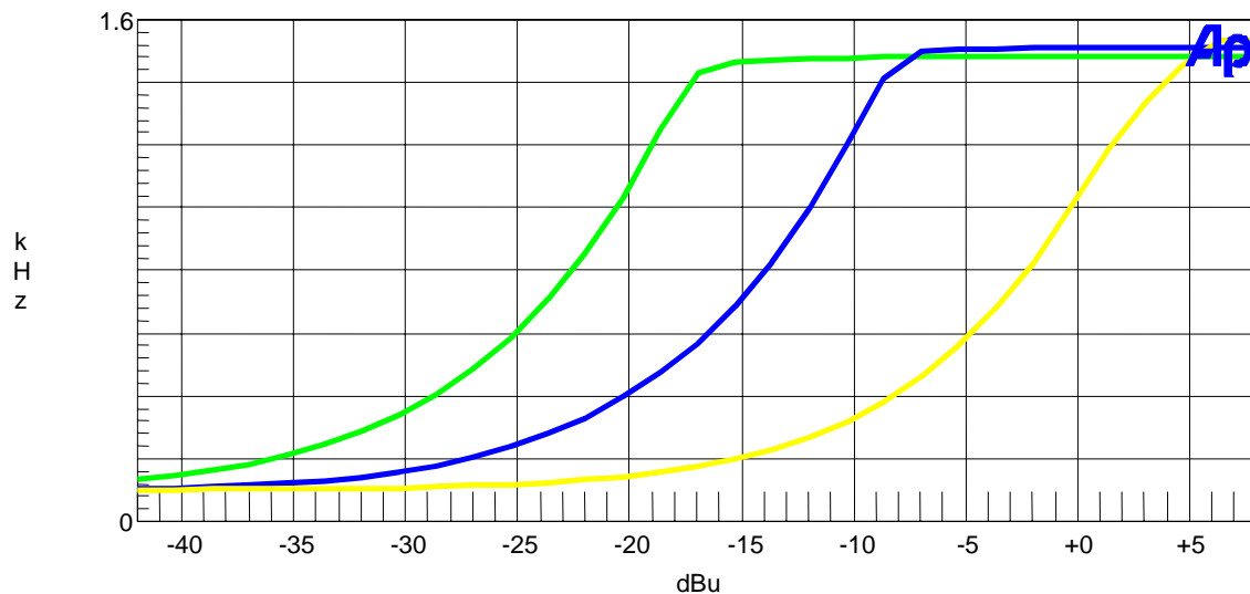
Modulation Limiting Plots Wide Band: 2.5 KHz (Green), 1.0 KHz (Blue), and 300 Hz (Yellow).
