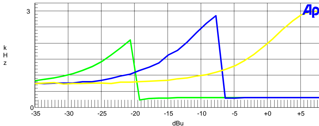
Modulation Limiting Plots Wide Band: 2.5 KHz (Green), 1.0 KHz (Blue), and 300 Hz (Yellow).
