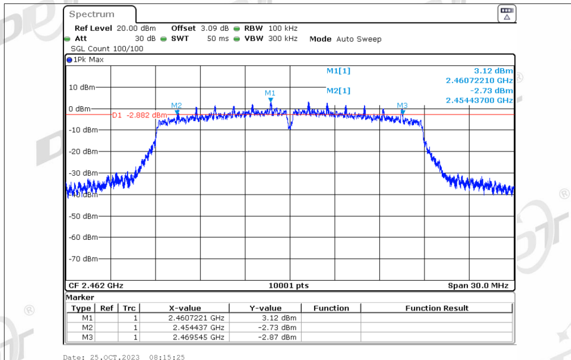
-6dB Bandwidth NVNT n20 2462MHz Ant2
