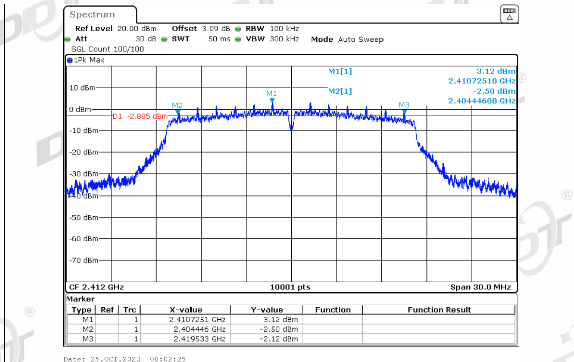
-6dB Bandwidth NVNT g 2412MHz Ant2
