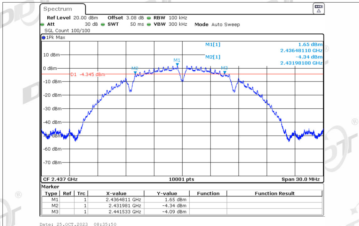
-6dB Bandwidth NVNT b 2437MHz Ant2
