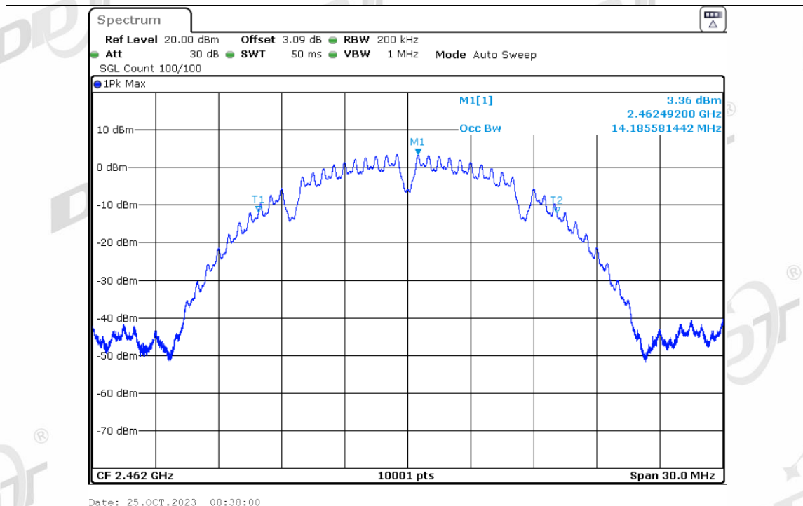
OBW NVNT b 2462MHz Ant2
