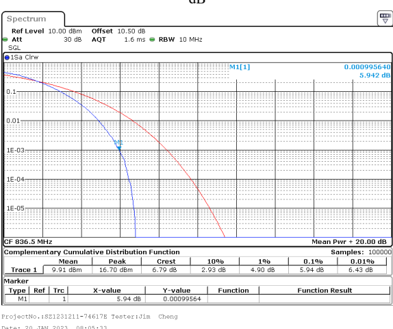
10MHz_15kHz_836.5MHz_DFT-s-OFDM 256 QAM_RB50@0&5.94 dB
