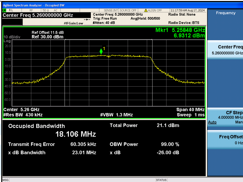
11N20MIMO-Ant2-5260
