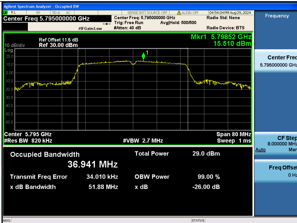
11AC40MIMO-Ant2-5795
