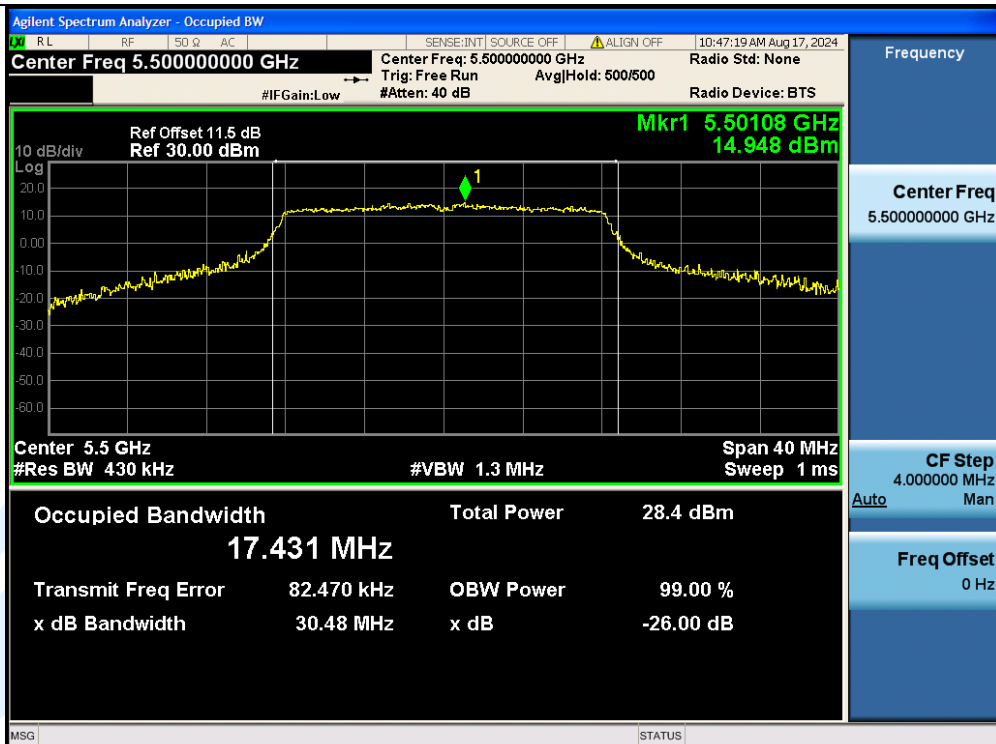
11A-Ant2-5500
