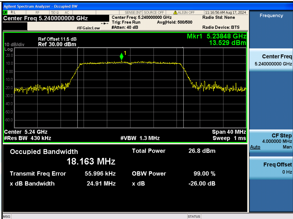
11N20MIMO-Ant2-5240
