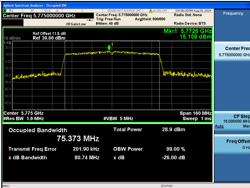
11AC80MIMO-Ant2-5775
