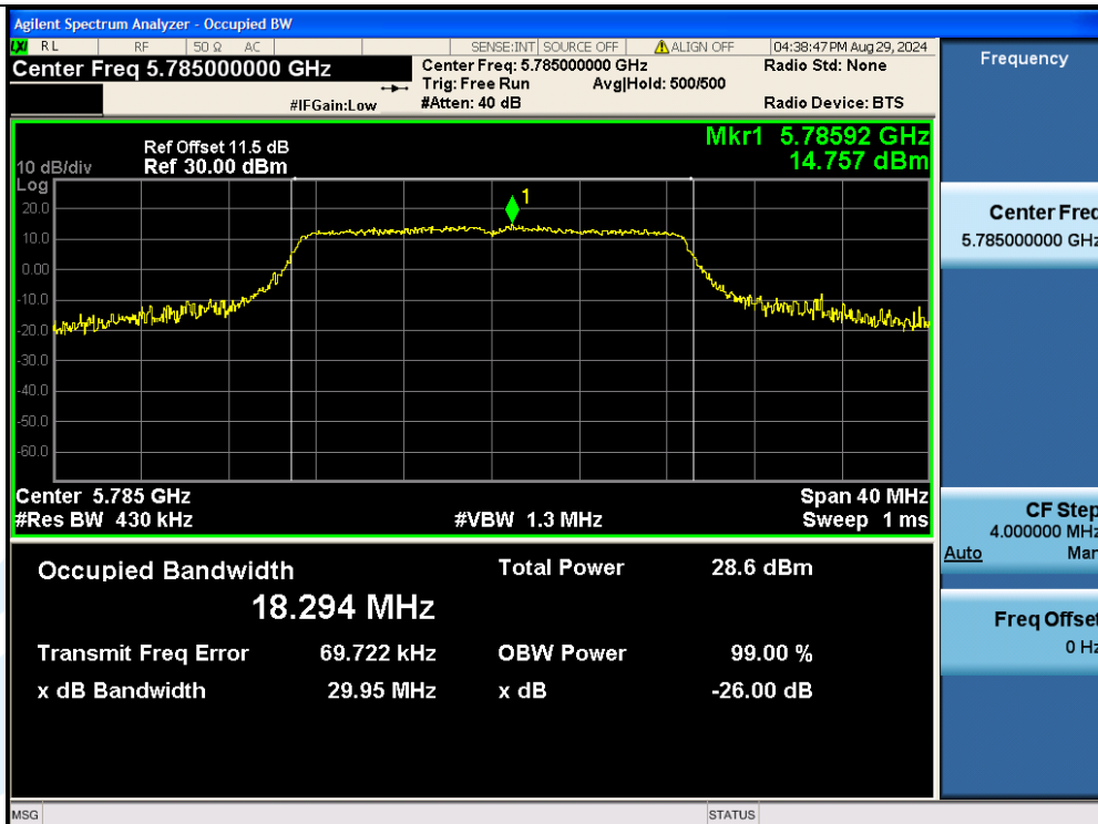
11N20MIMO-Ant2-5785
