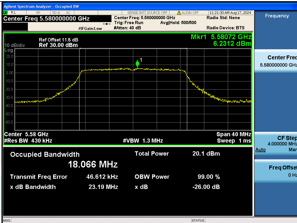
11N20MIMO-Ant2-5580
