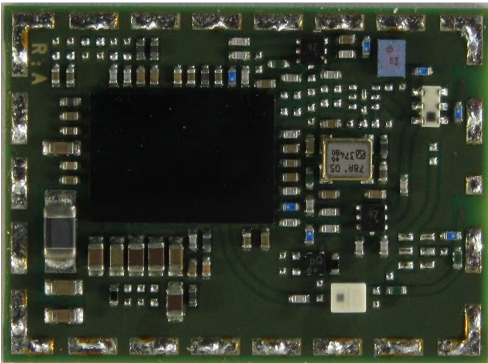
Figure 2: JODY-W164-07A internal photo
