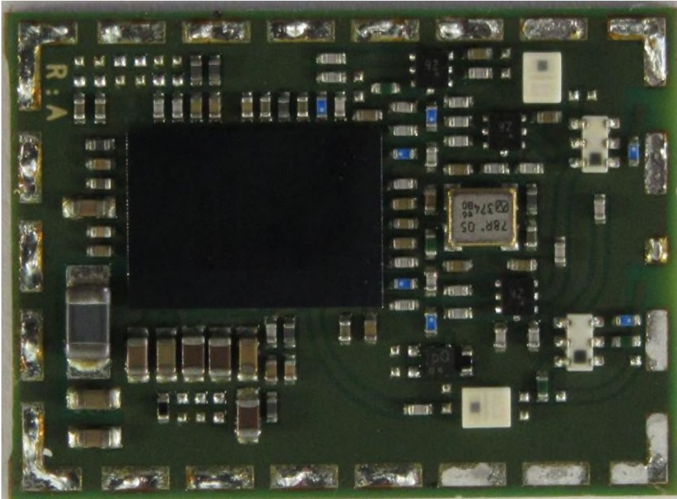
Figure 1: JODY-W164-03A internal photo
