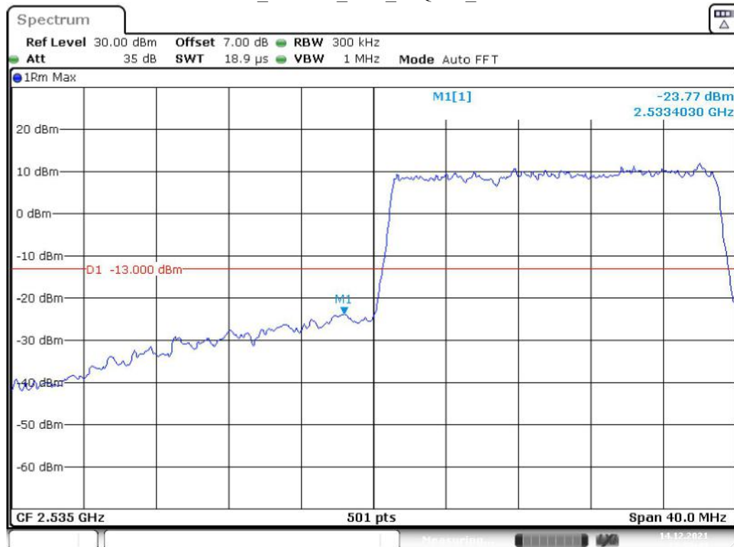
Band 41_20 MHz_Low_16QAM_RB100#0
