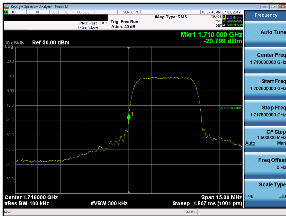
Plot 7-58. Band Edge Plot (AWS WCDMA Mode - Low Channel)
