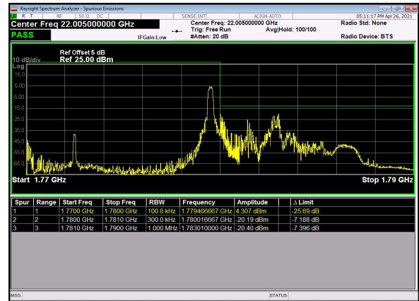
N66(15M)_DFT-s-OFDM_QPSK_Edge_1RB_R ght_High_CH
