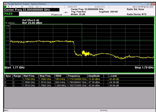
N66(15M)_DFT-s-OFDM_QPSK_Outer_Full_Hi gh_CH
