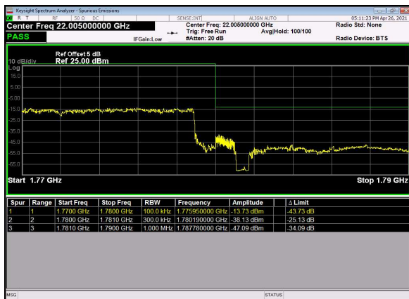
N66(15M)_DFT-s-OFDM_BPSK_Outer_Full_Hi gh_CH
