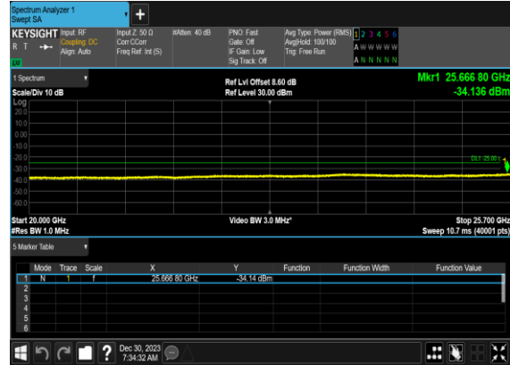
N7(5M)_DFT-s- OFDM_BPSK_Edge_1RB_Left_High_CH
