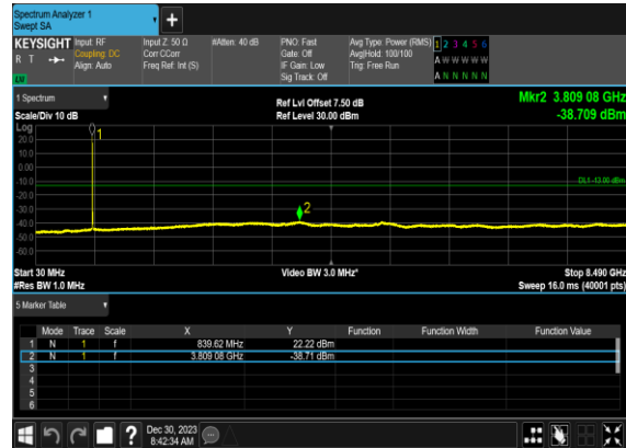
N5(10M)_DFT-s- OFDM_QPSK_Edge_1RB_Left_High_CH
