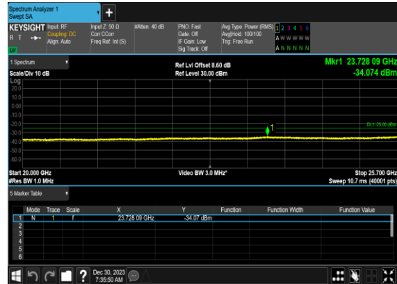
N7(5M)_DFT-s- OFDM_QPSK_Edge_1RB_Left_High_CH
