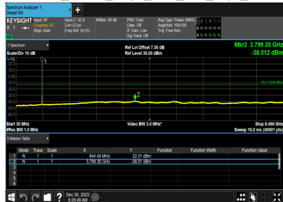
N5(5M)_DFT-s- OFDM_QPSK_Edge_1RB_Left_High_CH
