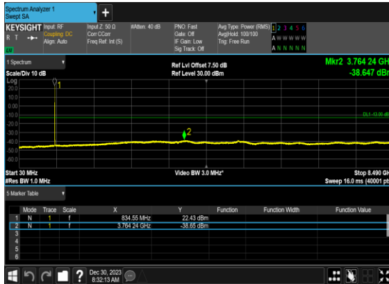
N5(5M)_DFT-s- OFDM_BPSK_Edge_1RB_Left_Mid_CH
