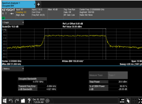
N7(5M)_CP-OFDM_64 QAM_Outer_Full_Mid_CH
