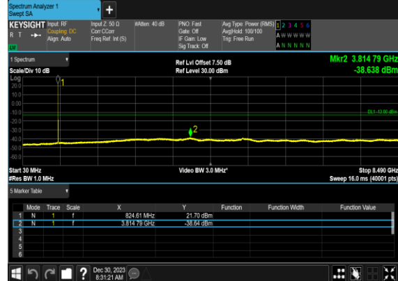
N5(5M)_DFT-s- OFDM_QPSK_Edge_1RB_Left_Low_CH
