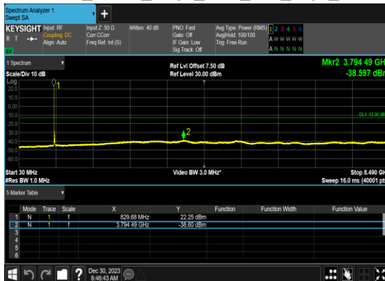
N5(20M)_DFT-s- OFDM_BPSK_Edge_1RB_Left_High_CH
