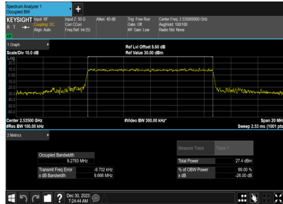
N7(10M)_CP-OFDM_16 QAM_Outer_Full_Mid_CH
