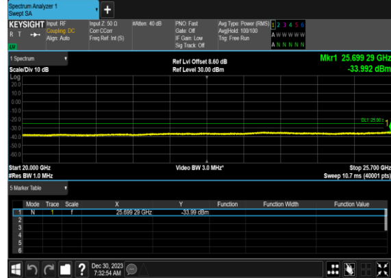
N7(5M)_DFT-s- OFDM_QPSK_Edge_1RB_Left_Mid_CH
