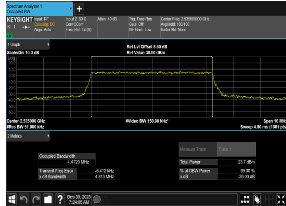
N7(5M)_CP-OFDM_256 QAM_Outer_Full_Mid_CH
