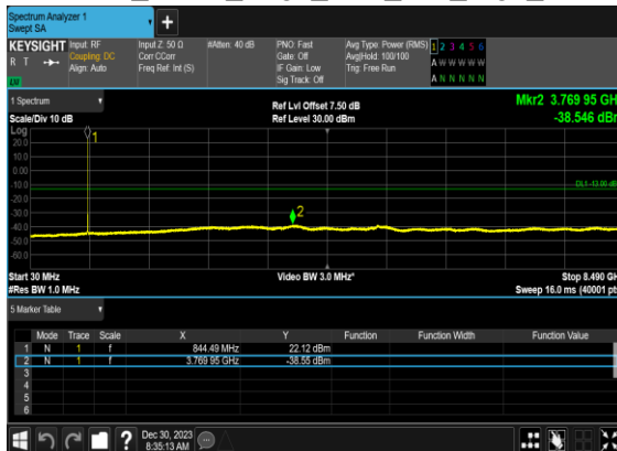
N5(5M)_DFT-s- OFDM_BPSK_Edge_1RB_Left_High_CH
