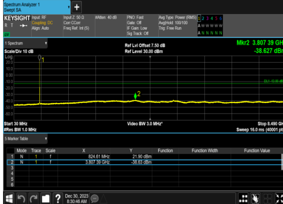
N5(5M)_DFT-s- OFDM_BPSK_Edge_1RB_Left_Low_CH
