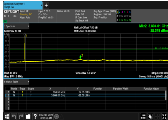
N5(5M)_DFT-s- OFDM_QPSK_Edge_1RB_Left_Mid_CH
