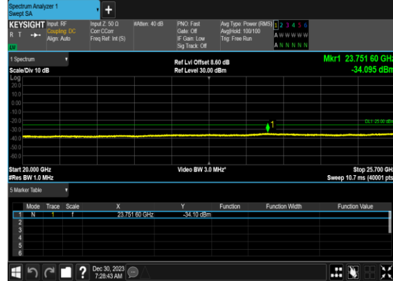
N7(5M)_DFT-s- OFDM_BPSK_Edge_1RB_Left_Low_CH
