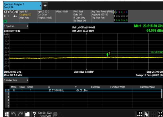
N7(5M)_DFT-s- OFDM_BPSK_Edge_1RB_Left_Mid_CH
