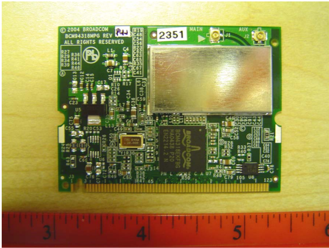
EUT – Top view shielded
