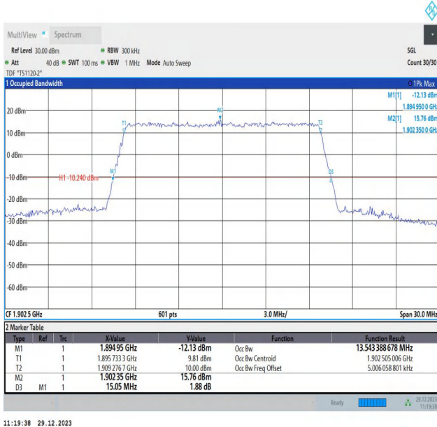
Band2-15MHz-64QAM-19125-75RB#0-PASS
