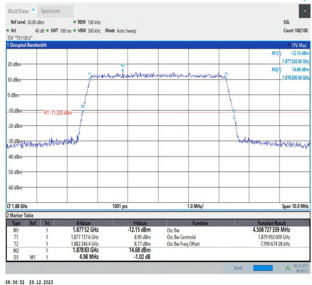
Band2-5MHz-64QAM-18900-25RB#0-PASS
