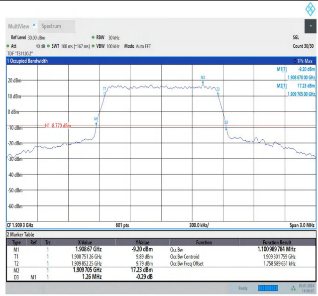
Band2-1.4MHz-16QAM-19193-6RB#0-PASS
