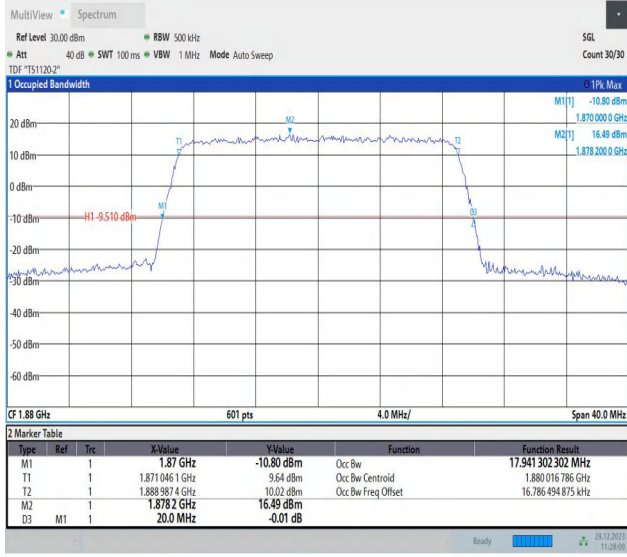
Band2-20MHz-64QAM-18900-100RB#0-PASS
