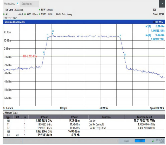
Band2-20MHz-64QAM-19100-100RB#0-PASS
