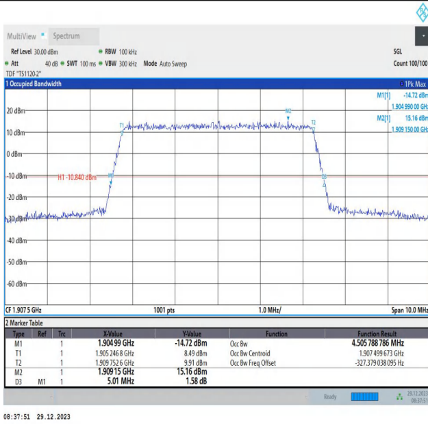
Band2-5MHz-64QAM-19175-25RB#0-PASS
