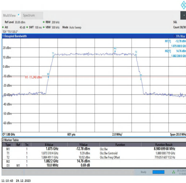
Band2-10MHz-64QAM-18900-50RB#0-PASS
