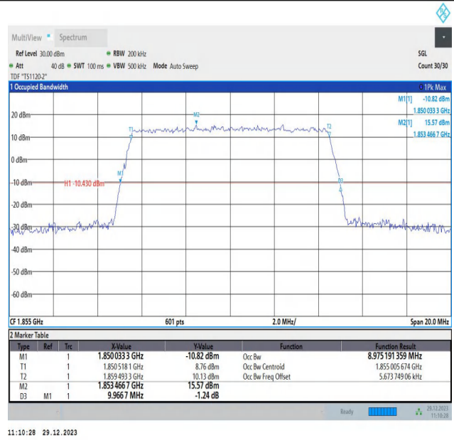
Band2-10MHz-64QAM-18650-50RB#0-PASS
