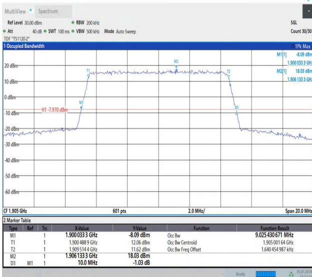
Band2-10MHz-QPSK-19150-50RB#0-PASS
