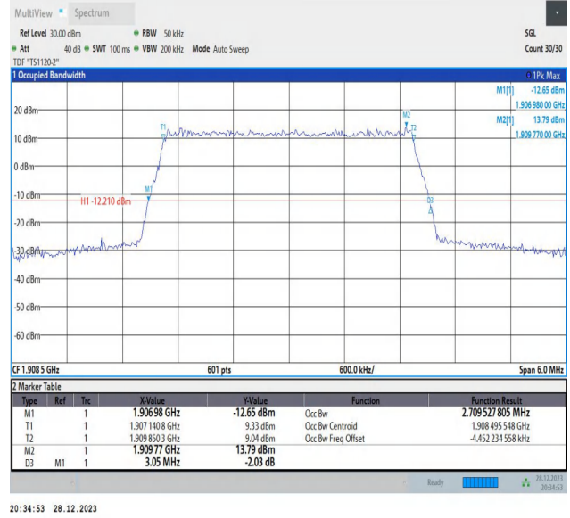
Band2-3MHz-64QAM-19185-15RB#0-PASS
