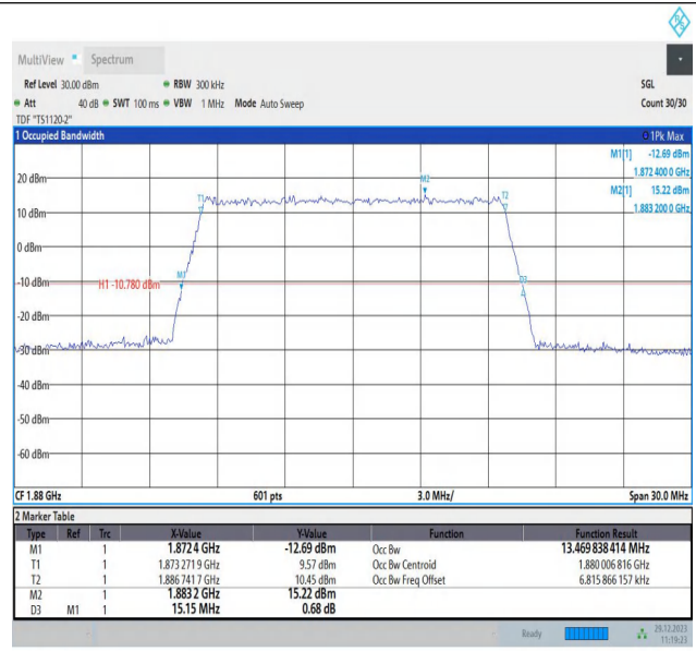
Band2-15MHz-64QAM-18900-75RB#0-PASS
