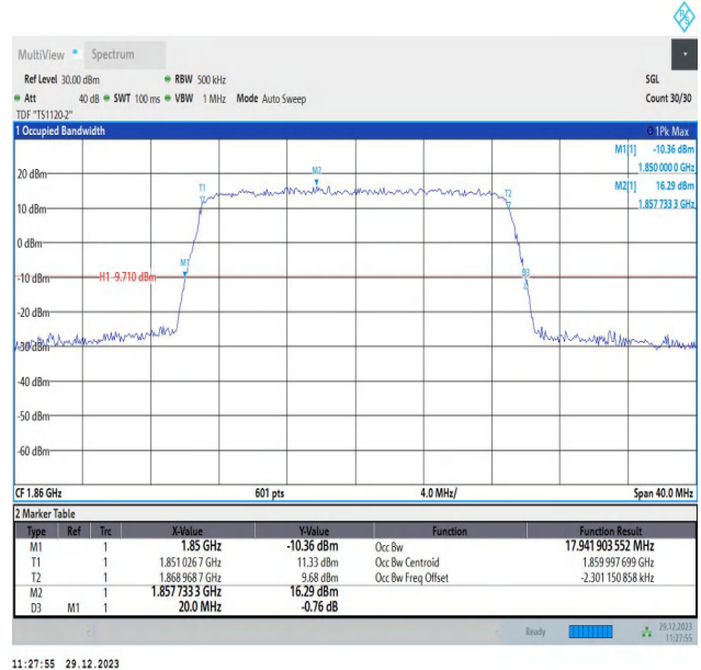
Band2-20MHz-64QAM-18700-100RB#0-PASS
