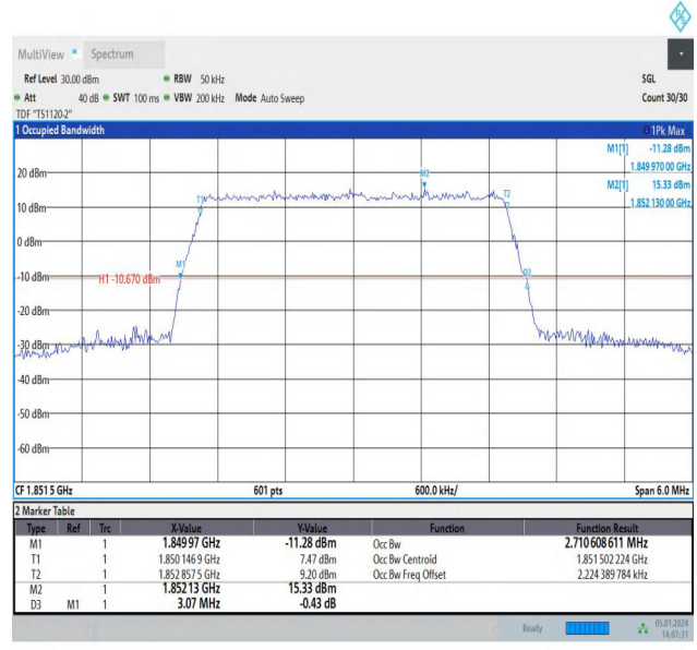
Band2-3MHz-16QAM-18615-15RB#0-PASS
