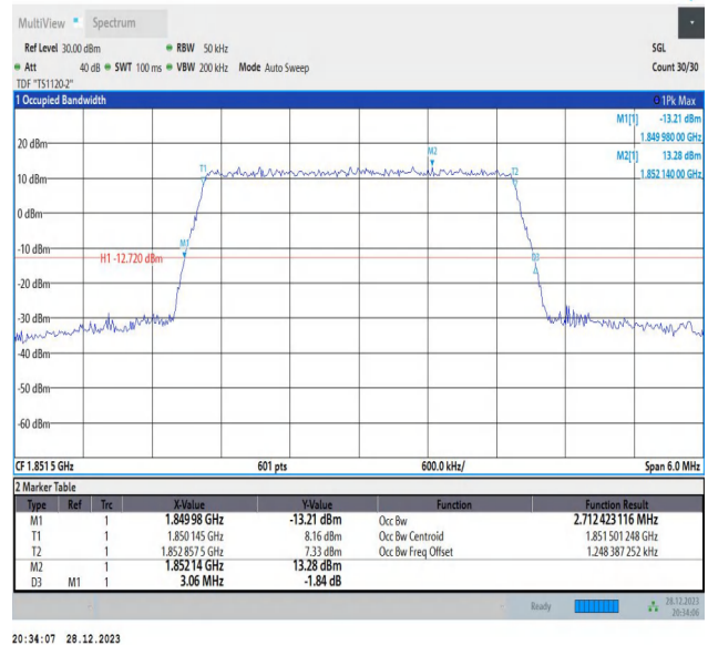
Band2-3MHz-64QAM-18615-15RB#0-PASS
