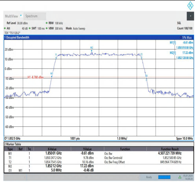
Band2-5MHz-16QAM-18625-25RB#0-PASS
