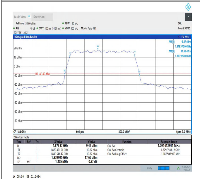
Band2-1.4MHz-QPSK-18900-6RB#0-PASS
