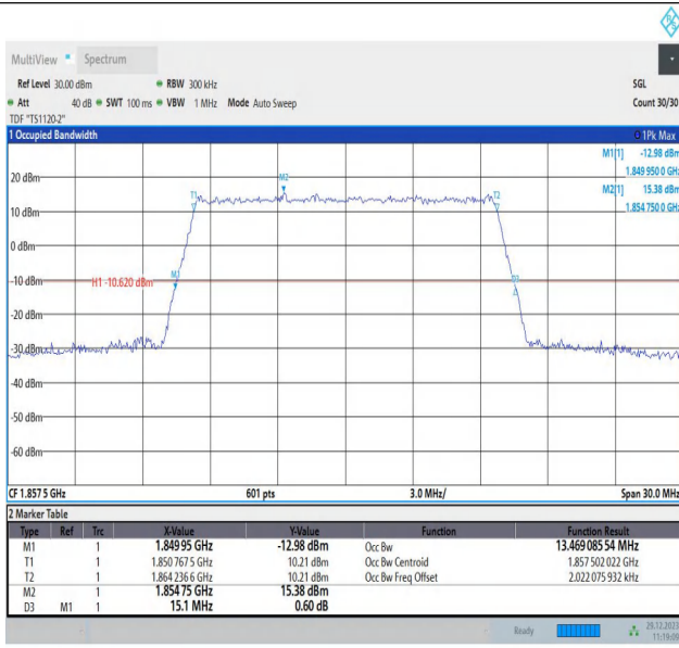
Band2-15MHz-64QAM-18675-75RB#0-PASS
