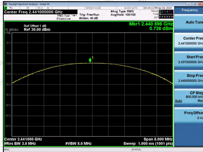
2DH5-Ant1-2441-PASS
