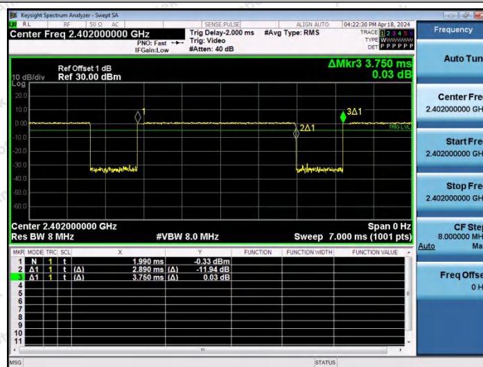
NTVN-3DH5-Ant1-2402
