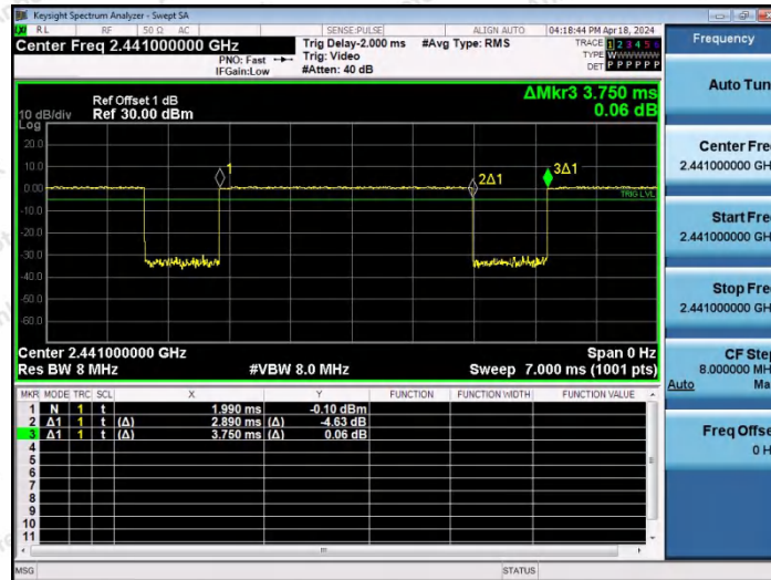
NTVN-2DH5-Ant1-2441
