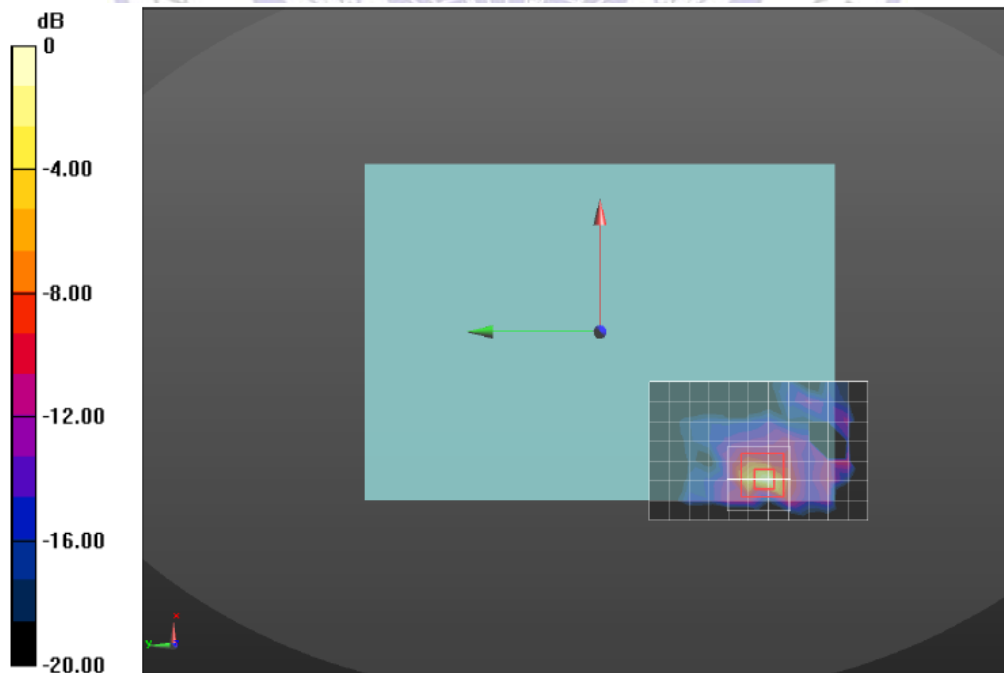
Figure 9: WLAN 802.11a U-NII 3 _ Rear side_0mm
