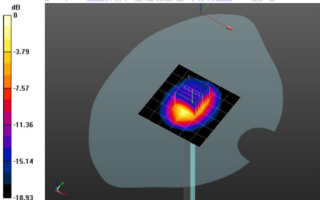
System Performance Check 1900MHz Body 250mW
