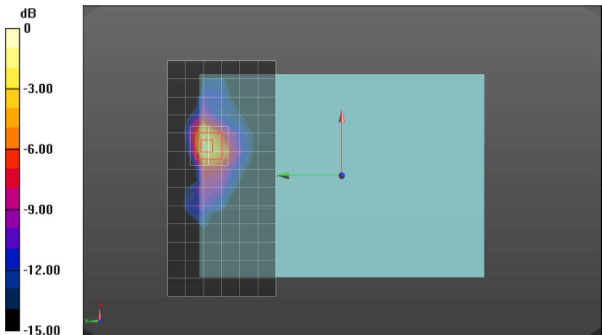
Figure 6: LTE Band 12_QPSK _Rear side_0mm_ Middle Channel
