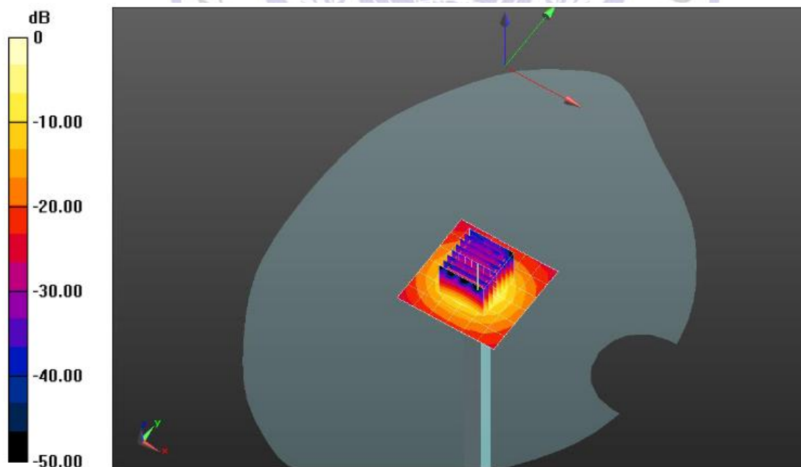
System Performance Check 5200MHz Body 100mW
