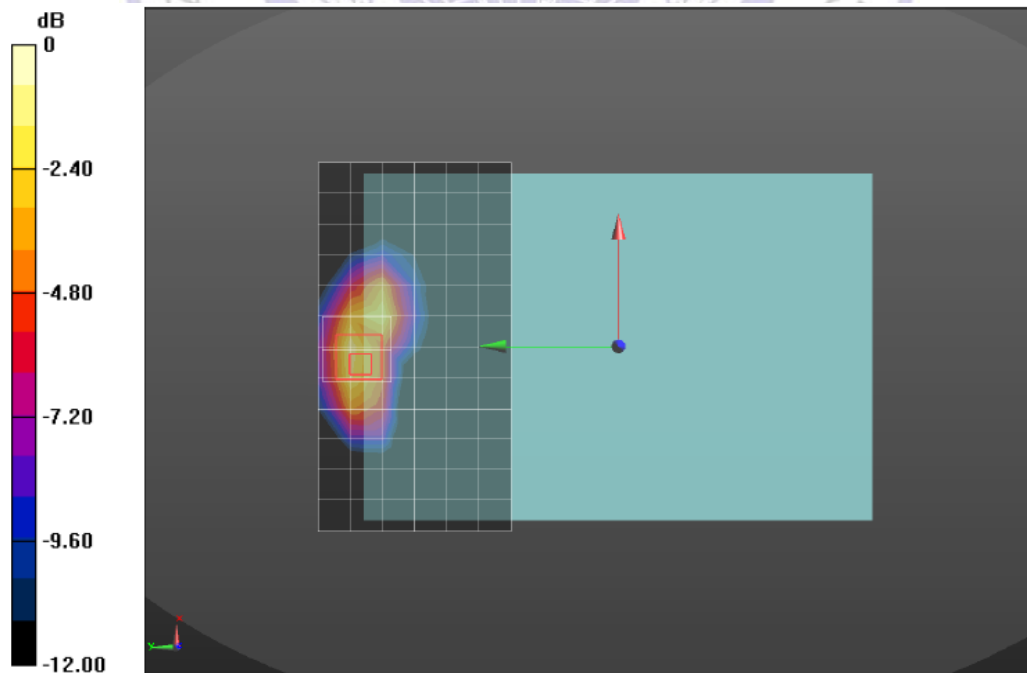
Figure 5: LTE Band 5_QPSK _ Rear side_0mm_ Middle Channel
