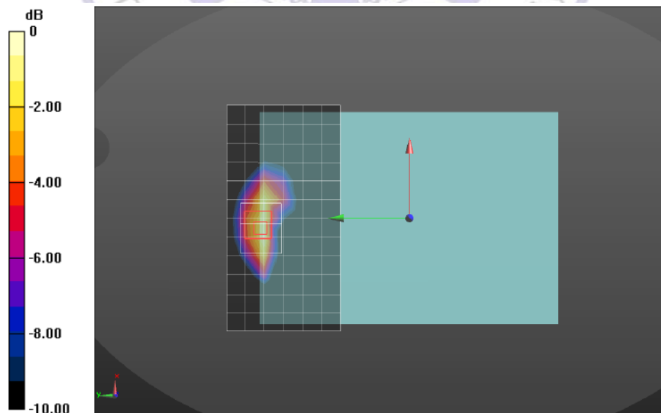
Figure 1: WCDMA Band V_RCM _ Rear side_0mm_Middle Channel
