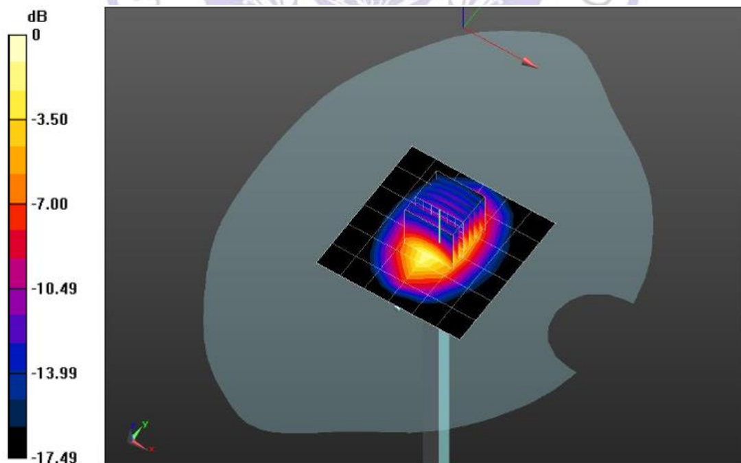
System Performance Check 1750MHz Body 250mW
