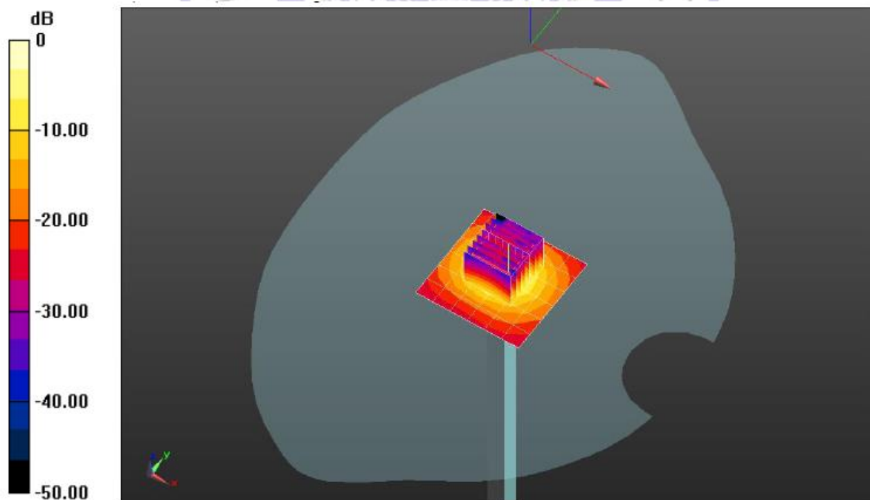
System Performance Check 5800MHz Body 100mW
