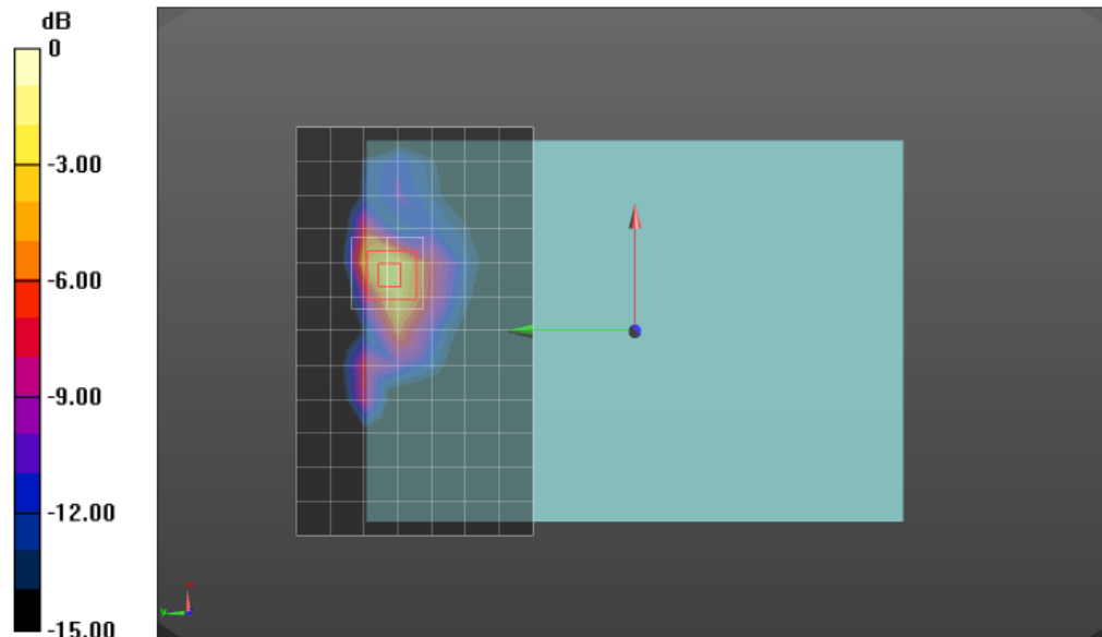
Figure 2: WCDMA Band II_RCM _ Rear side_0mm_Middle Channel
