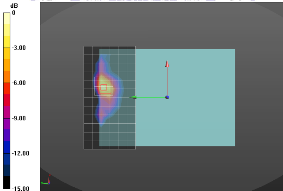
Figure 3: LTE Band 2_QPSK _ Rear side_0mm_ Middle Channel
