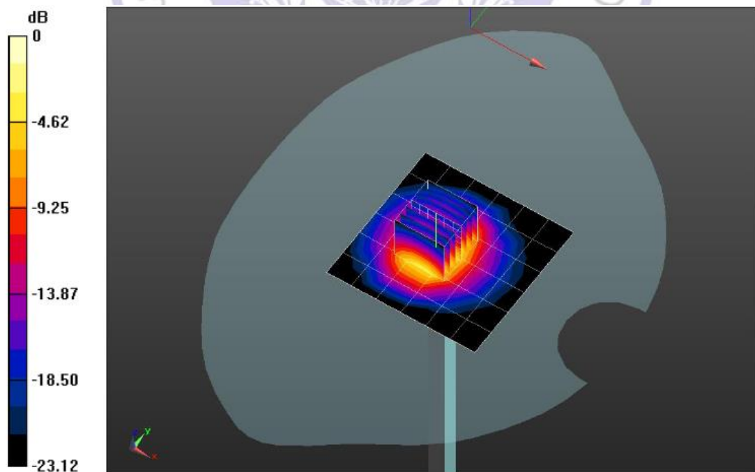
System Performance Check 2450MHz Body 250mW
