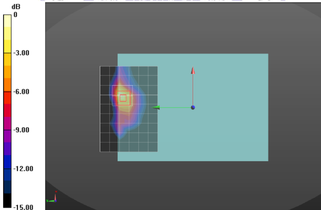
Figure 4: LTE Band 4_QPSK _ Rear side_0mm_ Middle Channel
