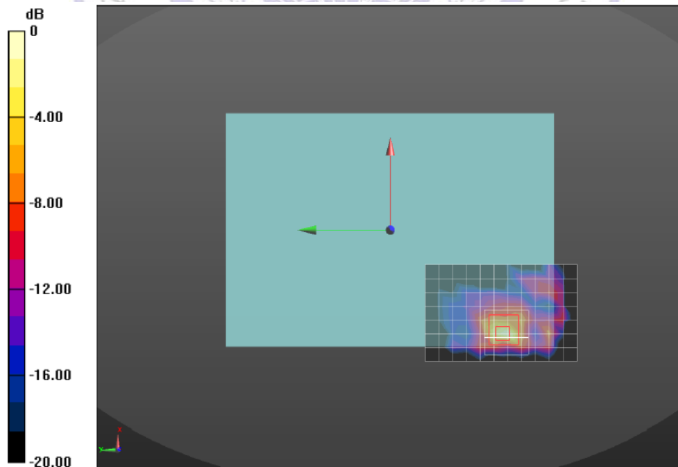
Figure 8: WLAN 802.11a U-NII 1 _ Rear side_0mm
