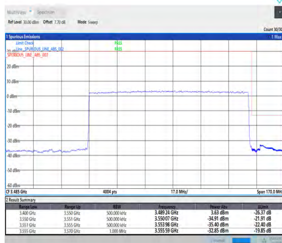
1-N78-3450-3550-PC2-30-100-H-3-DFT-PI2BPSK-Outer_Full-270@0-Ant1-PASS-see graph
