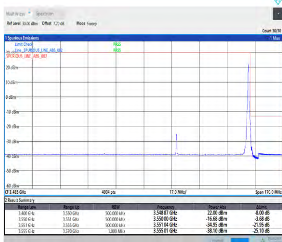
1-N78-3450-3550-PC2-30-90-H-5-CP-QPSK-Edge_1RB_Right-1@244-Ant1-PASS-see graph
