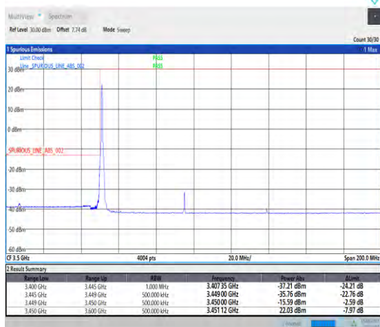
1-N78-3450-3550-PC2-30-90-L-1-DFT-PI2BPSK-Edge_1RB_Left-1@0-Ant1-PASS-see graph
