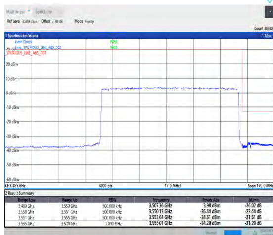
1-N78-3450-3550-PC2-30-90-H-3-DFT-PI2BPSK-Outer_Full-240@0-Ant1-PASS-see graph
