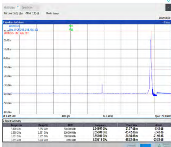
1-N78-3450-3550-PC2-30-100-H-2-DFT-PI2BPSK-Edge_1RB_Right-1@272-Ant1-PASS-see graph
