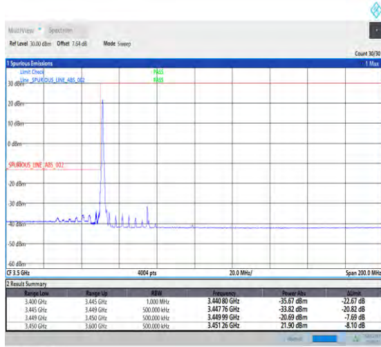
1-N78-3450-3550-PC2-30-50-L-1-DFT-PI2BPSK-Edge_1RB_Left-1@0-Ant1-PASS-see graph
