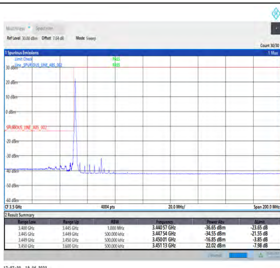
1-N78-3450-3550-PC2-30-40-L-1-DFT-PI2BPSK-Edge_1RB_Left-1@0-Ant1-PASS-see graph
