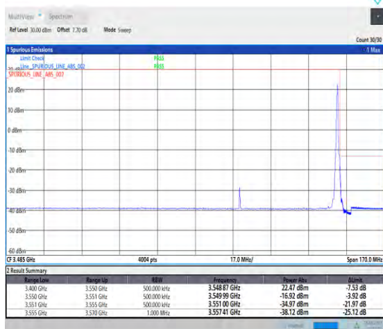
1-N78-3450-3550-PC2-30-90-H-2-DFT-PI2BPSK-Edge_1RB_Right-1@244-Ant1-PASS-see graph
