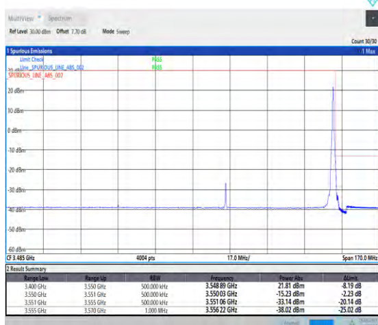
1-N78-3450-3550-PC2-30-100-H-5-CP-QPSK-Edge_1RB_Right-1@272-Ant1-PASS-see graph
