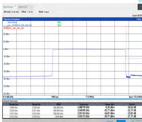
1-N78-3450-3550-PC2-30-90-H-6-CP-QPSK-Outer_Full-245@0-Ant1-PASS-see graph
