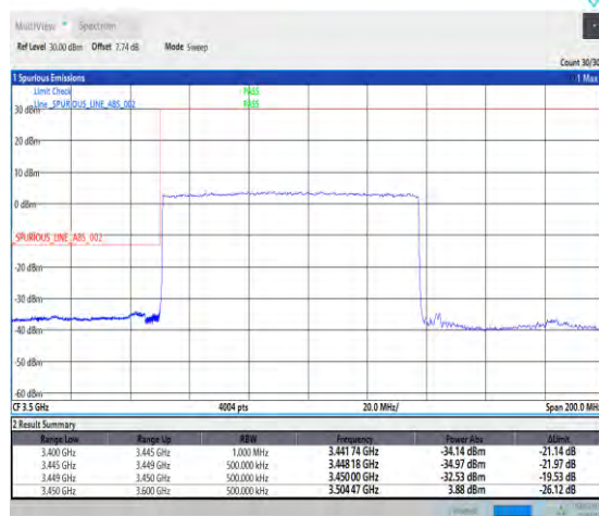
1-N78-3450-3550-PC2-30-90-L-3-DFT-PI2BPSK-Outer_Full-240@0-Ant1-PASS-see graph
