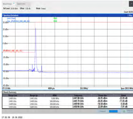
1-N78-3450-3550-PC2-30-20-L-1-DFT-PI2BPSK-Edge_1RB_Left-1@0-Ant1-PASS-see graph
