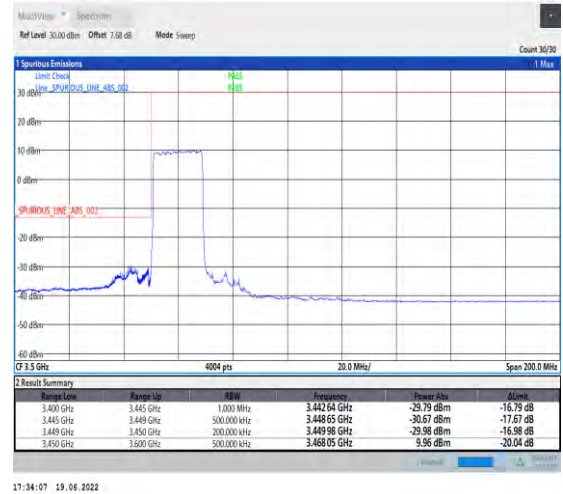
1-N78-3450-3550-PC2-30-20-L-3-DFT-PI2BPSK-Outer_Full-50@0-Ant1-PASS-see graph
