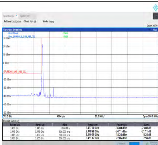
1-N78-3450-3550-PC2-30-30-L-1-DFT-PI2BPSK-Edge_1RB_Left-1@0-Ant1-PASS-see graph
