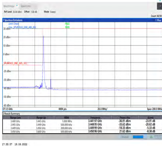
1-N78-3450-3550-PC2-30-20-L-4-CP-QPSK-Edge_1RB_Left-1@0-Ant1-PASS-see graph
