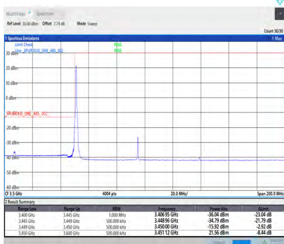
1-N78-3450-3550-PC2-30-90-L-4-CP-QPSK-Edge_1RB_Left-1@0-Ant1-PASS-see graph
