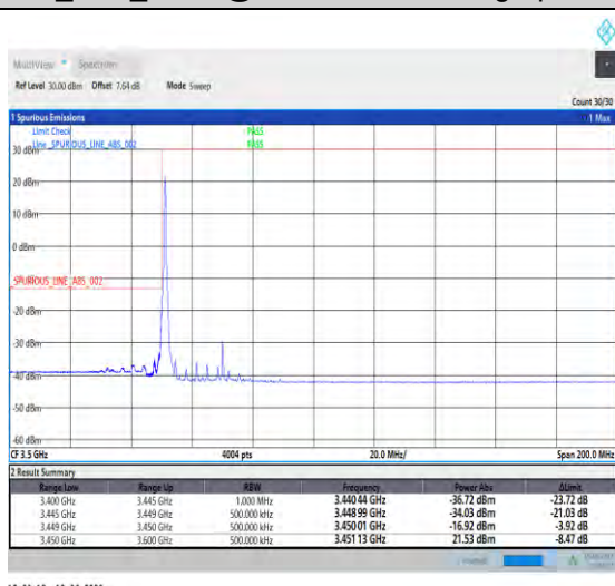
1-N78-3450-3550-PC2-30-40-L-4-CP-QPSK-Edge_1RB_Left-1@0-Ant1-PASS-see graph
