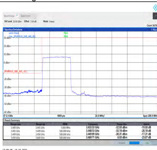
1-N78-3450-3550-PC2-30-40-L-3-DFT-PI2BPSK-Outer_Full-100@0-Ant1-PASS-see graph
