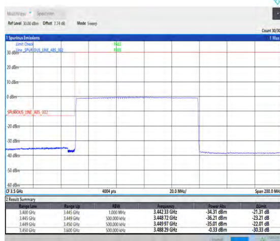
1-N78-3450-3550-PC2-30-90-L-6-CP-QPSK-Outer_Full-245@0-Ant1-PASS-see graph
