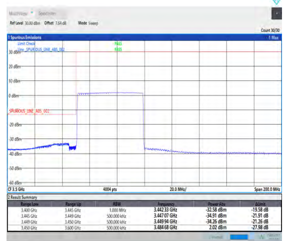
1-N78-3450-3550-PC2-30-50-L-6-CP-QPSK-Outer_Full-133@0-Ant1-PASS-see graph
