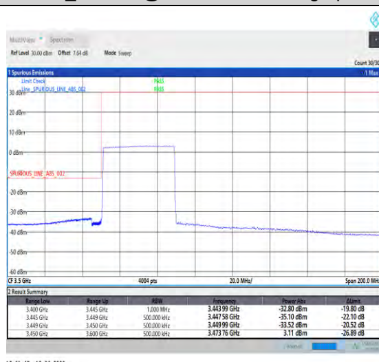
1-N78-3450-3550-PC2-30-40-L-6-CP-QPSK-Outer_Full-106@0-Ant1-PASS-see graph
