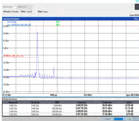
1-N78-3450-3550-PC2-30-50-L-4-CP-QPSK-Edge_1RB_Left-1@0-Ant1-PASS-see graph
