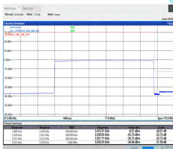
1-N78-3450-3550-PC2-30-100-H-6-CP-QPSK-Outer_Full-273@0-Ant1-PASS-see graph
