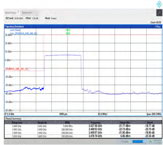
1-N78-3450-3550-PC2-30-50-L-3-DFT-PI2BPSK-Outer_Full-128@0-Ant1-PASS-see graph
