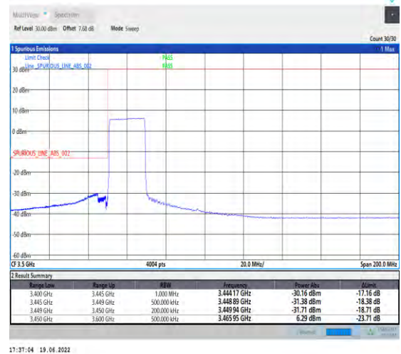
1-N78-3450-3550-PC2-30-20-L-6-CP-QPSK-Outer_Full-51@0-Ant1-PASS-see graph
