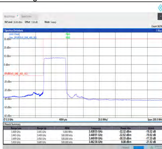
1-N78-3450-3550-PC2-30-30-L-3-DFT-PI2BPSK-Outer_Full-75@0-Ant1-PASS-see graph
