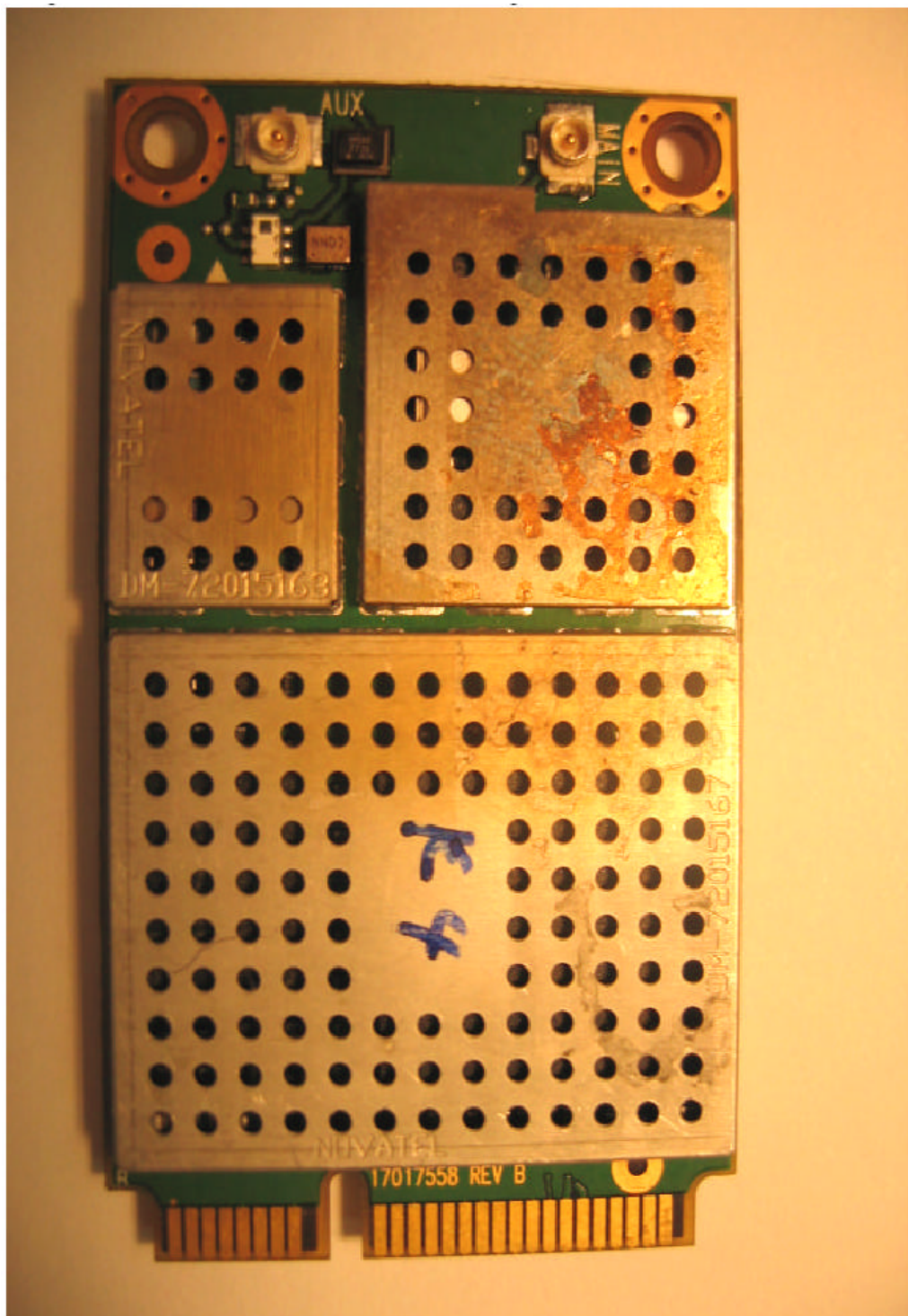
Top Side With Shields – Mini Express Card
