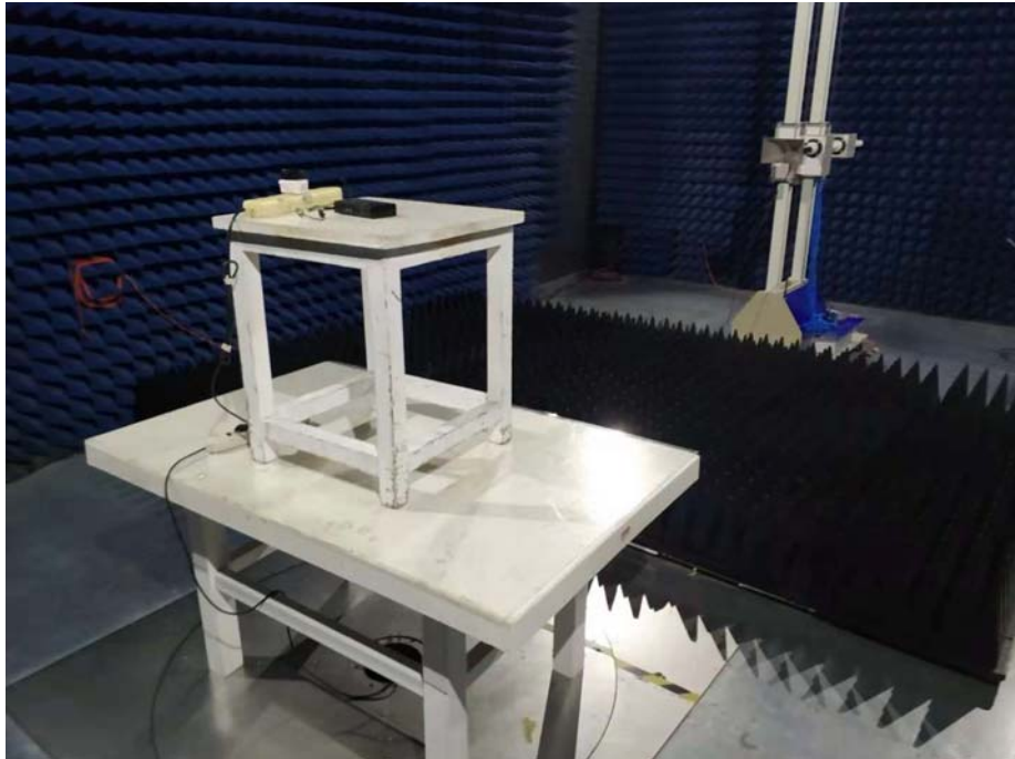
Photograph – Conducted Emission Test Setup Photos
