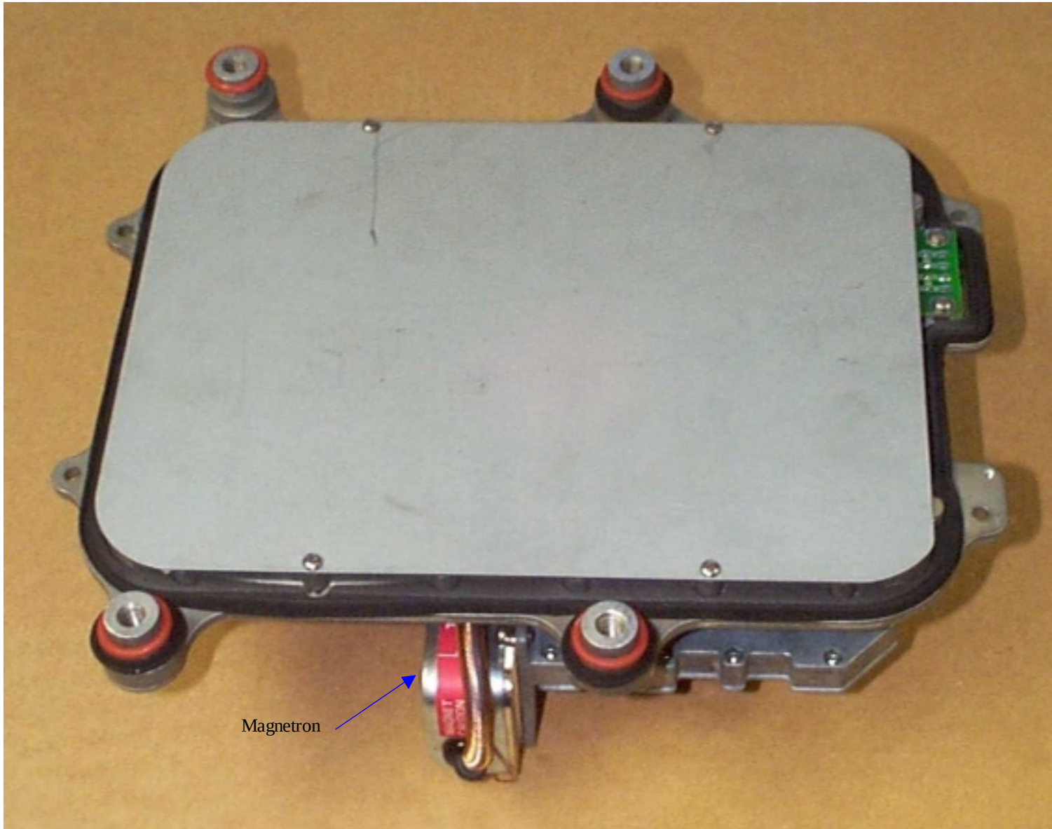
2D - 2kW, 18" Radome Scanner Unit
