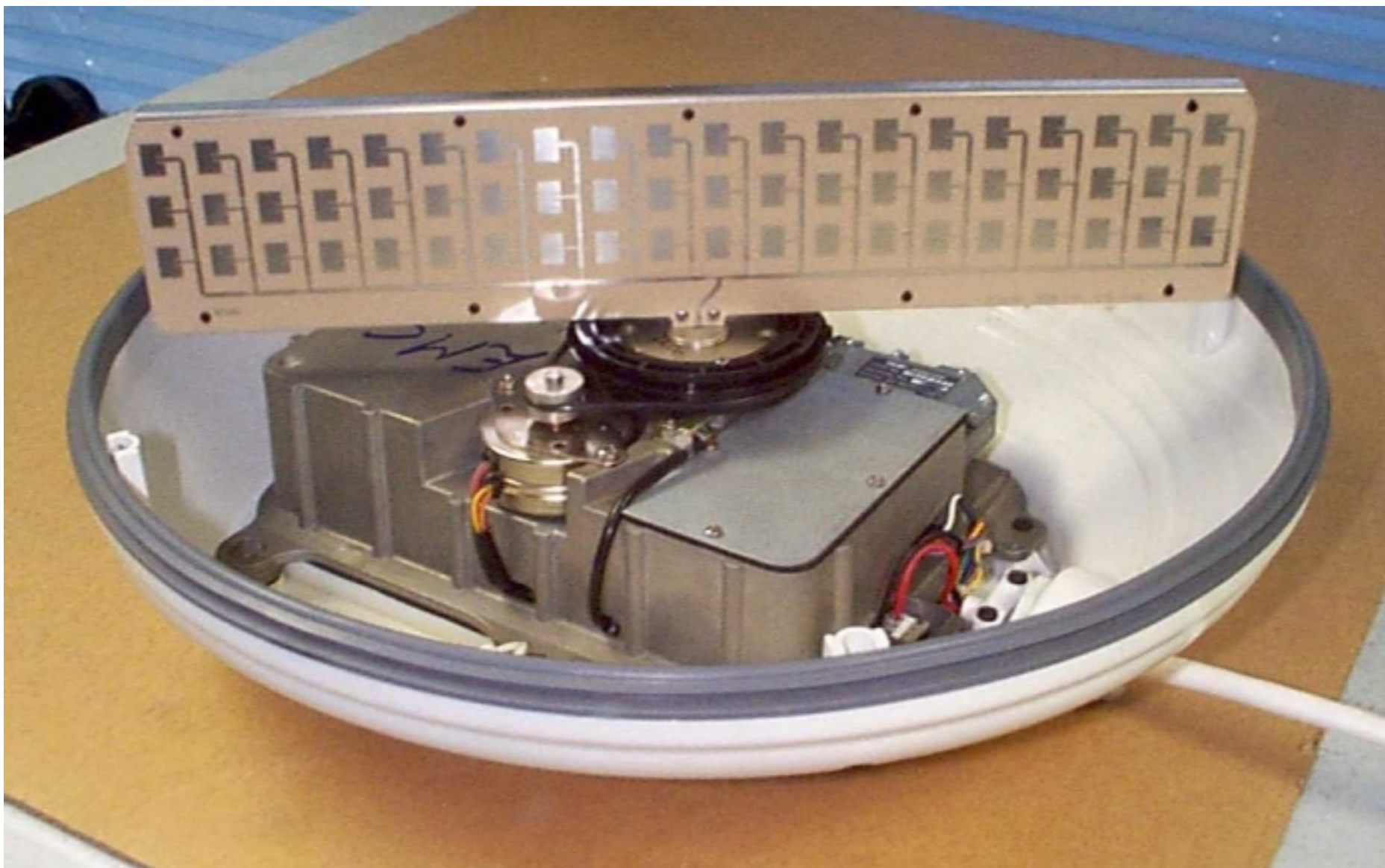
2D – 2kW, 18" Radome Scanner Unit
