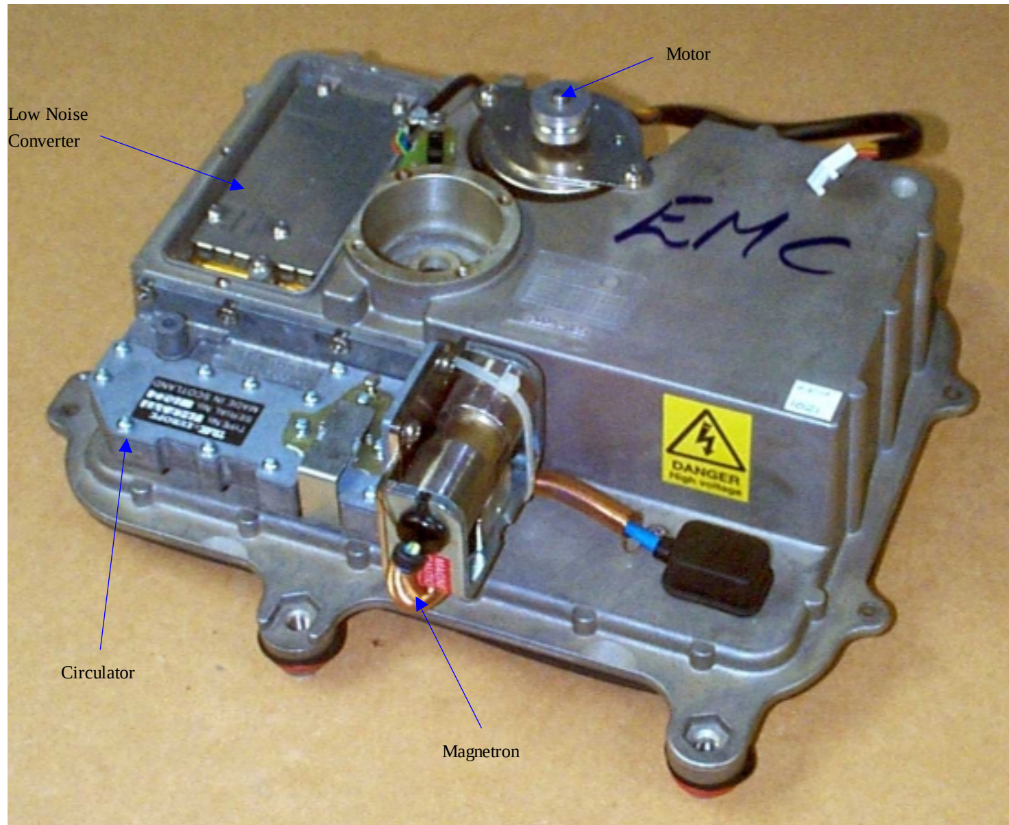
2D – 2kW, 18" Radome Scanner Unit
