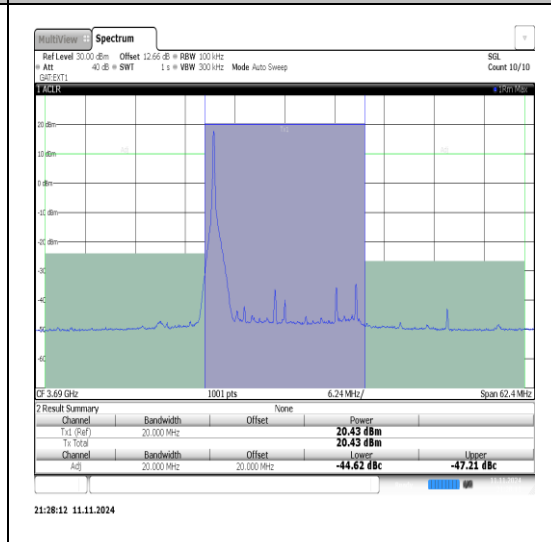
Band48-20MHz-16QAM-56640-1RB#99-PASS
