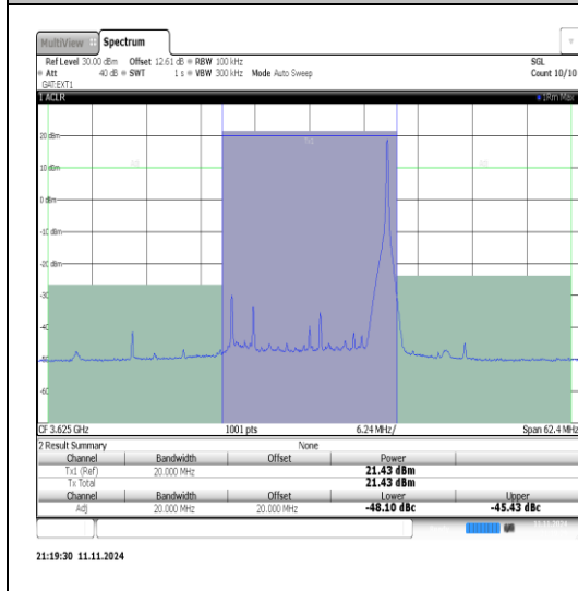
Band48-20MHz-16QAM-56640-100RB#0-PASS
