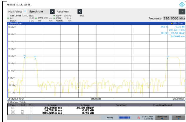
CONFIGURATION 1 (326.5kHz)
