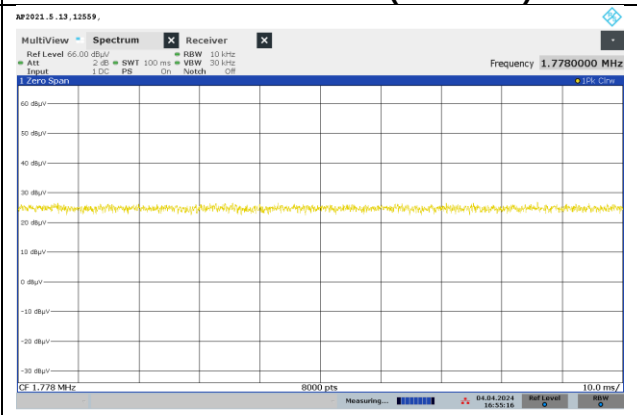
CONFIGURATION 6 (1.778MHz)
