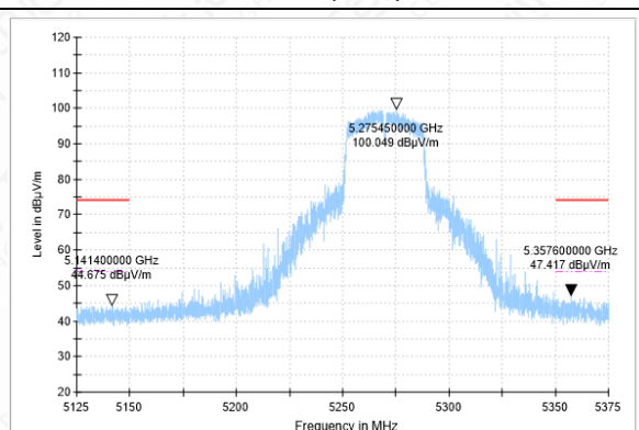
BANDEGE-11N(40M)-CH54-PK
