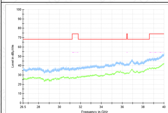
RSE-11N-CH36-26.5GHz-40GHz
