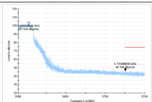
BANDEGE-11AC-CH120-PK
