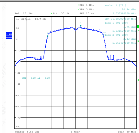
11N40SISO-Ant1-5550
