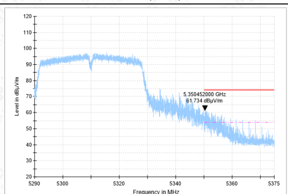
BANDEGE-11N(40M)-CH62-PK
