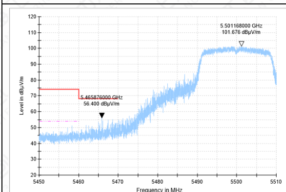
BANDEGE-11AC-CH100-PK
