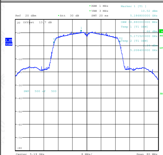
11N40SISO-Ant1-5190
