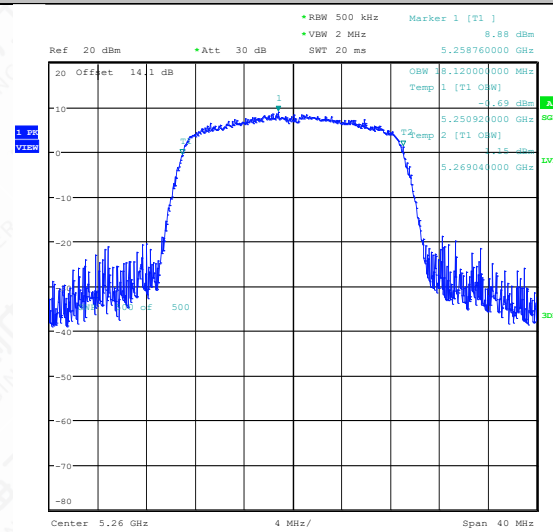
11AC20SISO-Ant1-5260
