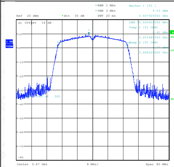
11AC40SISO-Ant1-5670
