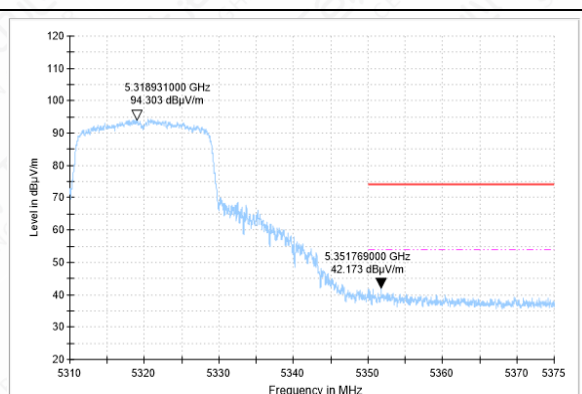
BANEDGE-11N-CH64-AV
