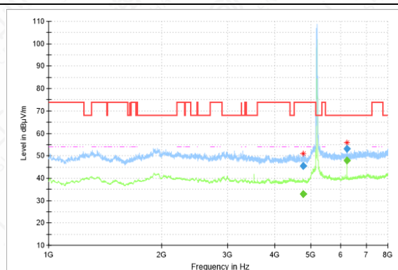
RSE-11N-CH36-1GHz-8GHz
