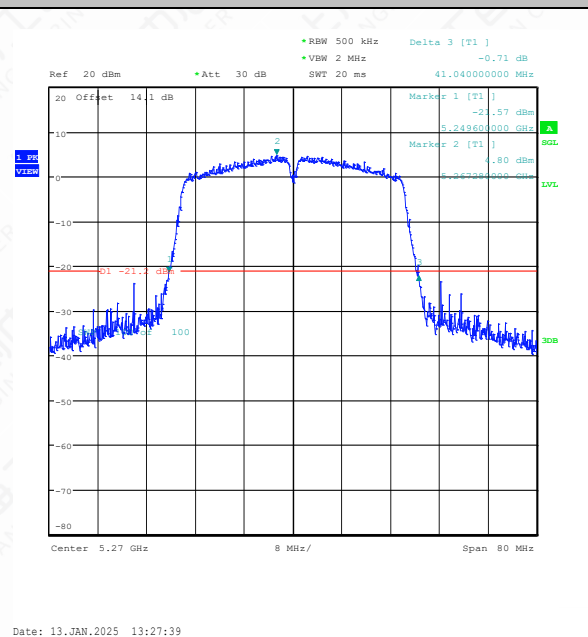
11AC40SISO-Ant1-5270
