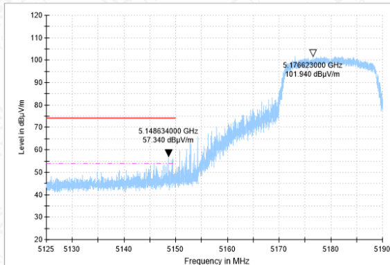
BANEDGE-11N-CH36-PK
