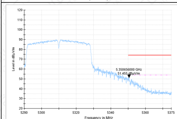
BANDEGE-11N(40M)-CH62-AV-17
