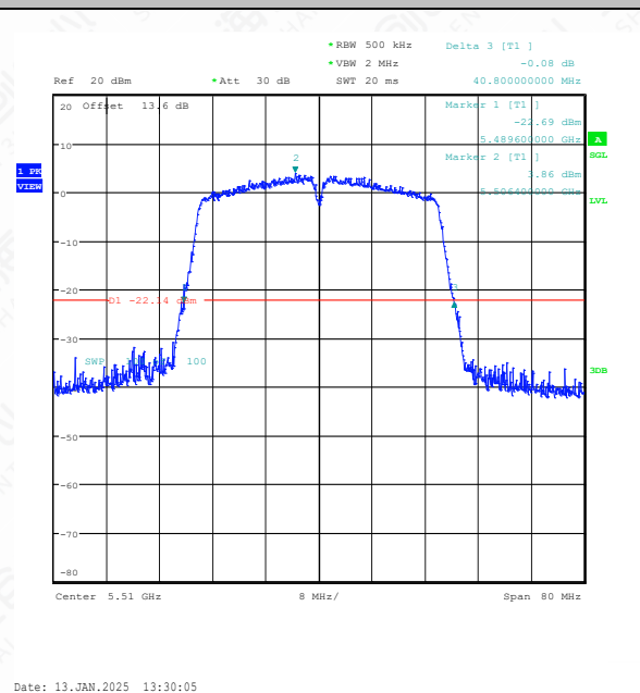
11AC40SISO-Ant1-5510
