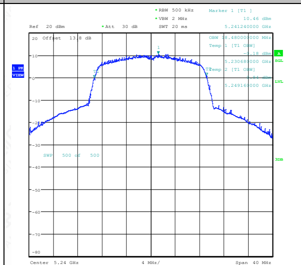
11N20SISO-Ant1-5240
