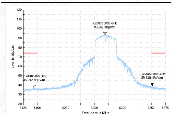
BANDEGE-11N(40M)-CH54-AV
