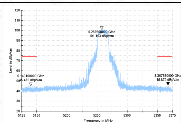
BANEDGE-11N-CH52-PK
