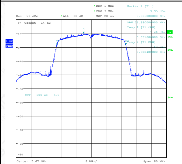
11N40SISO-Ant1-5670
