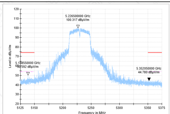
BANDEGE-11N(40M)-CH46-PK
