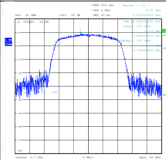
11AC20SISO-Ant1-5700
