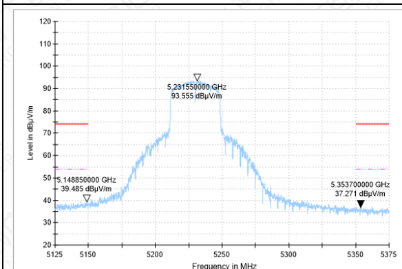
BANDEGE-11N(40M)-CH46-AV
