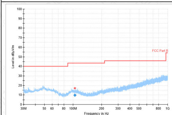
RSE-11N-CH36-30MHz-1GHz
