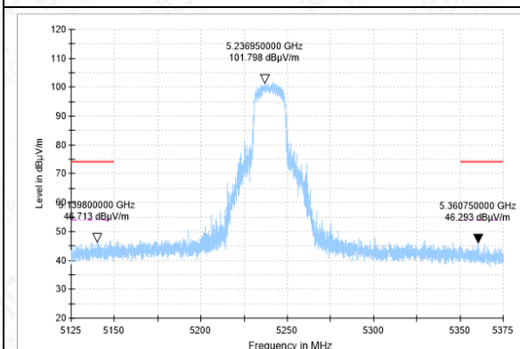
BANEDGE-11N-CH48-PK
