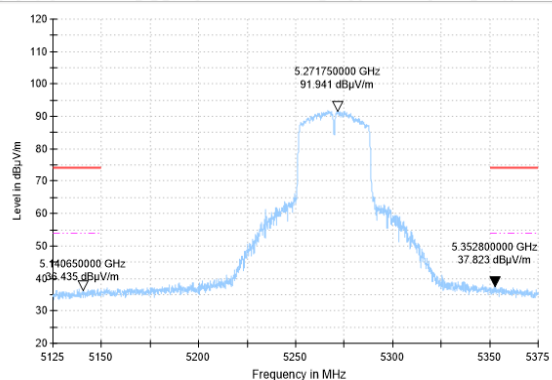
BANEDGE-11AC(40M)-CH54-AV
