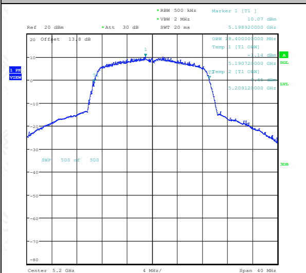
11N20SISO-Ant1-5200
