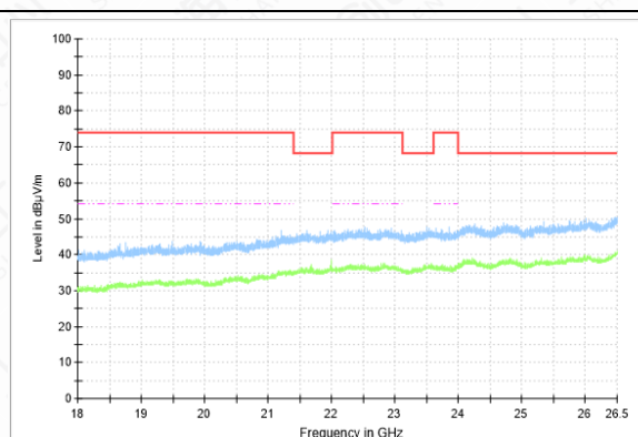
RSE-11A-CH140-18GHz-26.5GHz
