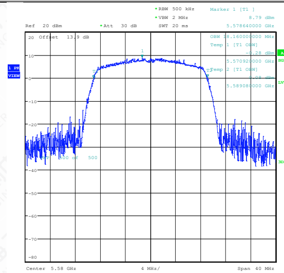
11AC20SISO-Ant1-5580
