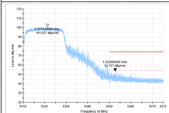
BANDEGE-11AC-CH64-PK
