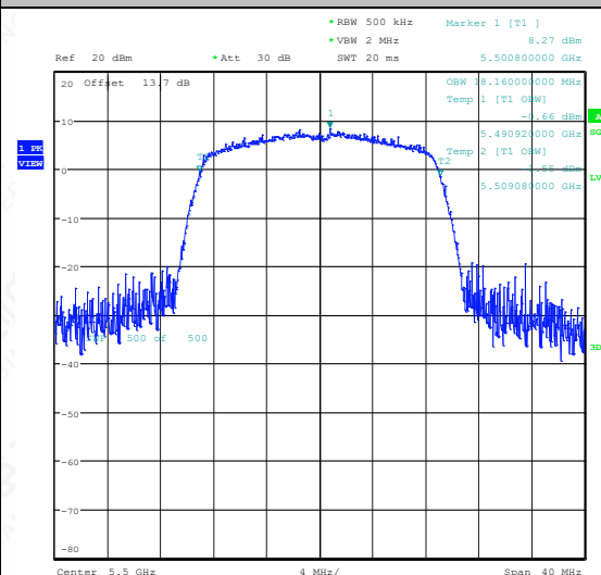
11AC20SISO-Ant1-5500
