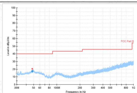
RSE-11N-CH56-30MHz-1GHz
