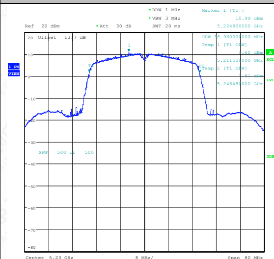
11N40SISO-Ant1-5230
