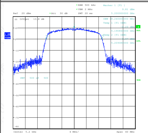
11AC20SISO-Ant1-5200
