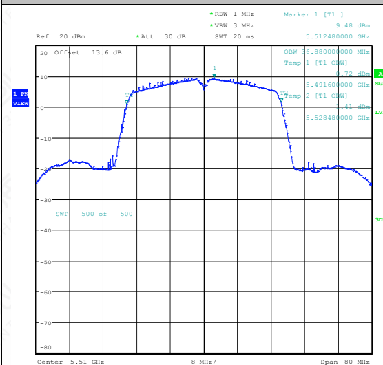
11N40SISO-Ant1-5510
