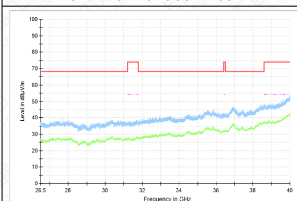
RSE-11A-CH140-26.5GHz-40GHz
