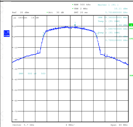
11N20SISO-Ant1-5700
