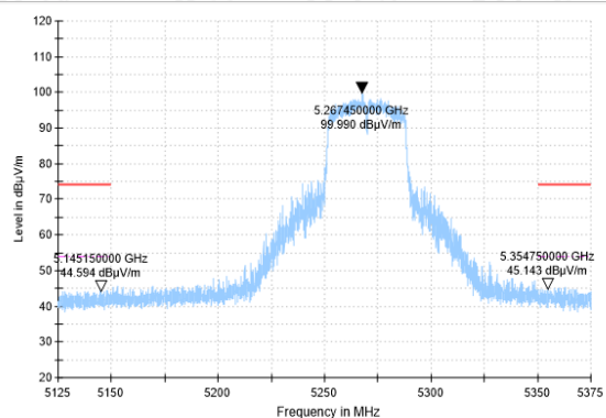
BANEDGE-11AC(40M)-CH54-PK
