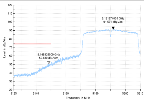
BANDEGE-11N(40M)-CH38-AV-16
