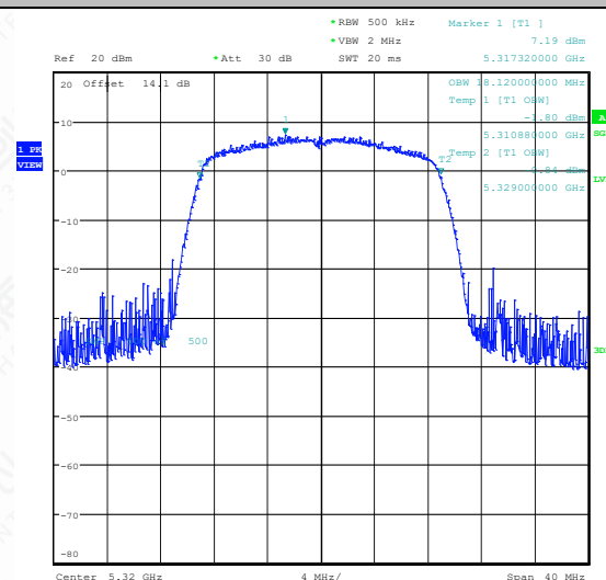
11AC20SISO-Ant1-5320
