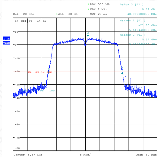
11AC40SISO-Ant1-5670
