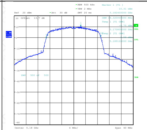
11N20SISO-Ant1-5180
