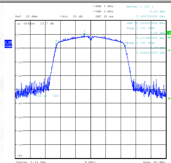
11AC40SISO-Ant1-5190
