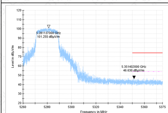
BANEDGE-11N-CH56-PK
