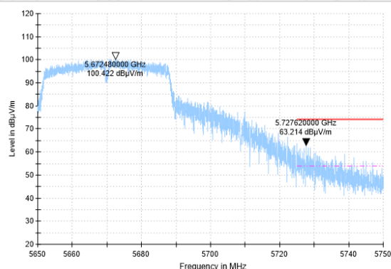
BANDEGE-11N(40M)-CH134-PK
