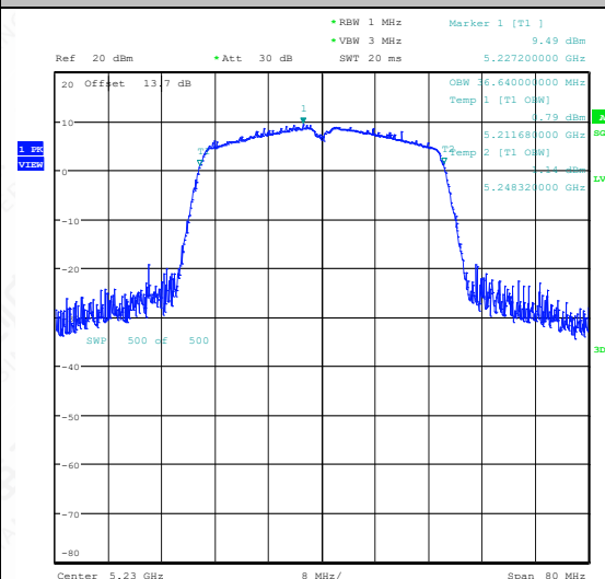
11AC40SISO-Ant1-5230
