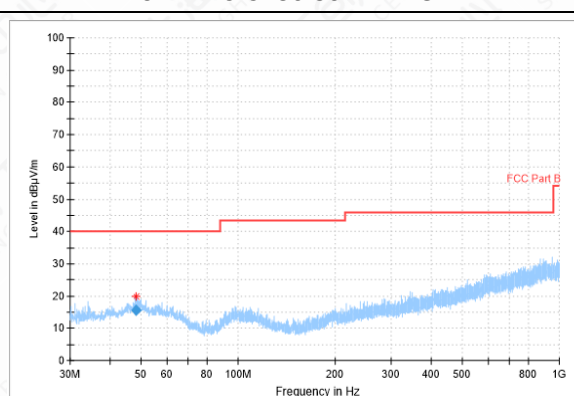
RSE-11AC-CH36-30MHz-1GHz
