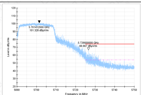
BANDEGE-11AC-CH140-PK
