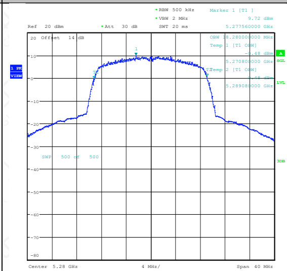
11N20SISO-Ant1-5280
