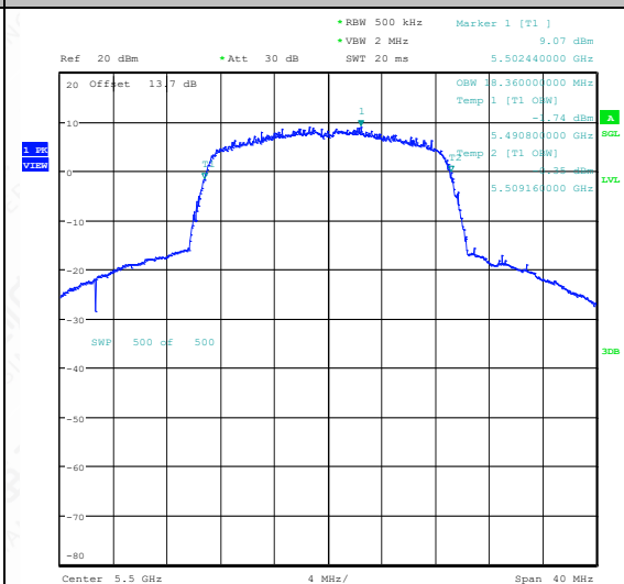
11N20SISO-Ant1-5500
