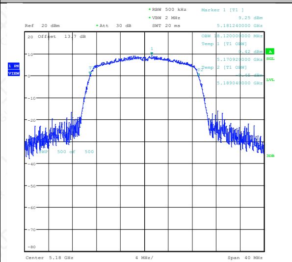
11AC20SISO-Ant1-5180
