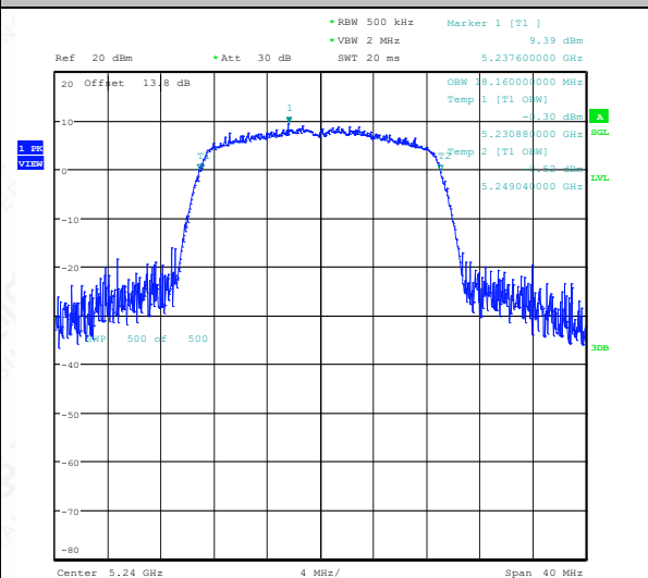
11AC20SISO-Ant1-5240
