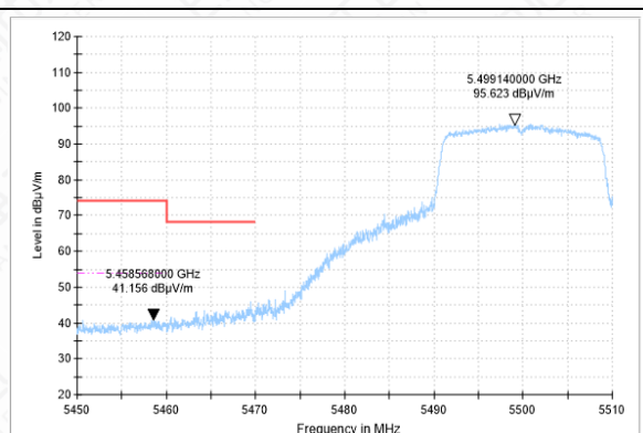
BANEDGE-11N-CH100-AV
