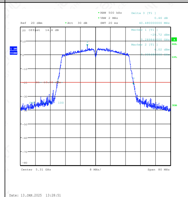
11AC40SISO-Ant1-5310
