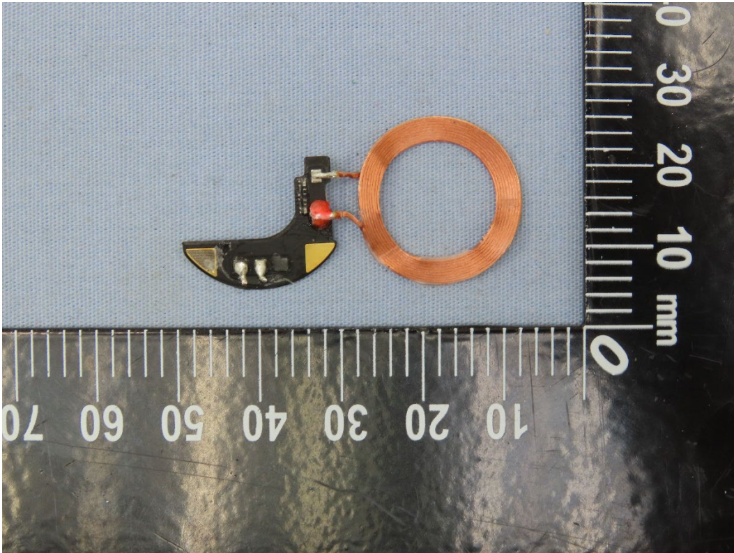
Apple Watch Coil and PCBA (326.5kHz / 1.778MHz)
