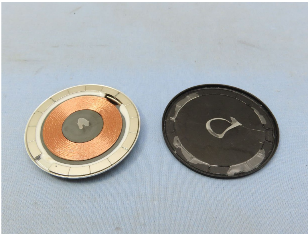
Qi2 MPP/BPP Coil and PCBA (127.7kHz, 360kHz)
