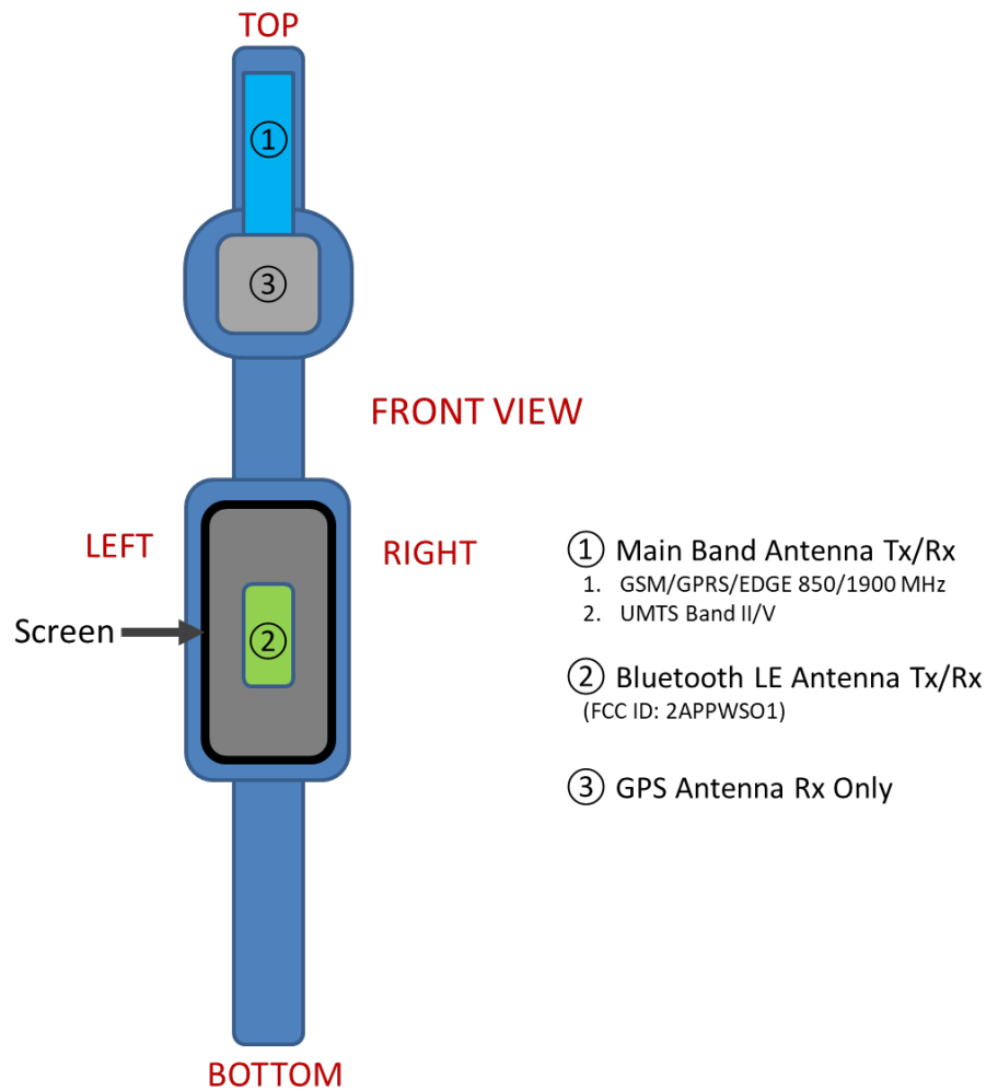
Figure F-1 DUT Antenna Locations
